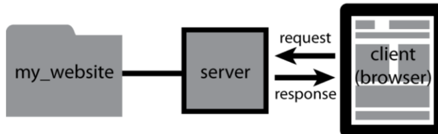
Figure 2.3: client-server architecture
