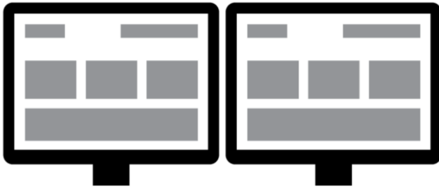
Figure 1.3: normalization demonstration
