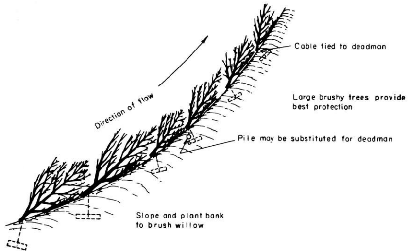
TREE REVETMENT
