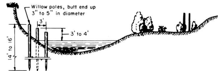
JETTED WILLOW POLES
