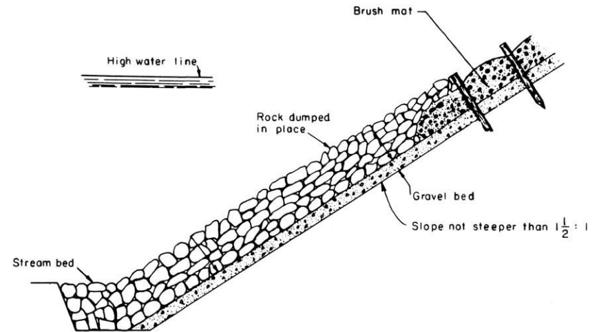
ROCK RIPRAP AND BRUSH MAT
