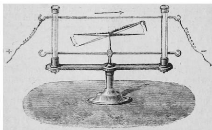
FIG. 1.—Action of an electrical current on the magnetic needle. (Oersted's experiment.)
