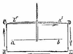
FIG. 7.—System of two magnetic needles, with their poles reversed, forming an astatic combination, neutralising the effects of terrestrial magnetism.
