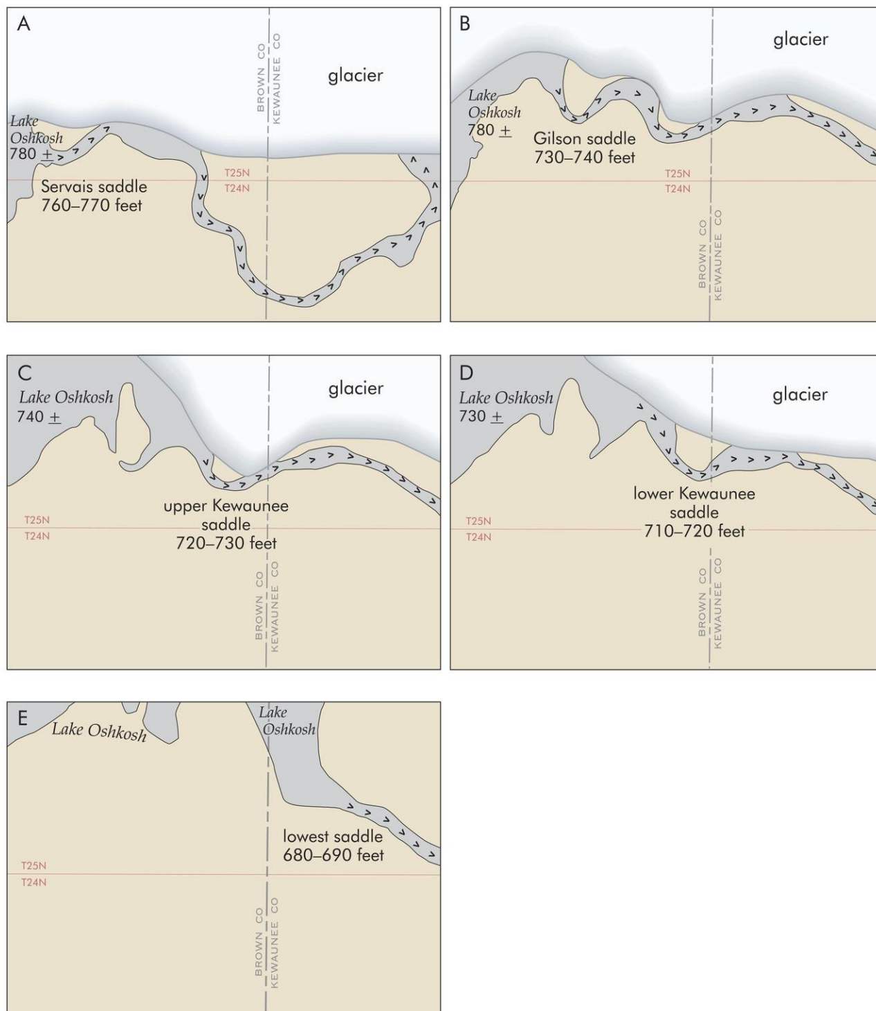
Figure 21. Some stages in the deglaciation of the head of the Kewaunee spillway in northern Kewaunee County and adjacent Brown County.
