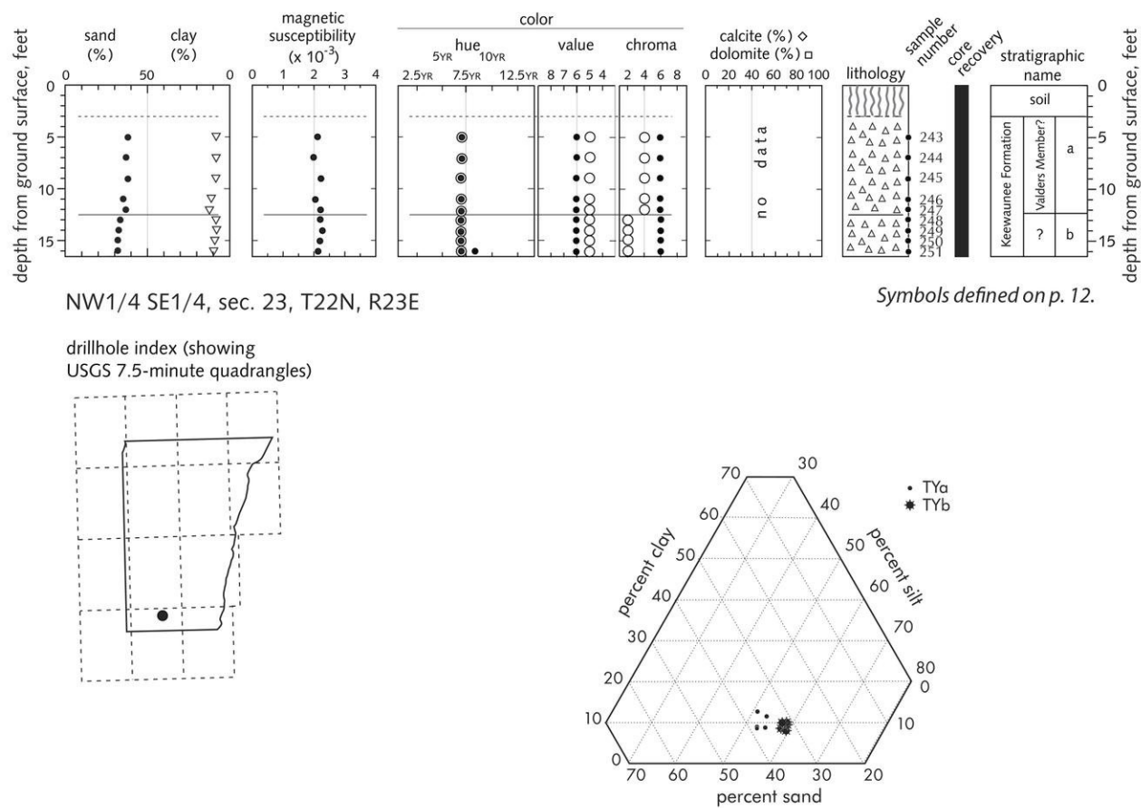
Figure 10I. Sample log for drill hole TY.
