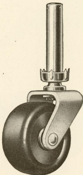
No. C-1 Diamond Velvet with Hard Tread Atlasite (Bakelite) Wheel 1 5/8 inch diameter Used on all chairs shown on pages 52 to 75
