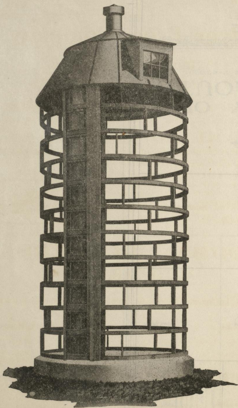
Frame of Rings and Studding Ready for Sheathing
