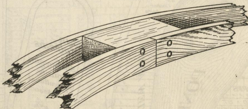
Piece of Double Oak Ring showing Open Air Space thru ring
