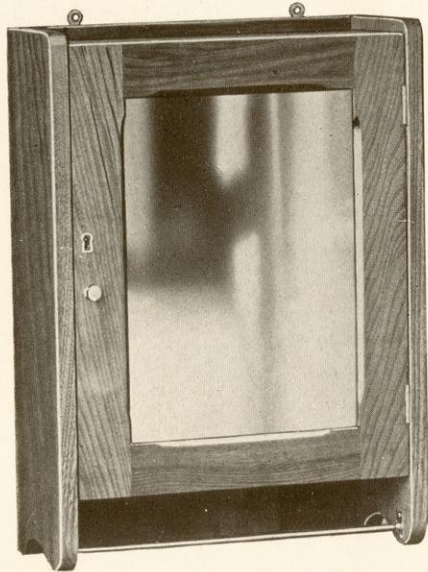
No. 841 TOWEL CABINET Size 15x6 inches. Height 21 inches. Hardwood, Golden Gloss Finish. Plain Plate Mirror 10x14 inches. Compartments for Clean and Soiled Towels. Shelf for Brush, Comb and Soap. Nickel Plated Towel Rod. Weight, one in a carton, 21 pounds.
