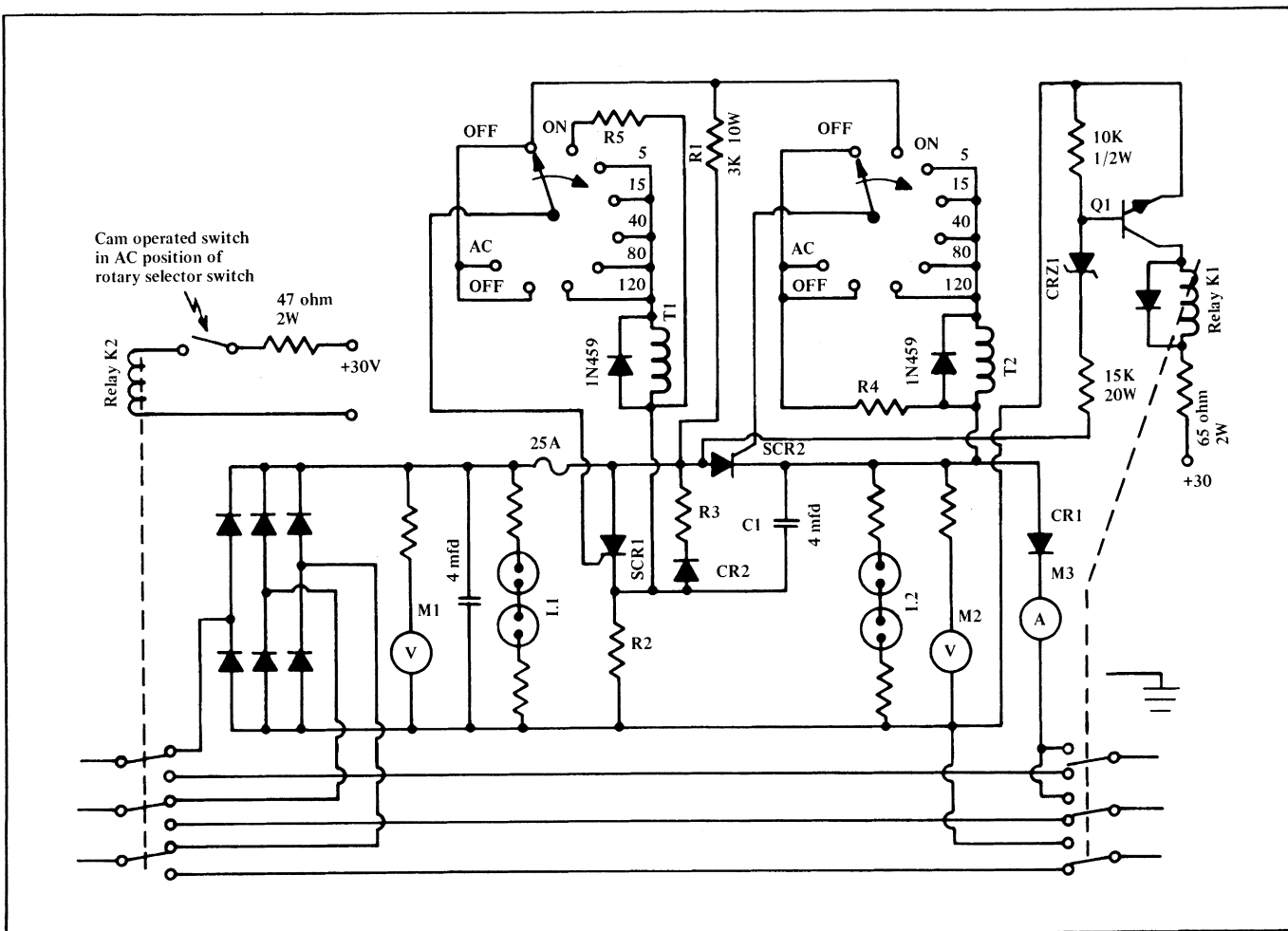
FIGURE 9. Power Control Panel
