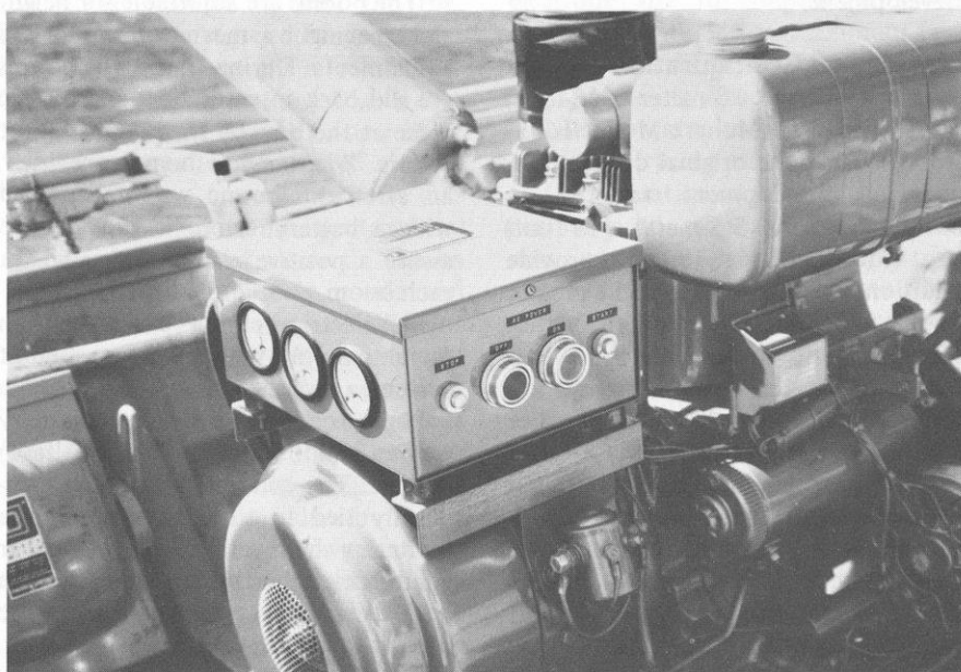
Engine-generator unit with control box mounted on generator. Note 12-volt automotive alternator in lower right corner.
