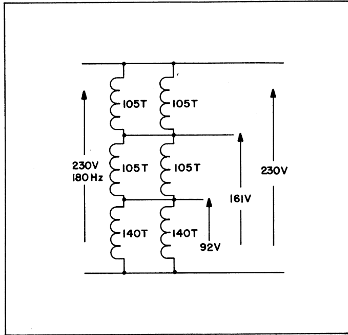
FIGURE 7. Low Voltage Transformer Connection
