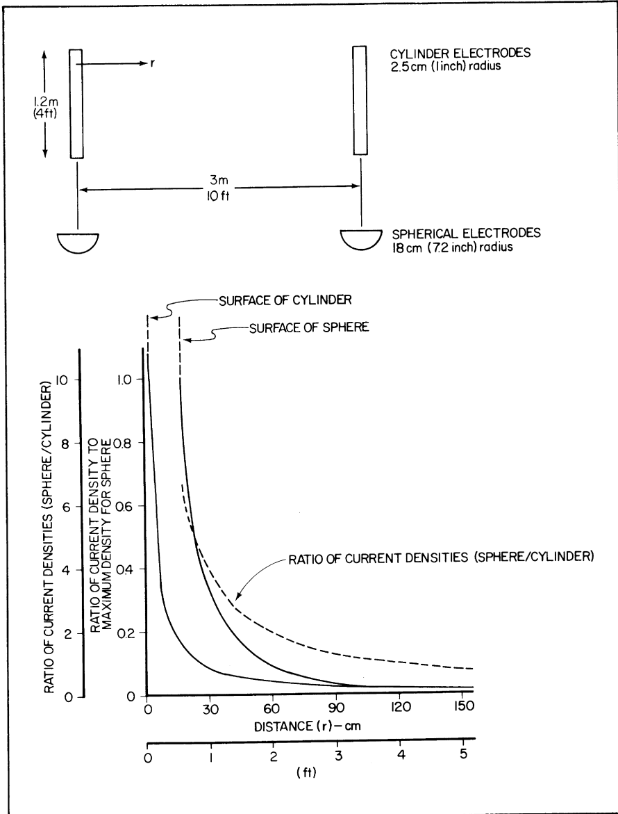
FIGURE 3. Comparison of current distribution of cylindrical and spherical electrodes
