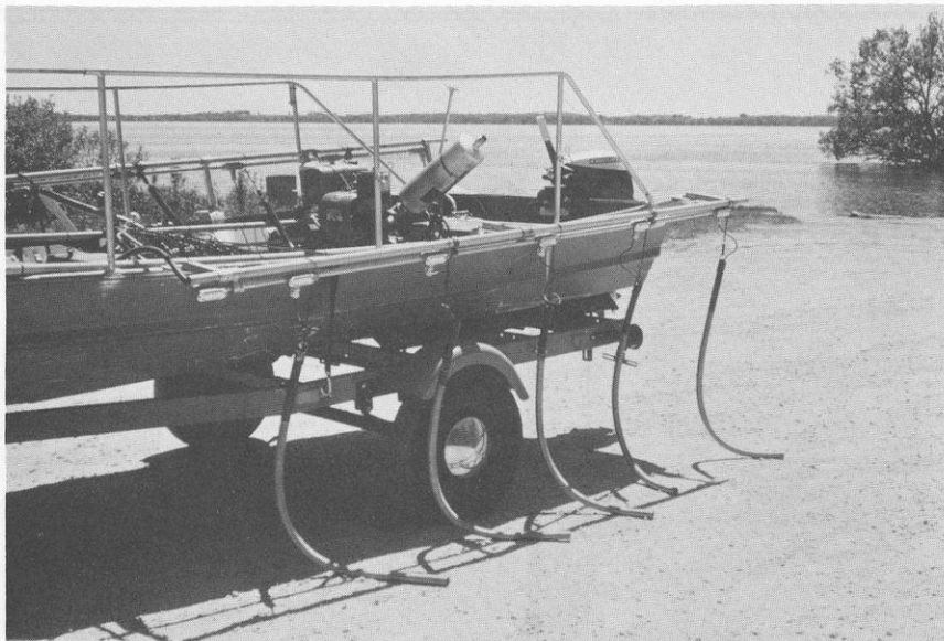
Cathode array—set of ten 1.2 m (4-foot) lengths of 2.5 cm (one-inch) diameter flexible conduit (5 on each side of boat).
