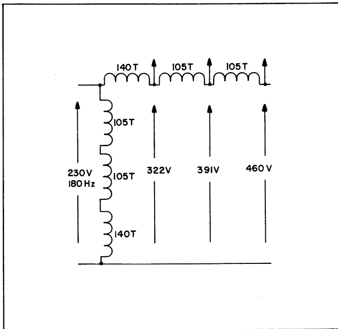
FIGURE 6. High Voltage Transformer Connection
