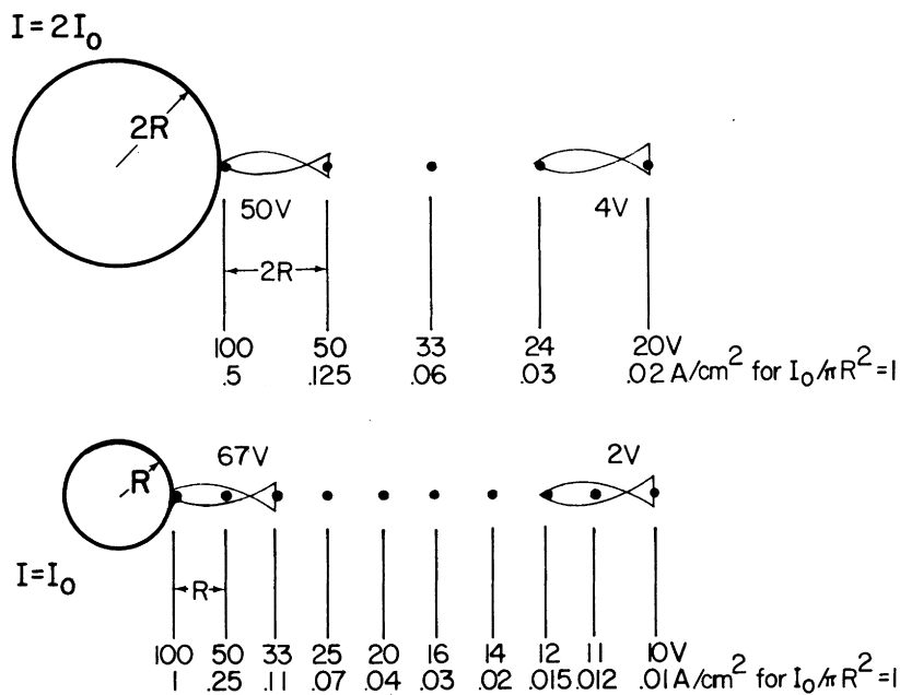
FIGURE 2. Field pattern, voltage and current distributions for spherical electrodes
