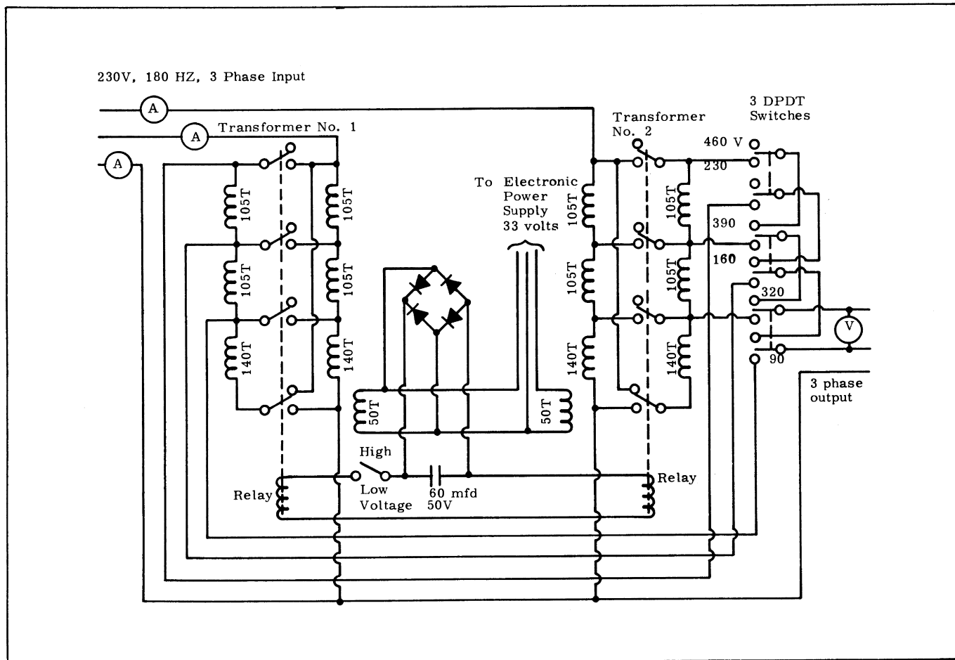
FIGURE 8. Transformer Panel
