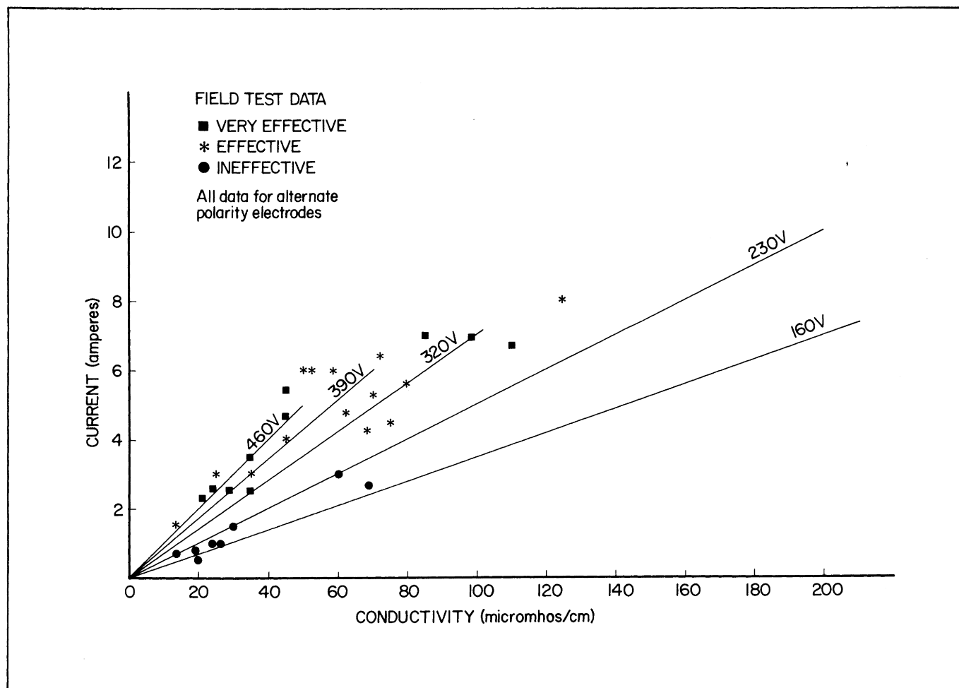
FIGURE 11. Electrofishing performance of ac electrofishing boats.
