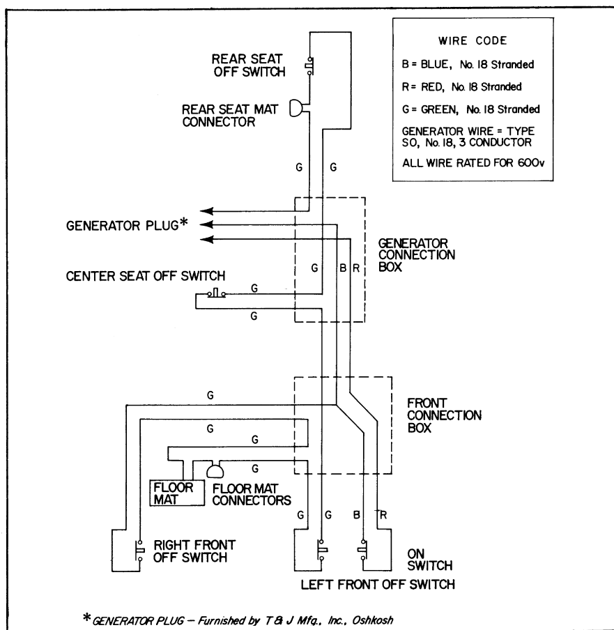
FIGURE 17. Twelve-volt control circuit
