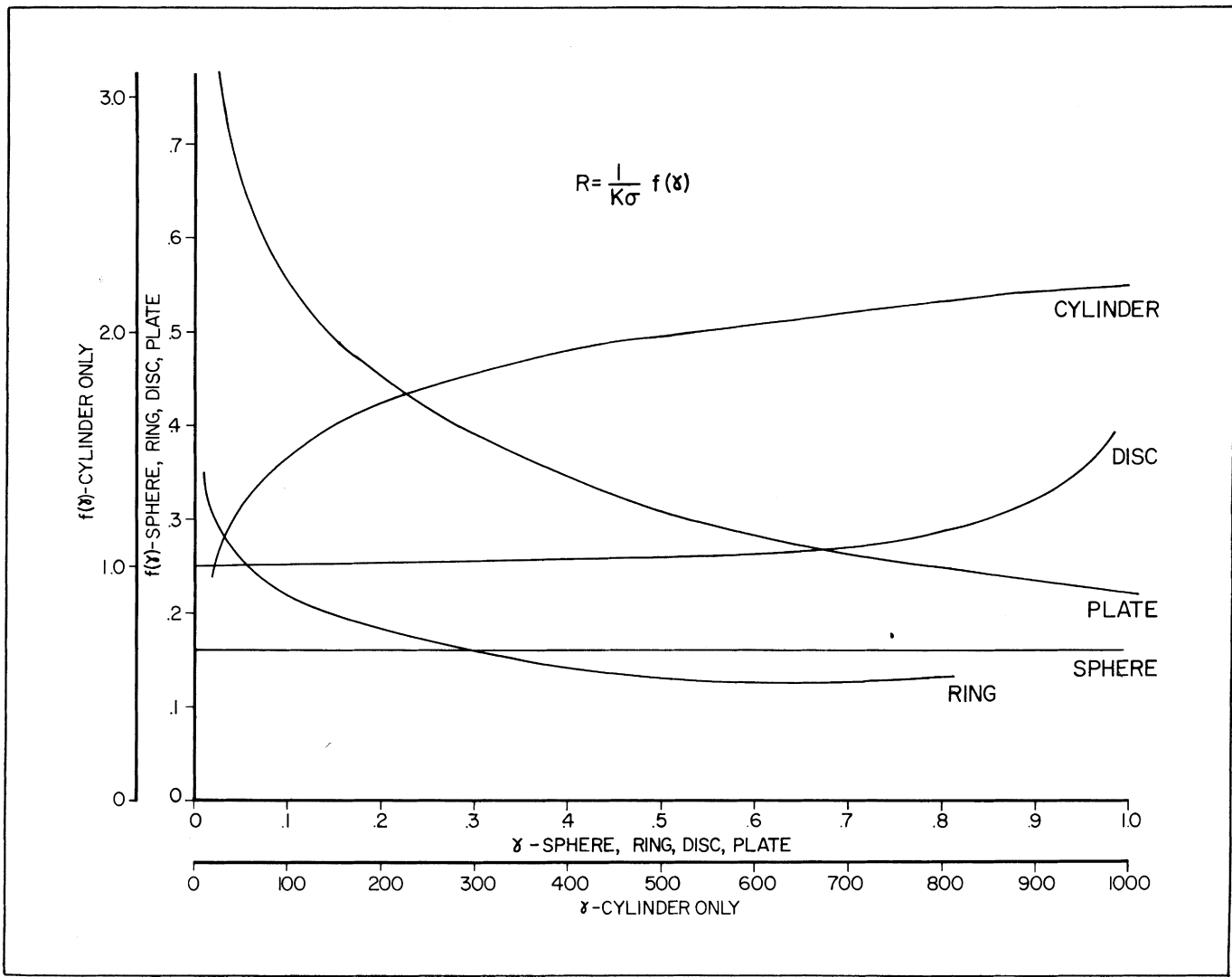
FIGURE 13. Electrode resistance factors
