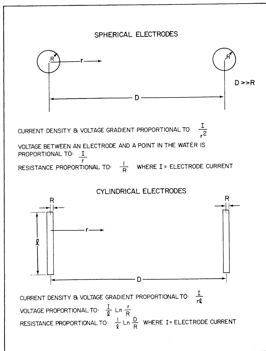
FIGURE 1. Properties of spherical and cylindrical electrodes
