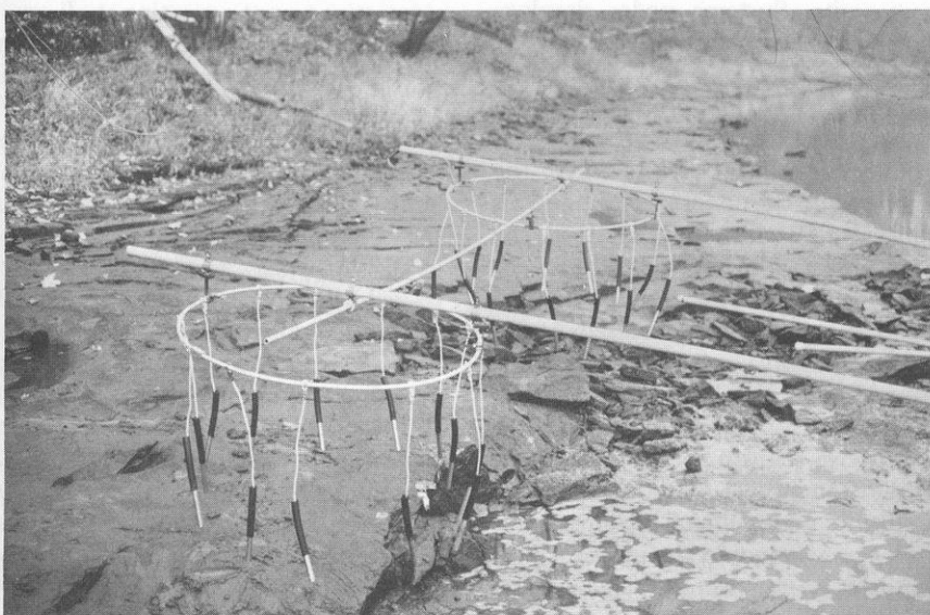
Anode array—two 36-inch [91 cm] aluminum rings with a large number of "dropper" electrodes (Fig. 8).
