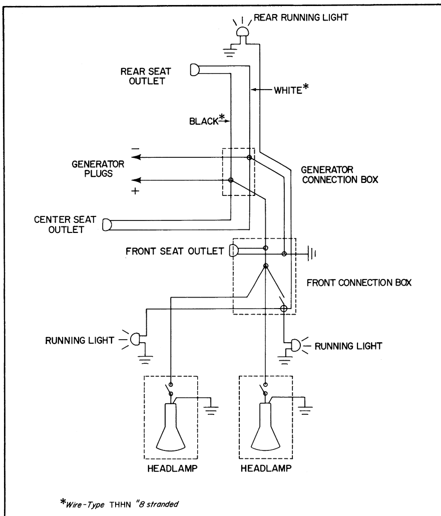
FIGURE 16. Twelve-volt lighting and auxiliary circuit
