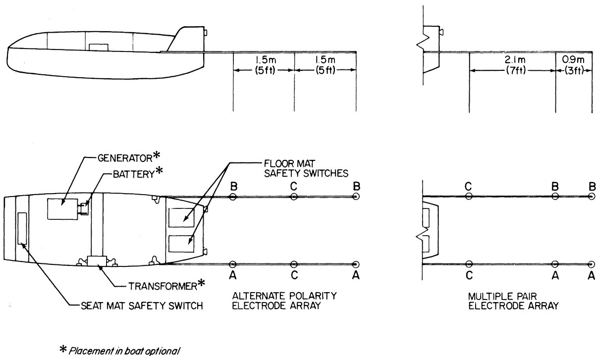
FIGURE 10. Configuration of the electrodes and the location of the major components of the ac electro-fishing boat
