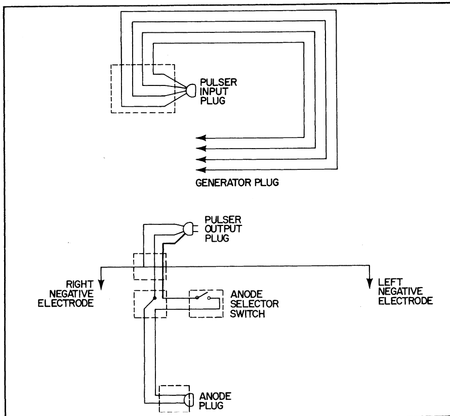
FIGURE 14. Power circuits for ac-pulsed dc electrofishing boat
