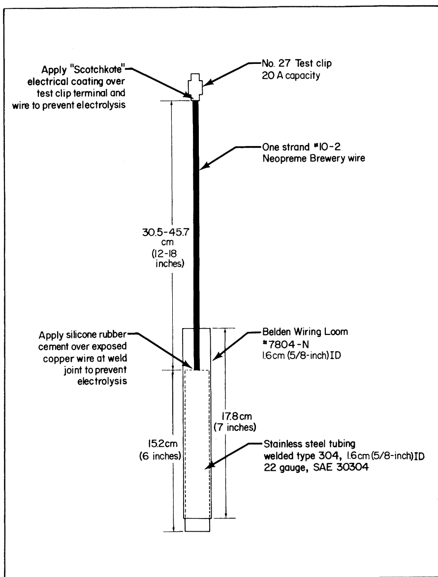
FIGURE 8. Detail of "dropper" electrodes
