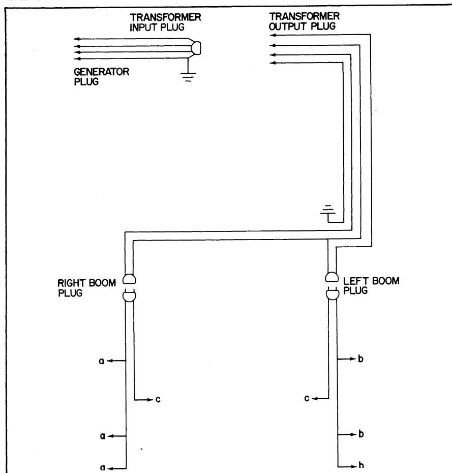
FIGURE 15. Power circuits for ac electrofishing boat
