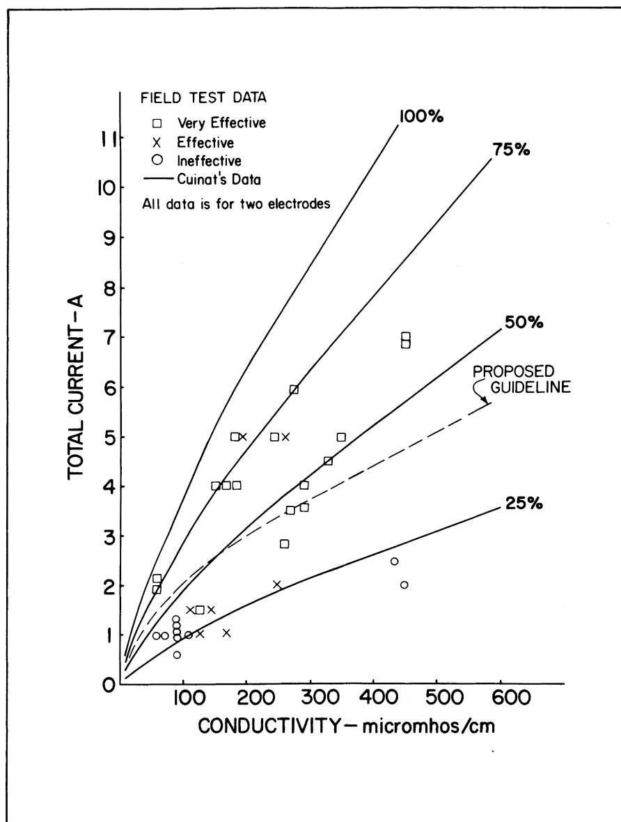
FIGURE 4. Required current for effective stream shocking with direct current using two anodes
