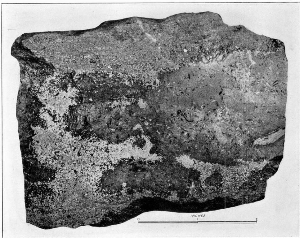
B. BASAL COMPACT BEDS OF GALENA FORMATION. G. WRIGHT'S QUARRY, LANCASTER, WISCONSIN
