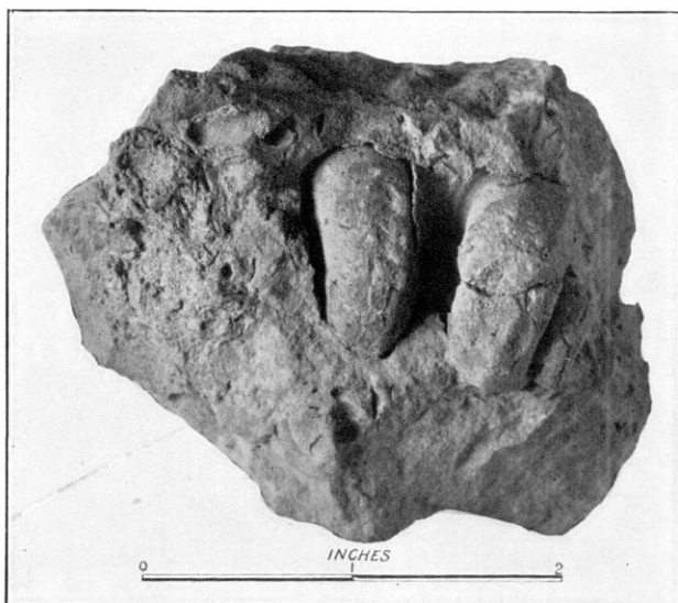
4. HOLLOW GASTROPOD CAST ENCLOSED BY PERFECT DOLOMITE MOLDS. FROM THE BLACK RIVER NEAR БЕЛОИТ, WISCONSIN
