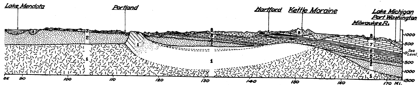
Figure 3.—East and west cross-section of Wisconsin through Blue Mounds, showing (1) the pre-Cambrian rocks, (2) the Cambrian sandstone, (3) the Lower Magnesian dolomite, (4) the St. Peter sandstone, (5) the Galena and Black River dolomite, (6) the Richmond or Maquoketa shale, (7) the Niagara formation, and (8) the glacial drift.
