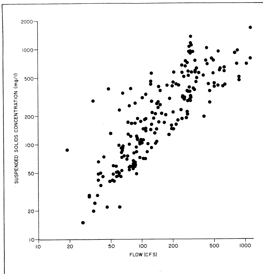
FIGURE 1. Suspended solids concentration vs. flow at 70th Street.
