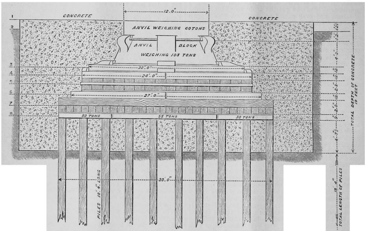
Foundations for 30-ton Steam Hammer.
