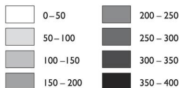
Figure 10. Thickness and extent of the unlithified aquifer in Sauk County.
