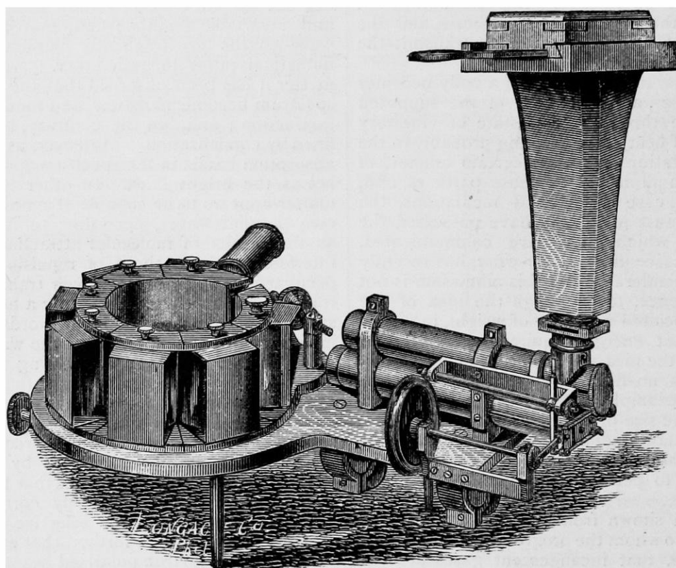
FIG. 1.—A NEW FORM OF SPECTROSCOPE
