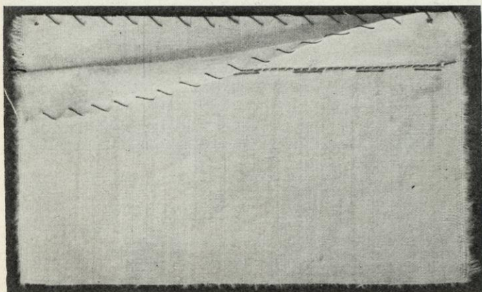
FIG. 118.—Plain seam.
