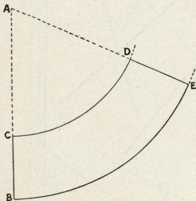
FIG. 56.—Draft of pattern for circular flounce for petticoats.
