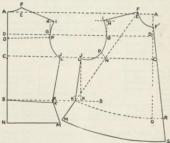
FIG. 45.—Draft of pattern for a mannish shirt.
