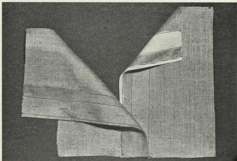
FIG. 197.—Placket facing in tuck opening.
