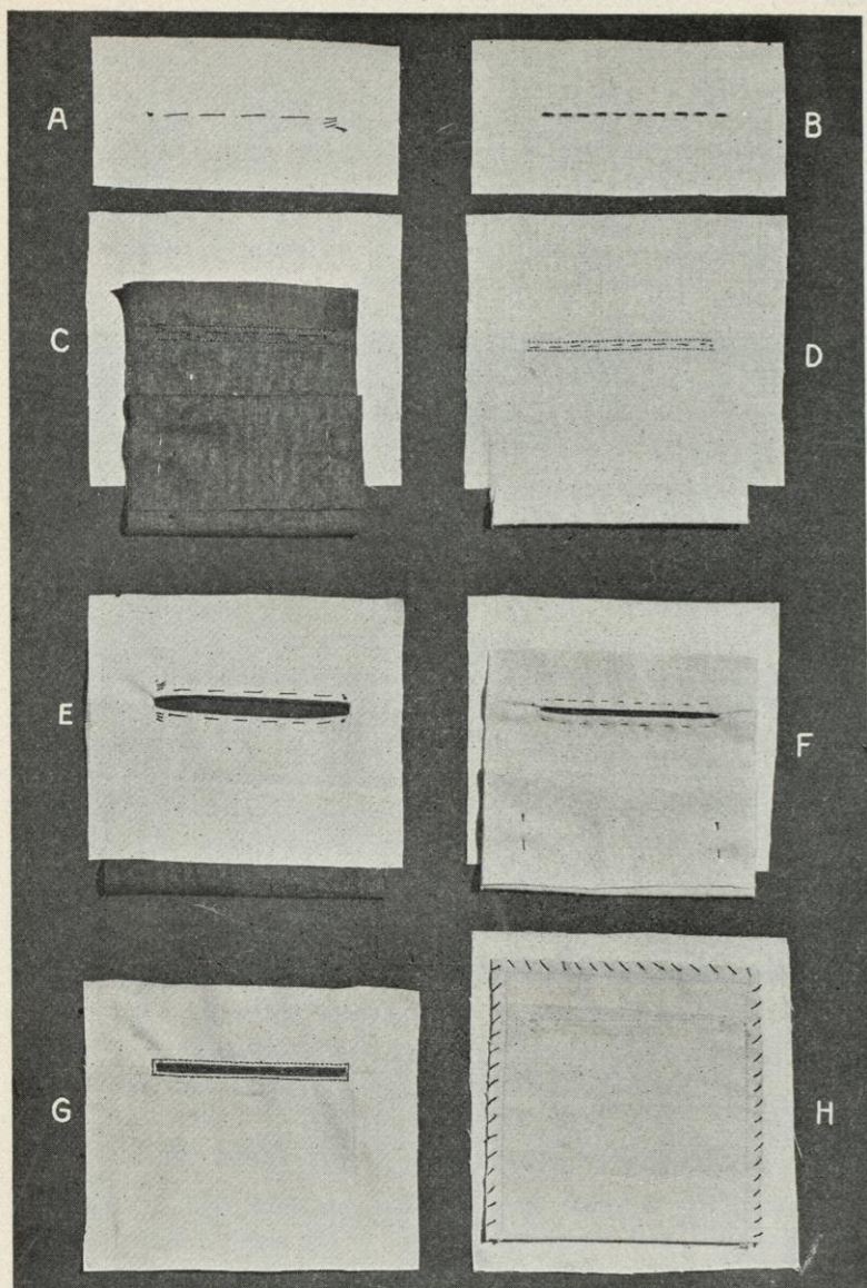
FIG. 174.—Set-in pocket; A, basting to mark for slit, right side garment; B, wrong side of A; C, pocket basted to right side of garment; D, wrong side C; E, pocket drawn through to wrong side garment, edge basted; F, wrong side E; G, pocket stitched, right side; H, completed pocket, wrong side.
