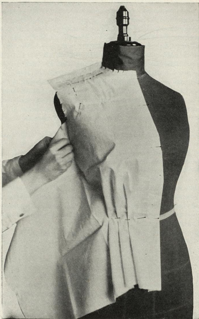
FIG. 80.—Draping a simple waist.
