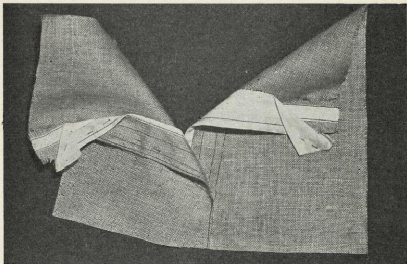
FIG. 196.—Placket facing on bias seam.
