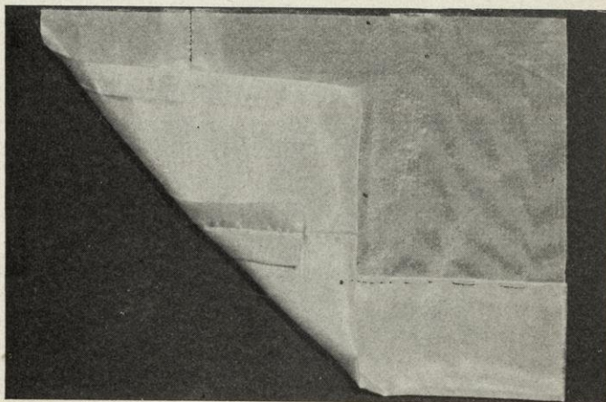
FIG. 233.—Reversed hem.
