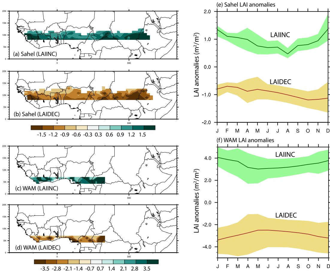
Figure 9 LAI anomalies ( m^2 m^{-2} ) in the (a,c) LAIINC and (b,d) LAIDEC dynamical experiments with modified LAI ( EXP_{LAI} ) across the (a,b) Sahel and (c,d) WAM region with the (e, f) seasonal cycle of area-average LAI anomalies. Green and brown lines in (e-f) represent area-average LAI anomalies averaged across LAIINC and LAIDEC members, respectively, and the shading denotes the minimum and maximum anomalies among all members.
