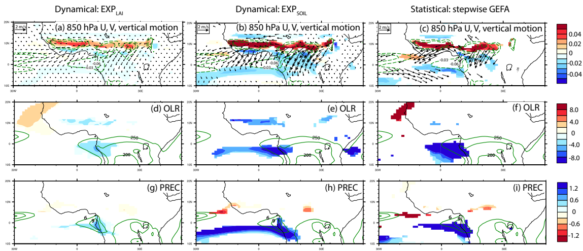
Figure 29 Dynamically and statistically assessed responses to LAI anomalies across the Sahel in December. Response fields include (a-c) 850-hPa wind ( \text{m s}^{-1} \text{LAI}^{-1} , vector) and vertical motion ( \text{Pa s}^{-1} \text{LAI}^{-1} , shading), and (d-f) OLR ( \text{W m}^{-2} \text{LAI}^{-1} , shading), and (g-i) and precipitation (PREC) ( \text{mm d}^{-1} \text{LAI}^{-1} , shading). Climatology of December 850-hPa vertical motion ( \text{Pa s}^{-1} ), OLR ( \text{Pa s}^{-1} ), and precipitation ( \text{mm d}^{-1} ) in CTRL are shown in (a-c), (d-f), and (g-i), respectively, by green contours. Dynamical responses are assessed from the (a,d,g) EXP LAI and (b,e,h) EXP SOIL ensembles. Statistical responses are assessed based
