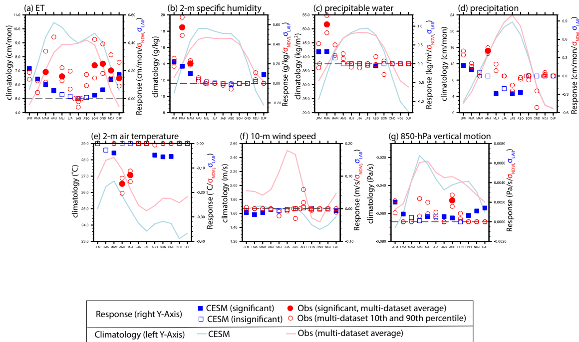
Figure 48 Same as Figure 47, but for local responses to vegetation anomalies across HOA.
