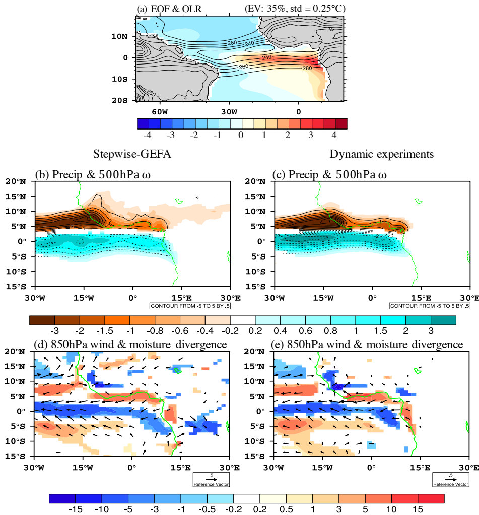
Figure 23 (a) Climatological OLR (contour, unit: \text{W m}^{-2} ) and leading EOF of SST over the tropical Atlantic Ocean based on 300-year CTRL for June in CESM. The magnitude of the spatial pattern is normalized with a standard deviation of 1^\circ\text{C} . The explained variance (EV) and standard deviation (std) of corresponding PCs are indicated in parentheses. Precipitation (shading, unit: \text{mm day}^{-1} \sigma_{PC}^{-1} ) and 500-hPa vertical motion (contour, unit: \text{Pa s}^{-1} \sigma_{PC}^{-1} ) response to TA1 forcing using (b) stepwise-GEFA and (c) dynamical experiments during June. 850-hPa moisture divergence (shading, unit: 10^{-6} \text{kg m kg}^{-1} \text{s}^{-1} \sigma_{PC}^{-1} ) and 850-hPa wind response (vector, \text{m s}^{-1} \sigma_{PC}^{-1} ) for TA1 forcing using (d) SGEFA and (e) dynamical experiments. Only statistical significant response ( p < 0.1 ) fields are shown.
