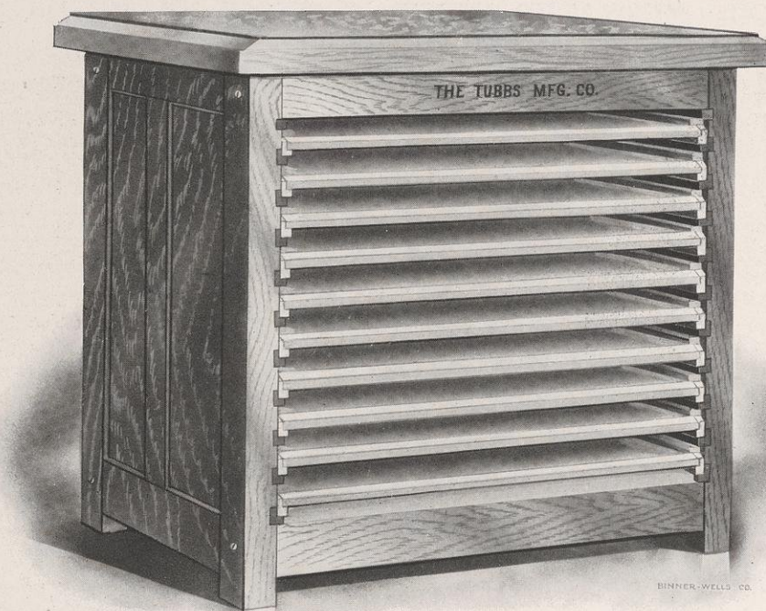
Tubbs Imposing Table No. 151 With 10 Letter Boards. Size of Stone, 24x36 Inches List Price, Complete, Panel Ends, $44.00. Open Ends, $40.00
