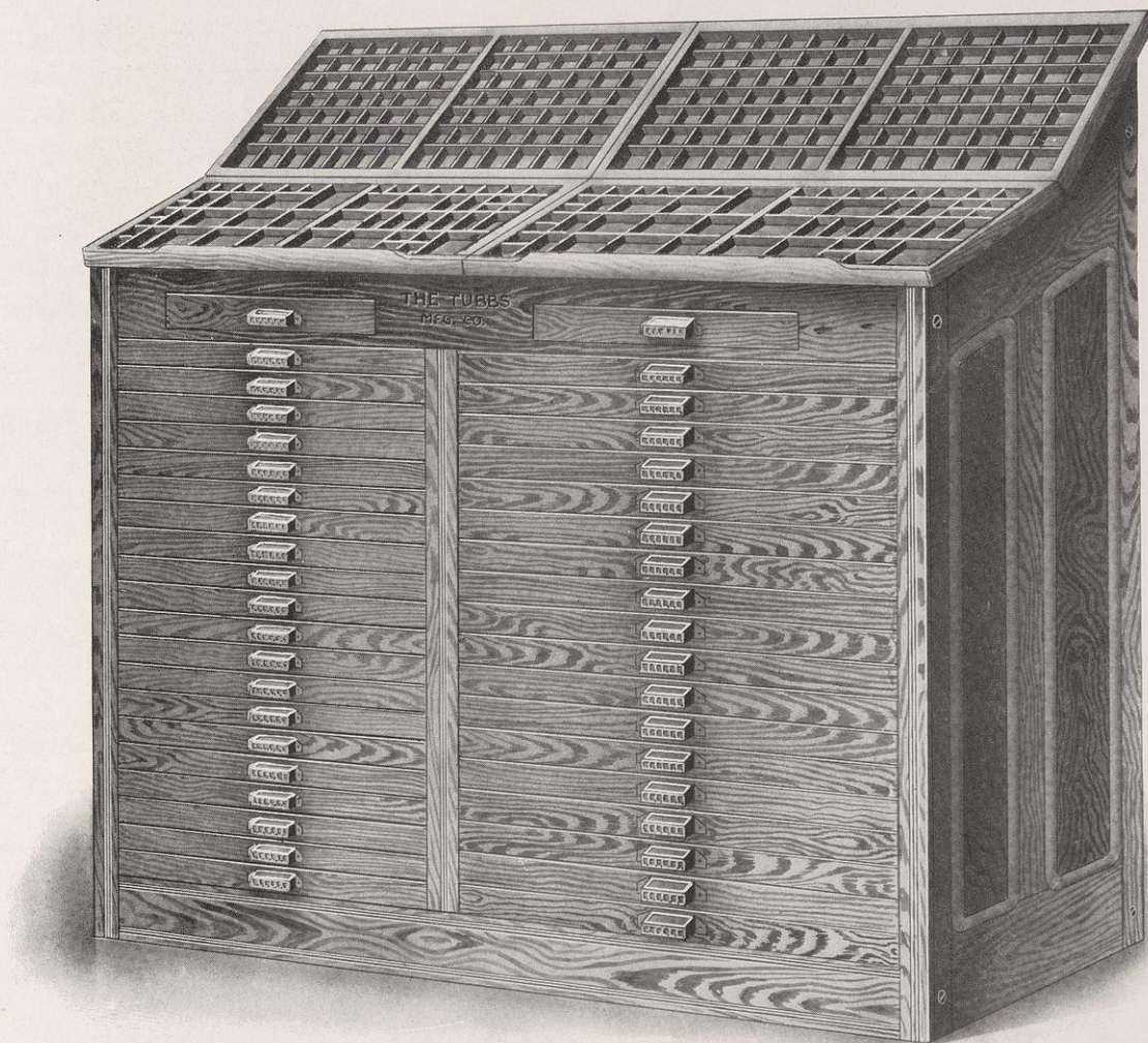
Tubbs Standard Cabinet No. 294 Wood Slides
