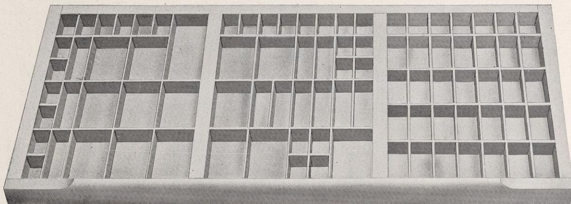
This is Tubbs New Idea Case with White Rock Maple Triple Veneer Bottom
