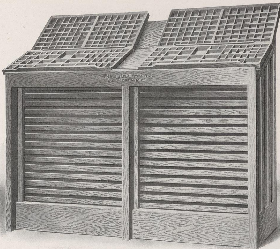
Tubbs Steel Slide Case Stand No. 127, Front View List Price, $25.00
