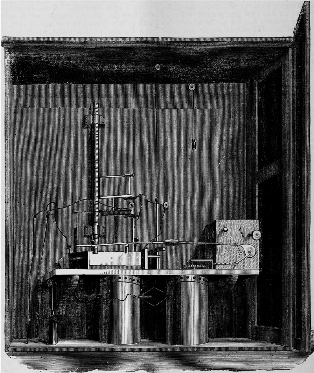
FIG. 4.—PROF. HOUGH'S NEW PRINTING BAROMETER
