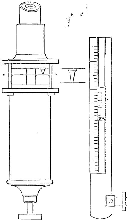
FIG. 6.—SECTION OF GREEN'S STANDARD BAROMETER
