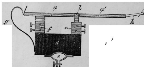
FIG. 3.—The marking lever for indicating graphically on a revolving drum the moment at which an electric current is broken.
