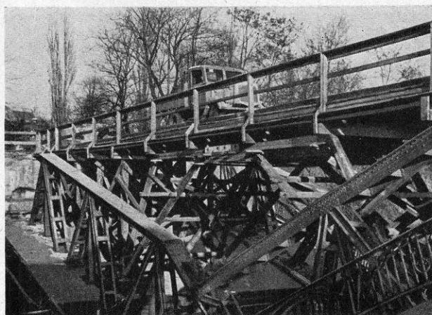
Bridge repairs in Berlin were essential before normal transportation could be resumed. Five out of every six bridges in the U.S. Sector had been destroyed.
