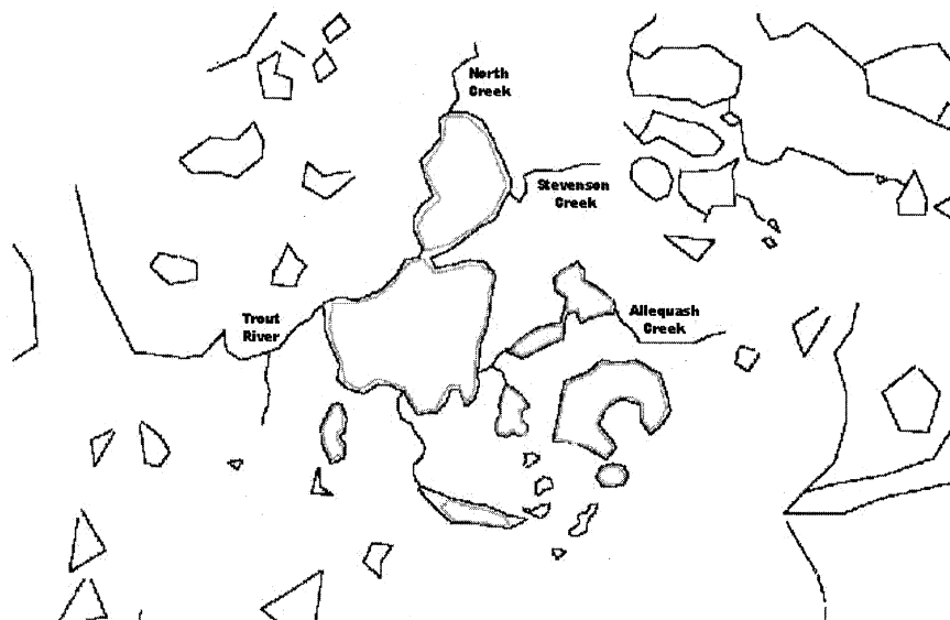
Figure 4. Analytic element model of the Trout Lake basin showing location of tributary streams.
