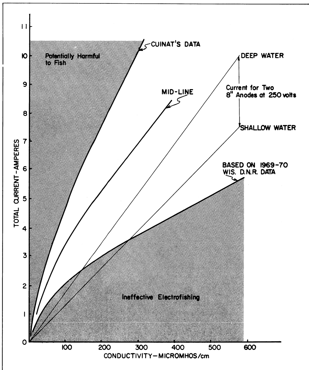
FIGURE 2. Proposed guideline for stream shocking with direct current using two anodes.
