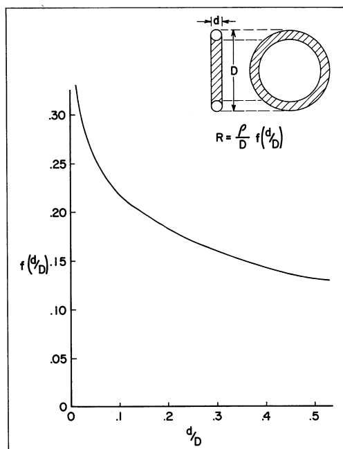
FIGURE 9. Resistance in ohms of a ring electrode.
