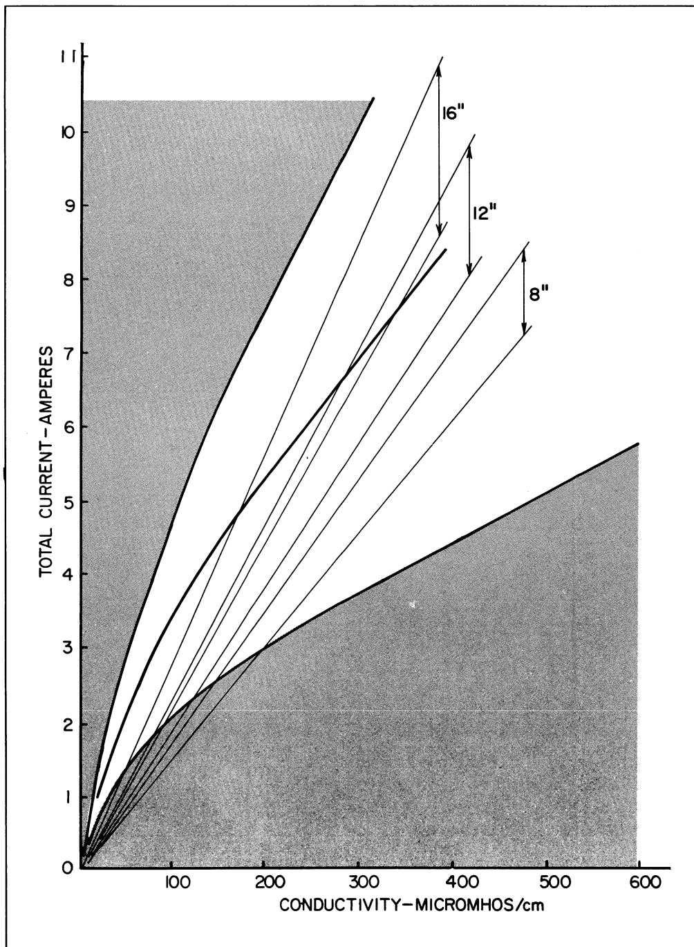
FIGURE 5. Effect of doubling effective cathode size using two anodes in shallow water at 300 volts.
