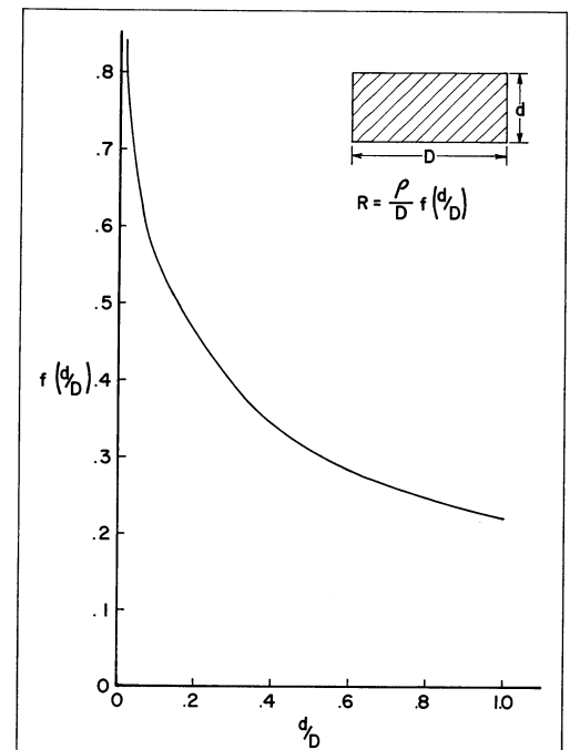
FIGURE 11. Resistance in ohms of a rectangular plate electrode.
