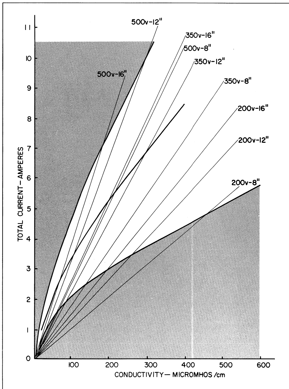
FIGURE 4. Effect of varying anode size and voltage using two anodes in shallow water.
