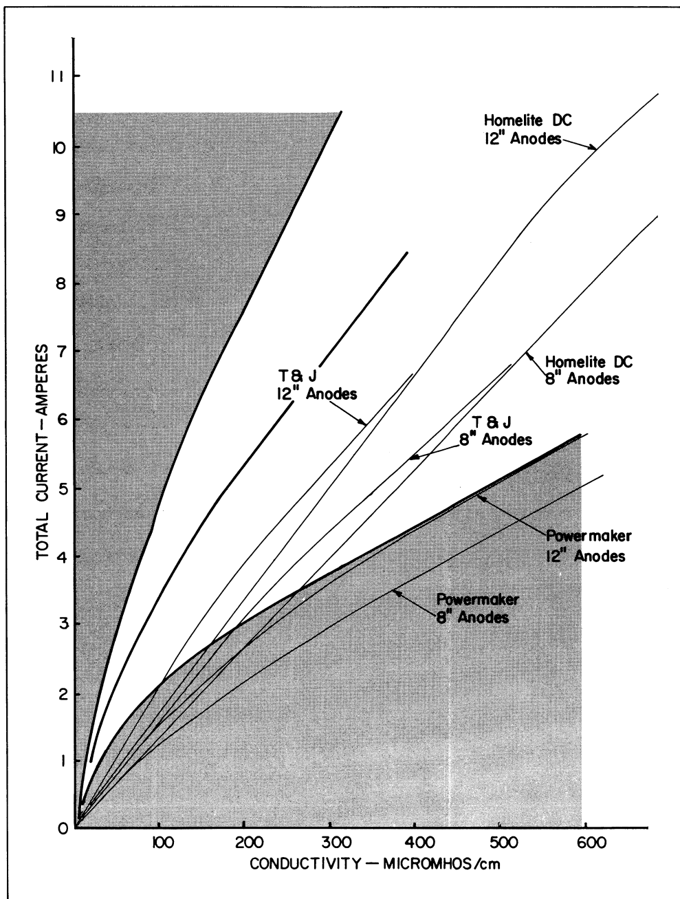
FIGURE 6. Effect of generator characteristics on fishing efficiency using two anodes in shallow water.
