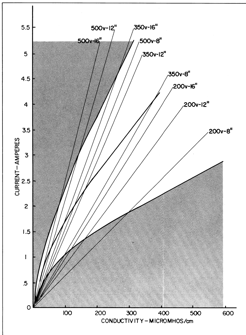
FIGURE 8. Effect of varying anode size and voltage using one anode in shallow water.
