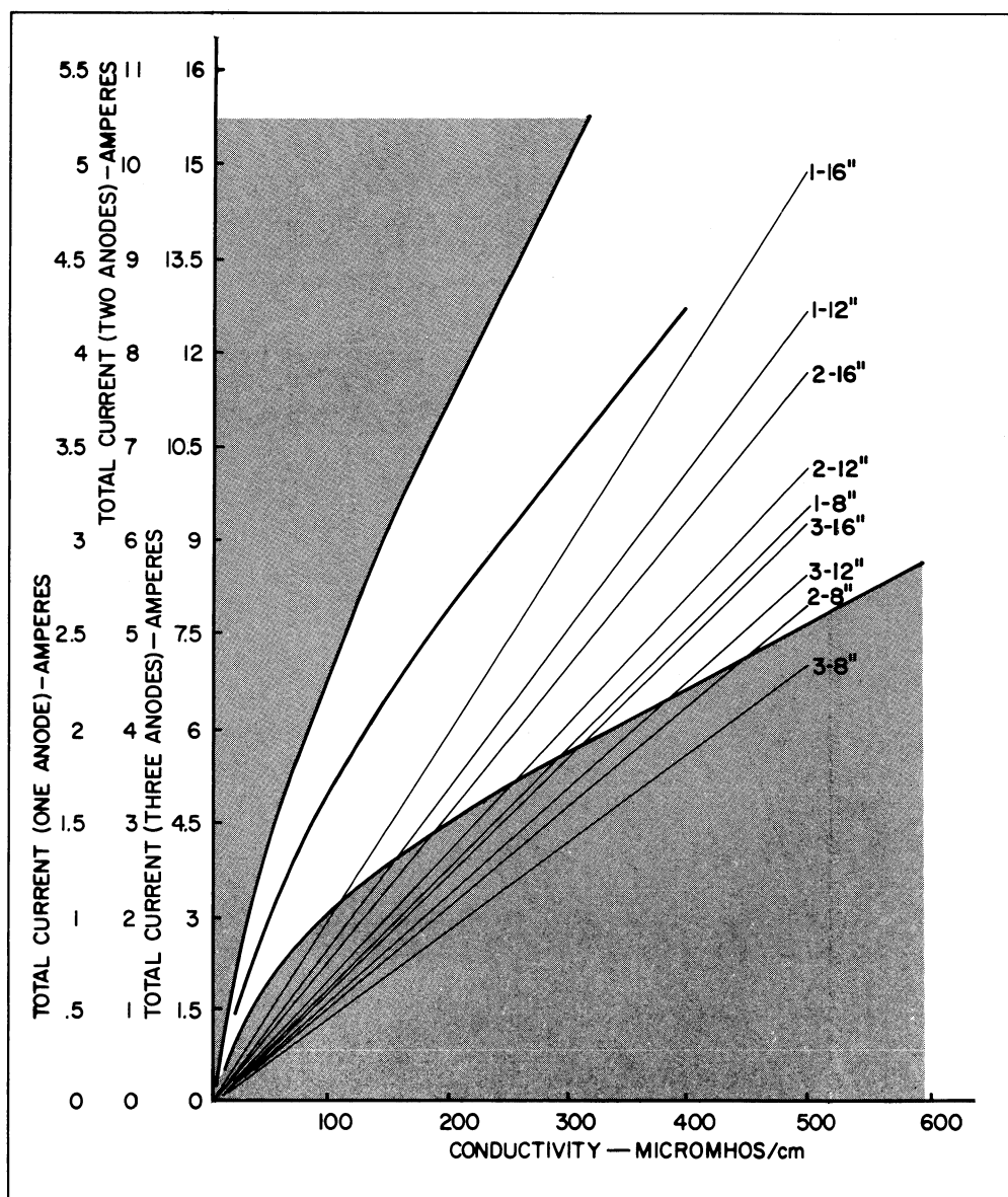
FIGURE 7. Effect of varying the number of anodes in shallow water at 200 volts.
