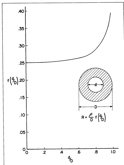
FIGURE 10. Resistance in ohms of a circular disc electrode.
