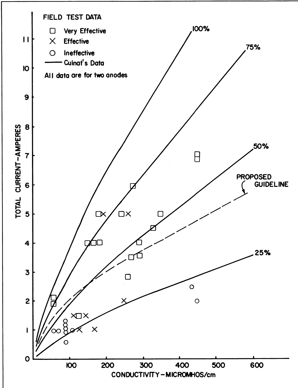
FIGURE 1. Required current for effective stream shocking with direct current using two anodes.
