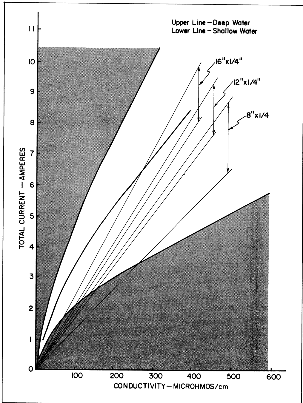
FIGURE 3. Effect of varying anode size using two anodes at 250 volts.
