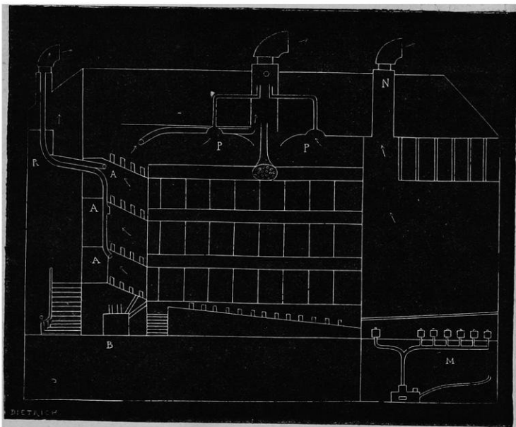
FIG. 1.—Ventilation of a Theatre (Chavannes' system).
