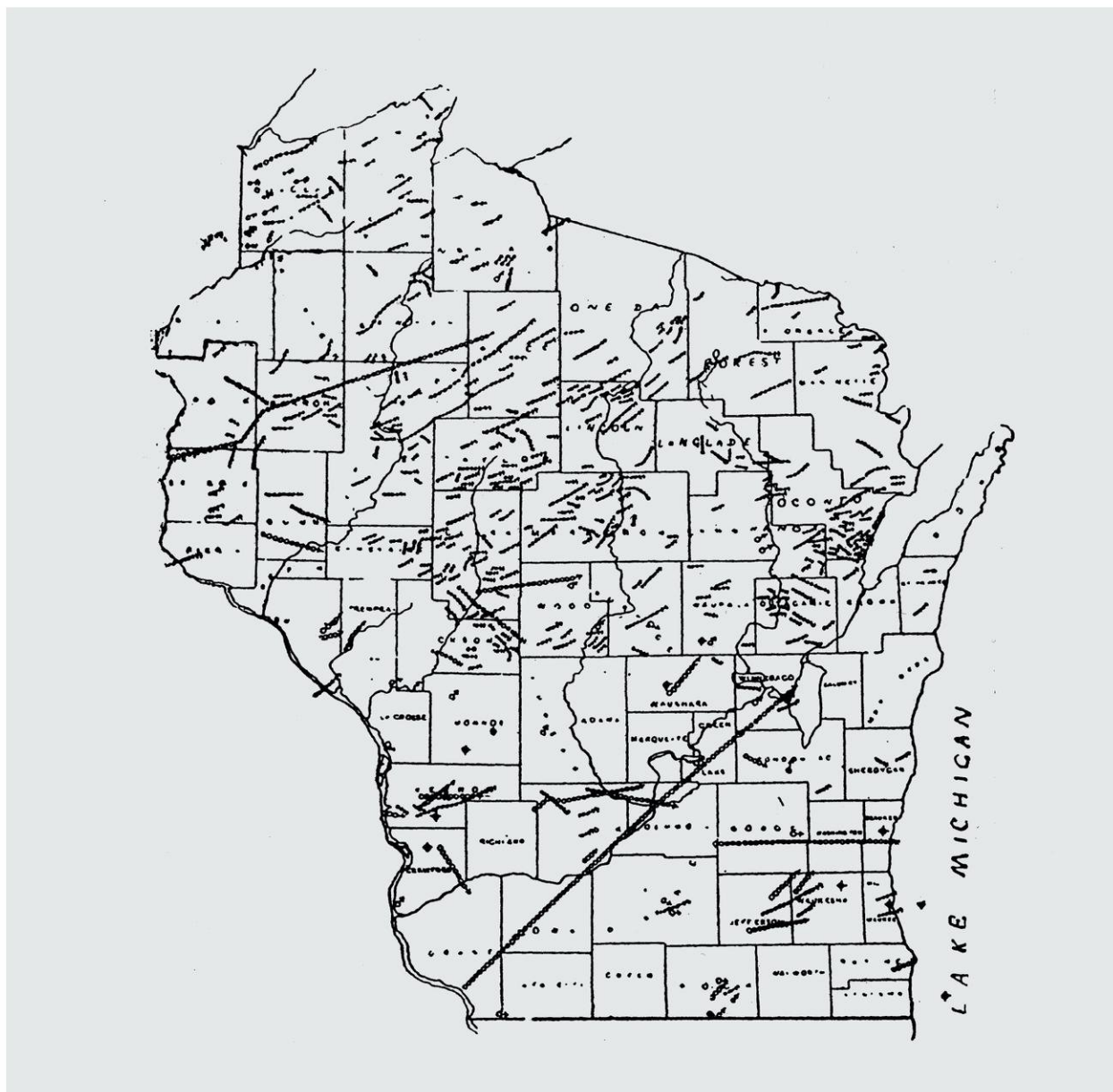
Figure 2. Tornado paths of Wisconsin tornadoes, 1844–80, from Finley (1888).
