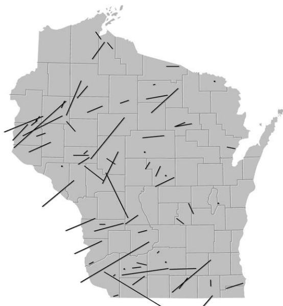
Figure 32. Paths of historic killer tornadoes before 1950.
