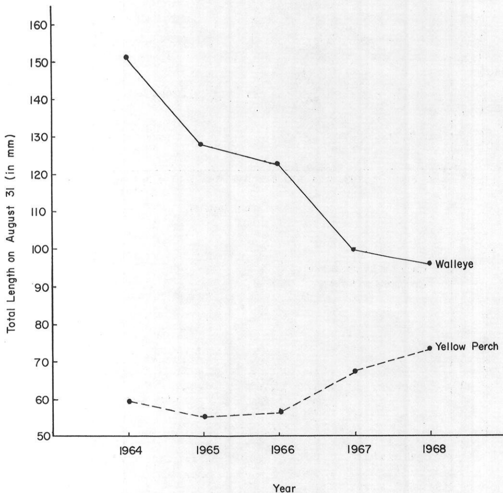
Figure 2. Total length on the same day for young-of-the-year walleyes and yellow perch, 1964-68.
