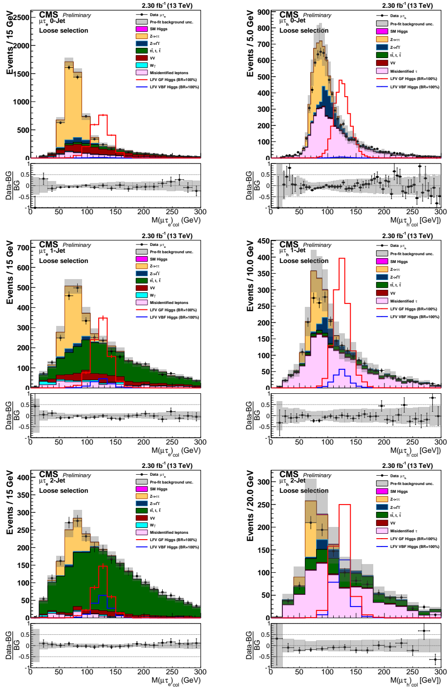
Figure 6.7: Distributions of the collinear mass M_{collinear} at \sqrt{s} = 13 TeV, for signal with B(H \rightarrow \mu\tau) = 100\% for clarity, and background processes after the loose selection requirements for the LFV H \rightarrow \mu\tau candidates for the different channels and categories compared to data. The shaded grey bands indicate the total uncertainty. The bottom panel in each plot shows the fractional difference between the observed data and the total estimated background. Top left: H \rightarrow \mu\tau_e 0-jet; top right: H \rightarrow \mu\tau_h 0-jet; middle left: H \rightarrow \mu\tau_e 1-jet; middle right: H \rightarrow \mu\tau_h 1-jet; bottom left: H \rightarrow \mu\tau_e 2-jet; bottom right H \rightarrow \mu\tau_h 2-jet.
