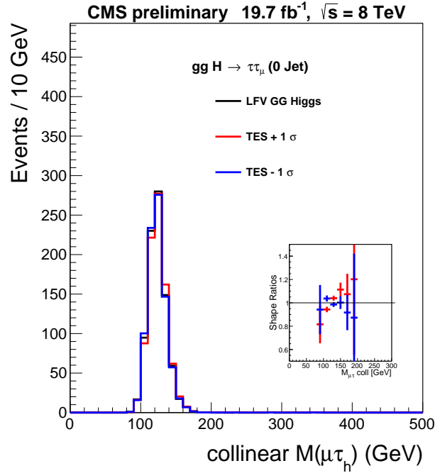
Figure 6.10: The effect of shifting the tau energy scale by \pm 1\sigma . The shift in this is shown for the LFV signal in the 0 jet category.
