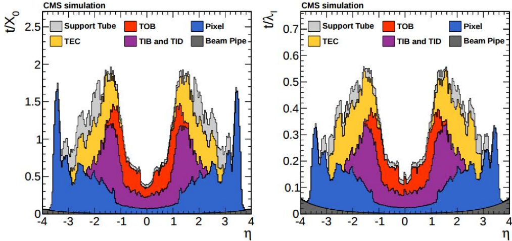
Figure 3.4: Width of the tracker in unites of radiation length (left) and nuclear interaction length (right) [41]
