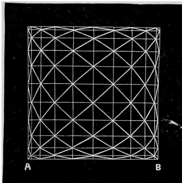
FIG. 13.—Diagram showing approximately the theoretical path of a spring vibrating without friction, with periods of vibration in cross-planes in the proportion of n to n + 1 . ( n = 10 .) A and B are the beginning and end of the cycle, perpetually retraced, and are analogous to the two cusps of Fig. 9 or Fig. 11.
