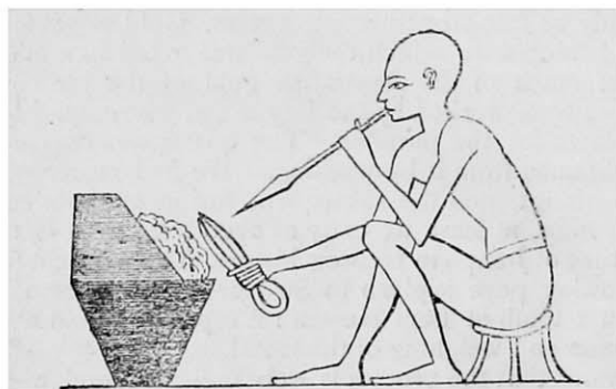
FIG. 2.—Furnace and Blow-pipe from Egyptian Tomb
