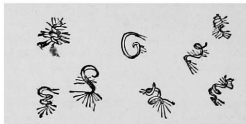
FIG. 6.—Antherozoids
