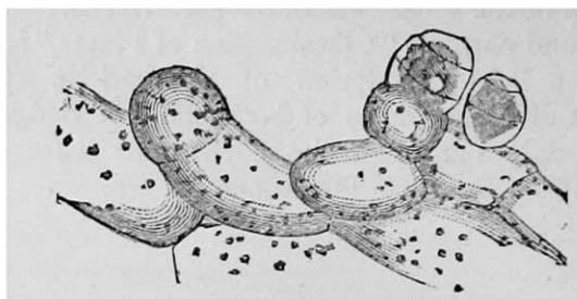
FIG. 5.—Antheridia (magnified)
