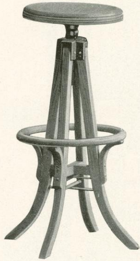
No. 200 Screw Stool Oak, Office Color, Rubbed Height 33 inches Seat 14 inches wide, 14 inches deep, 1½ inches thick K. D.
