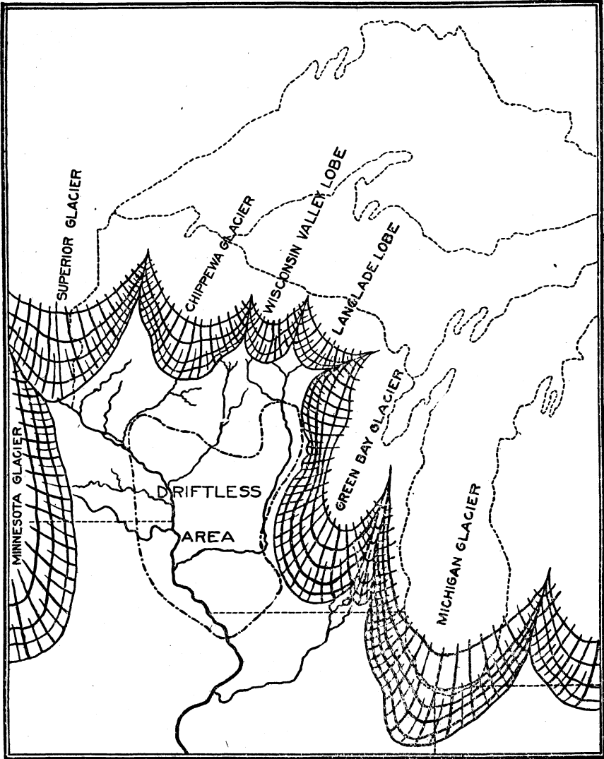
Fig. 2. Sketch map showing the location of the Wisconsin ice sheet. (After Weidman.)
