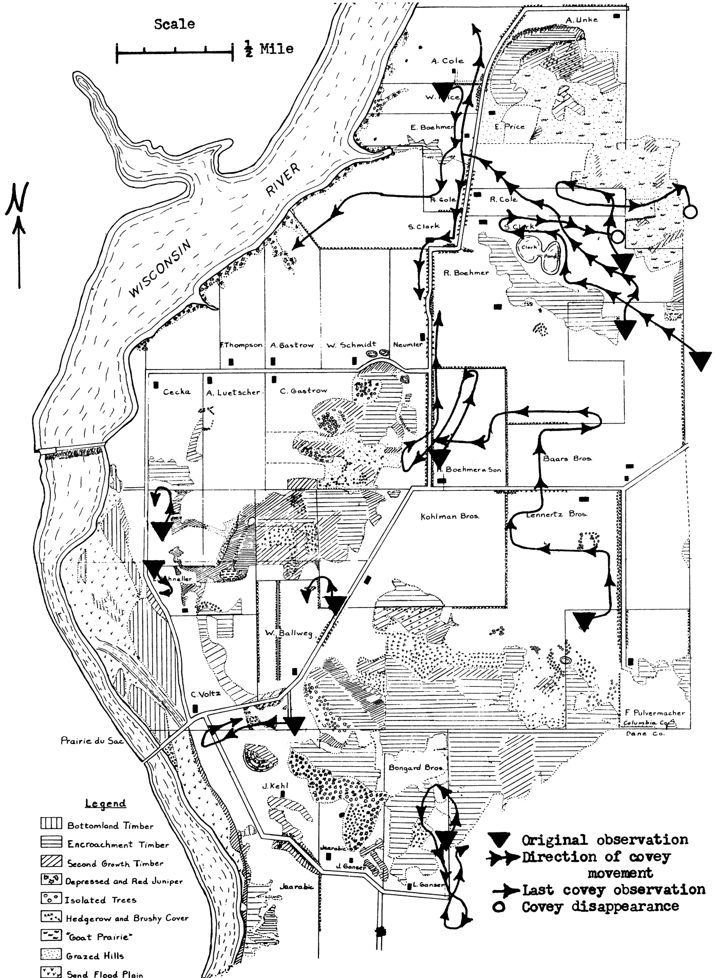
Figure 13. Quail covey movement at Prairie du Sac in the winter of 1946-47 showing maximum ranging.
