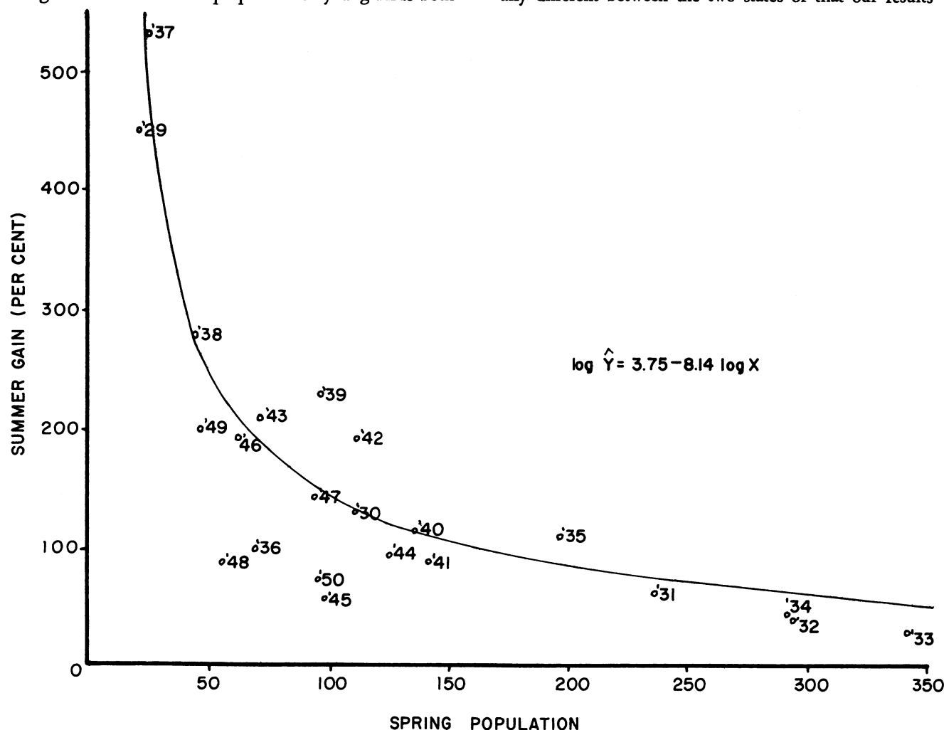
Figure 25. The regression of the percentage of summer gain on spring population for Prairie du Sac quail, 1929-50.
