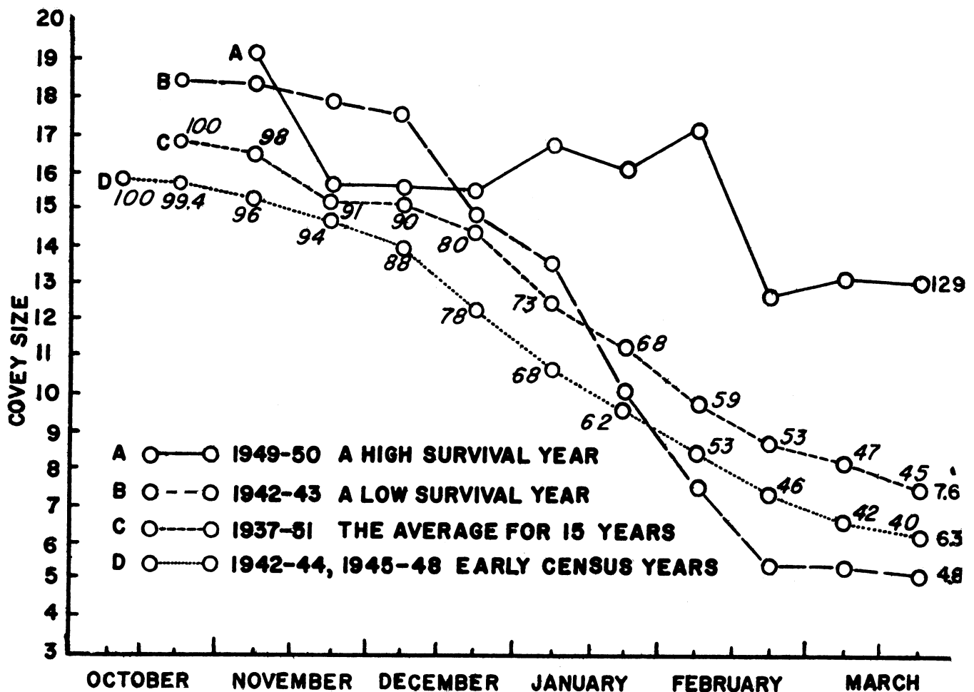
Figure 9. The shrinkage of Prairie du Sac quail coveys in winter. (The numbers on curves C and D express covey survival in per cent.)
