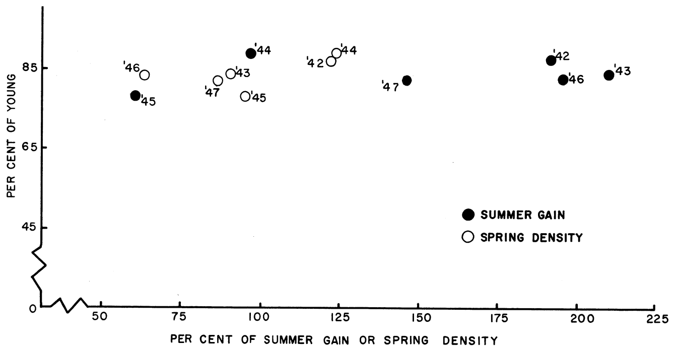
Figure 26. The relationship between the percentage of summer gain and spring density with the percentage of young (Prairie du Sac).
