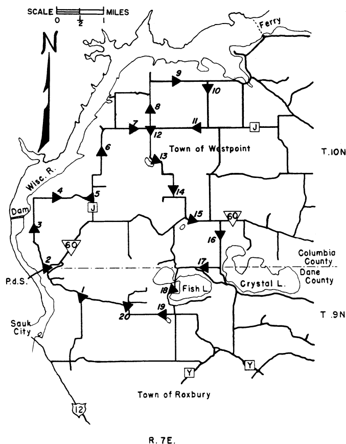
Figure 6. Stops on the whistling transect in the Prairie du Sac study area and the Towns of Westpoint and Roxbury.
