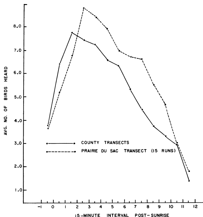
Figure 29. A comparison of the average number of bobwhites whistling at Prairie du Sac and on various county transects throughout the state.
