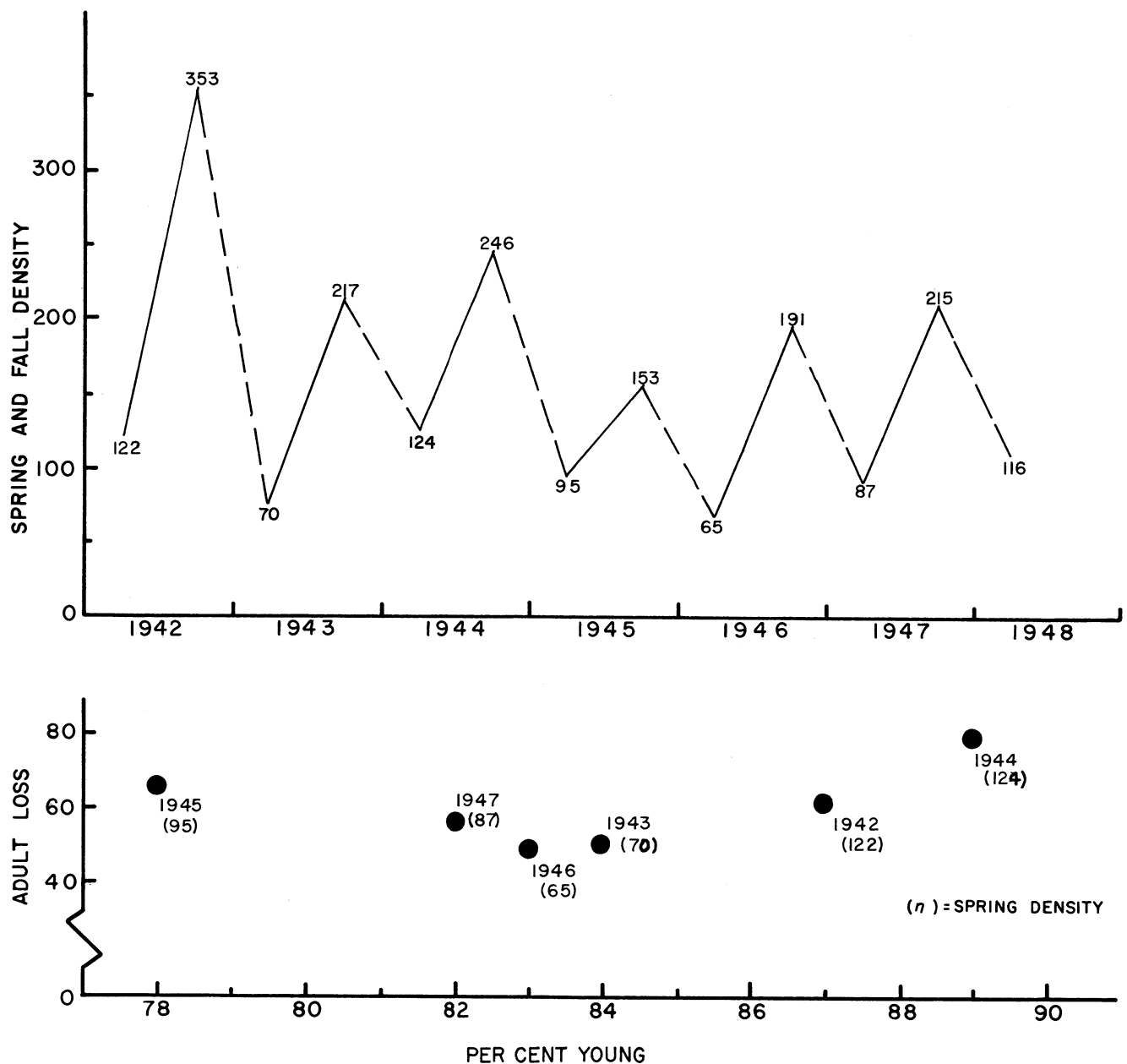
Figure 23. The spring and fall density, 1942-47, and the regression of the percentage of spring-to-fall loss of adults on the percentage of juveniles in the fall population (Prairie du Sac).
