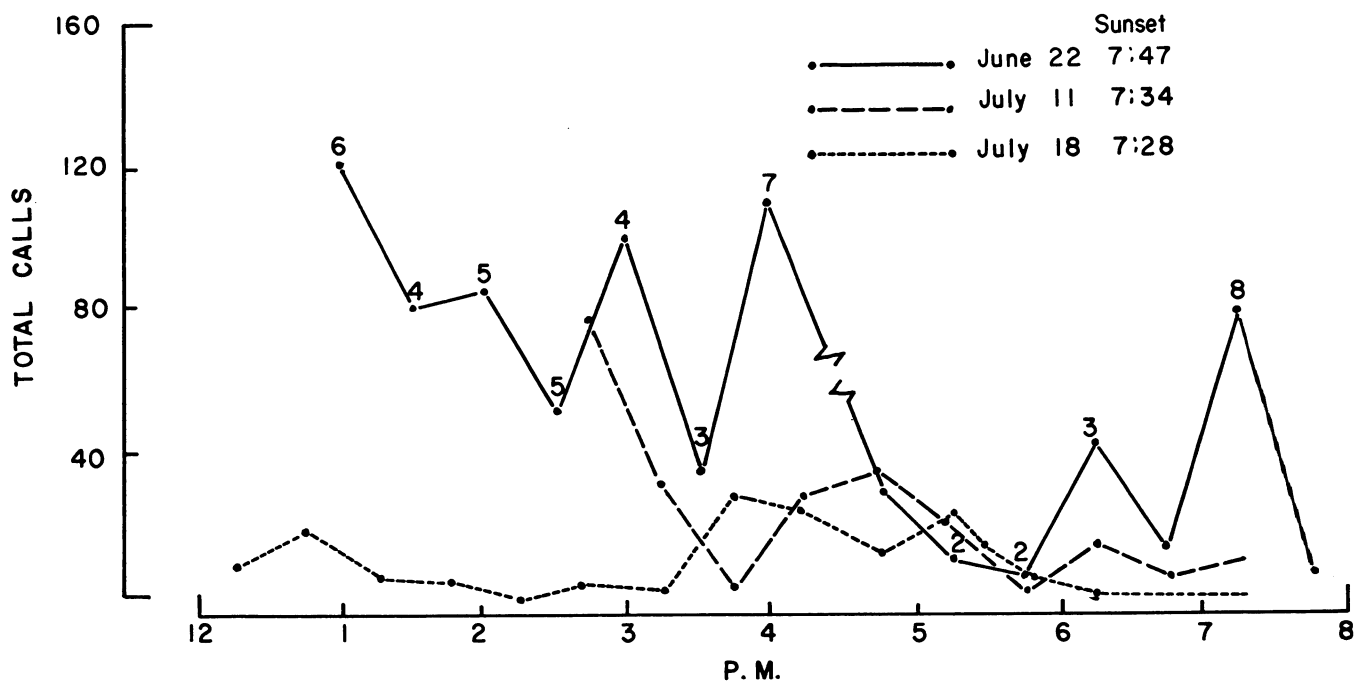
Figure 28. Daily pattern of whistling activity, afternoon hours, C.S.T., (1948) (6, 4, etc. are number of individual birds calling where known. Total calls are per half-hour interval).
