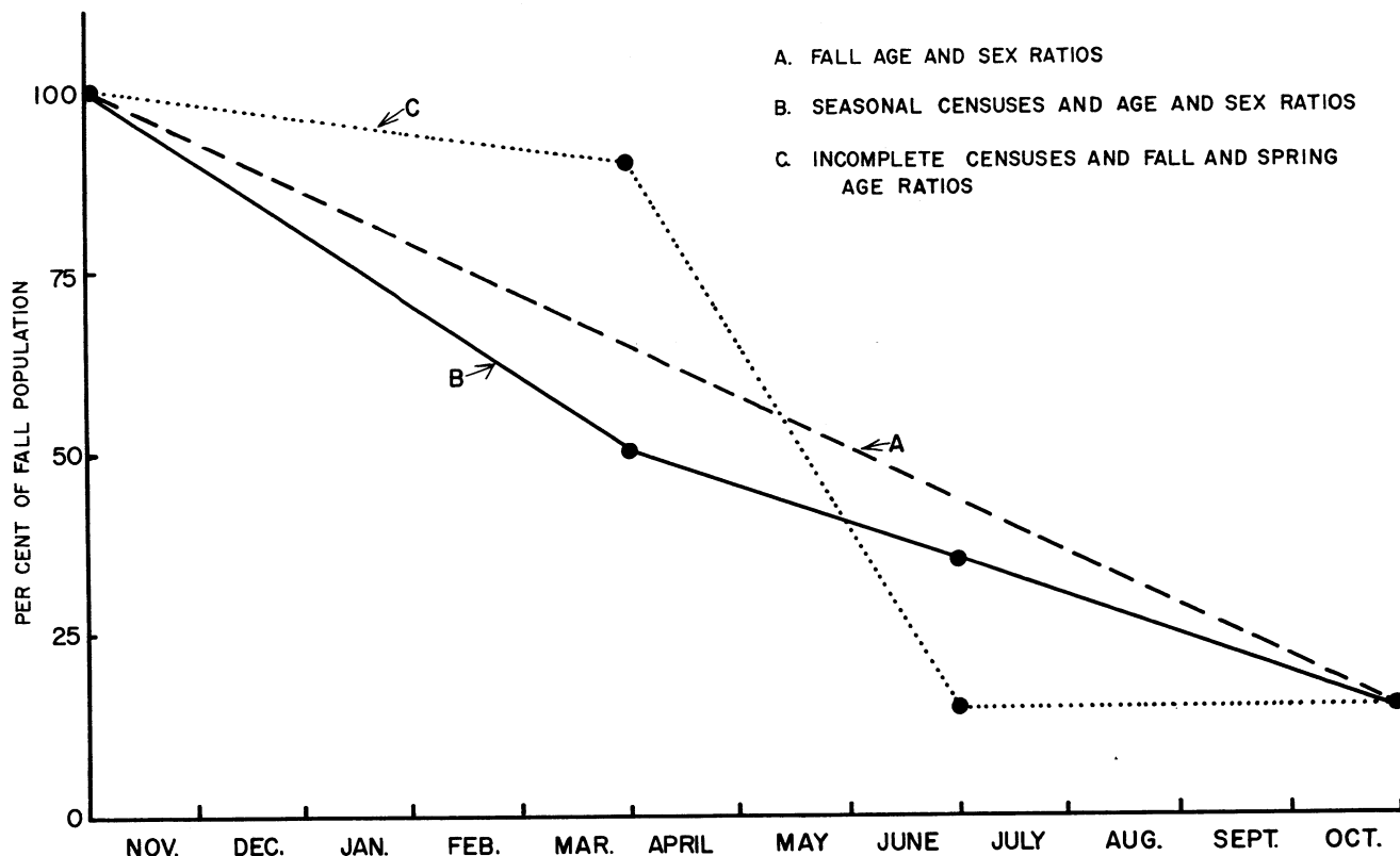
Figure 21. Shrinkage rates of a quail population based on different types of data.
