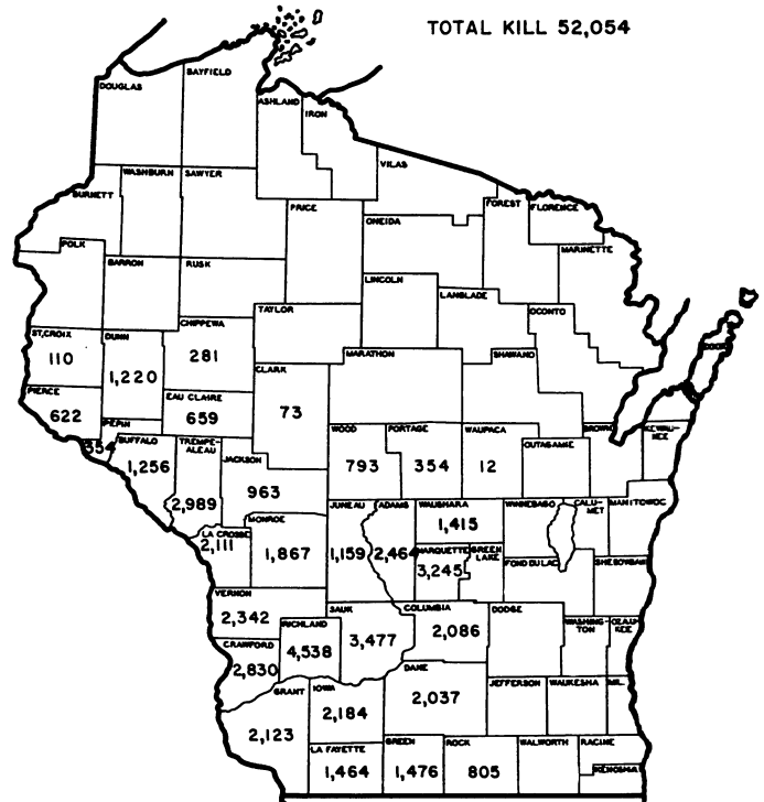
Figure 7. The estimated quail kill by counties in 1957.
