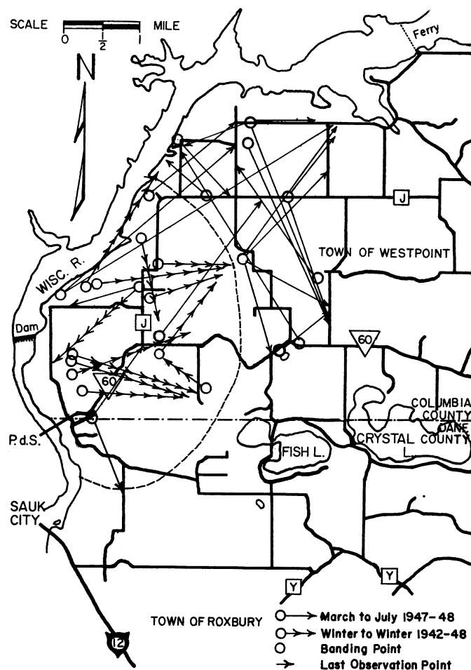
Figure 14. Quail movement from March to July and winter to winter at Prairie du Sac.
