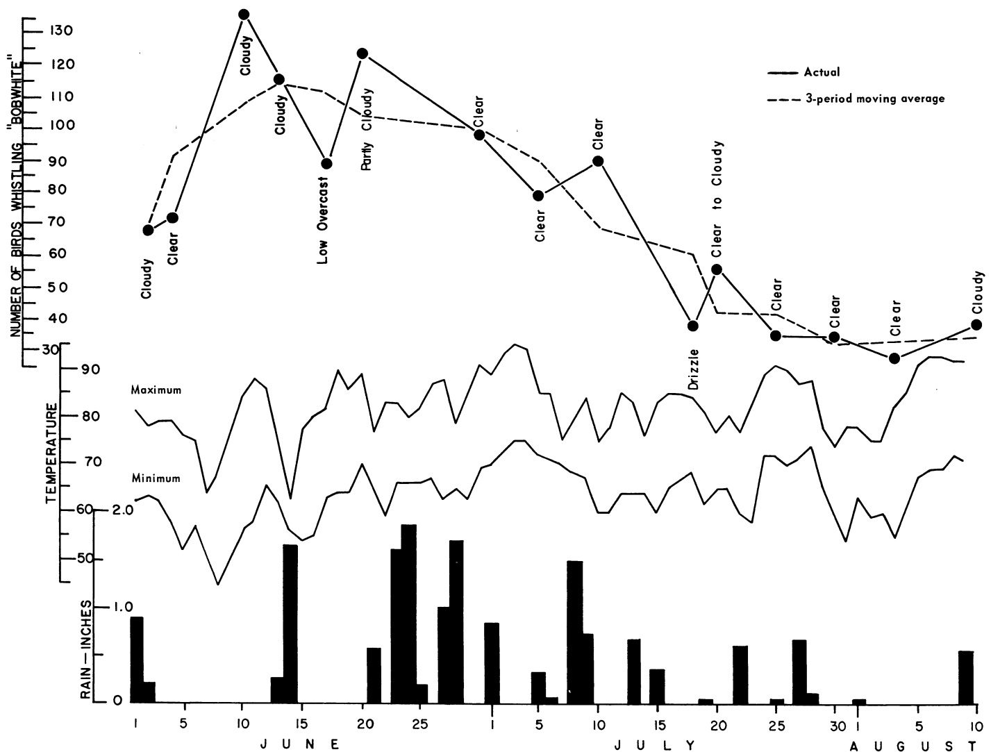
Figure 30. Seasonal pattern of whistling in bobwhite quail at Prairie du Sac, 1949, occurring under different weather conditions. (Weather data gathered at Prairie du Sac.)
