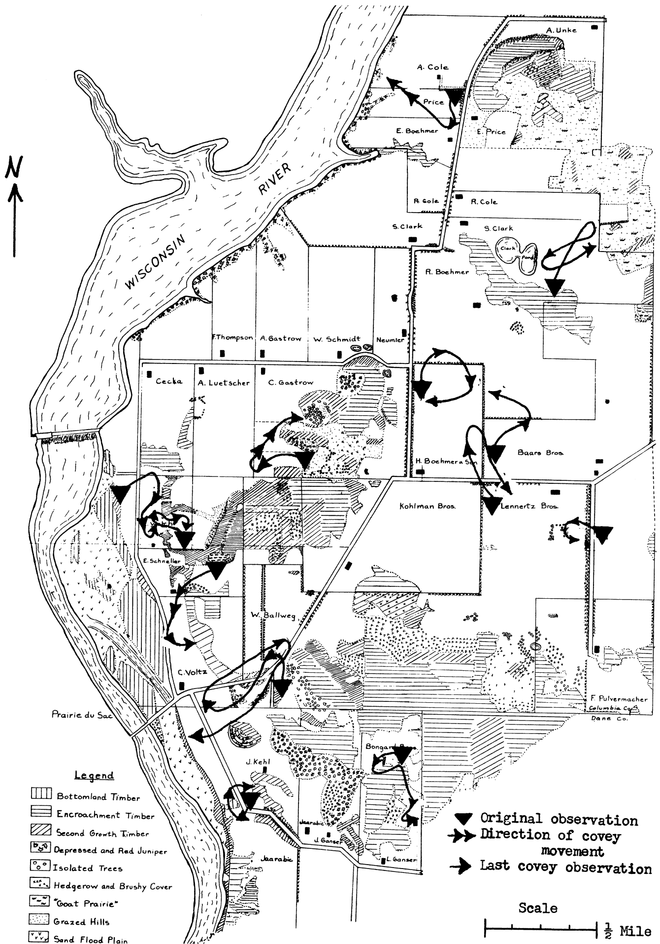
Figure 12. Quail covey movement at Prairie du Sac in the winter of 1943-44 showing minimum ranging.
