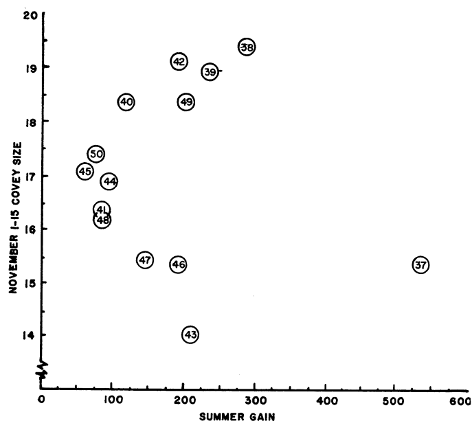
Figure 10. The relationship between covey size and the percentage of summer gain on the Prairie du Sac Study area, 1937-50.
