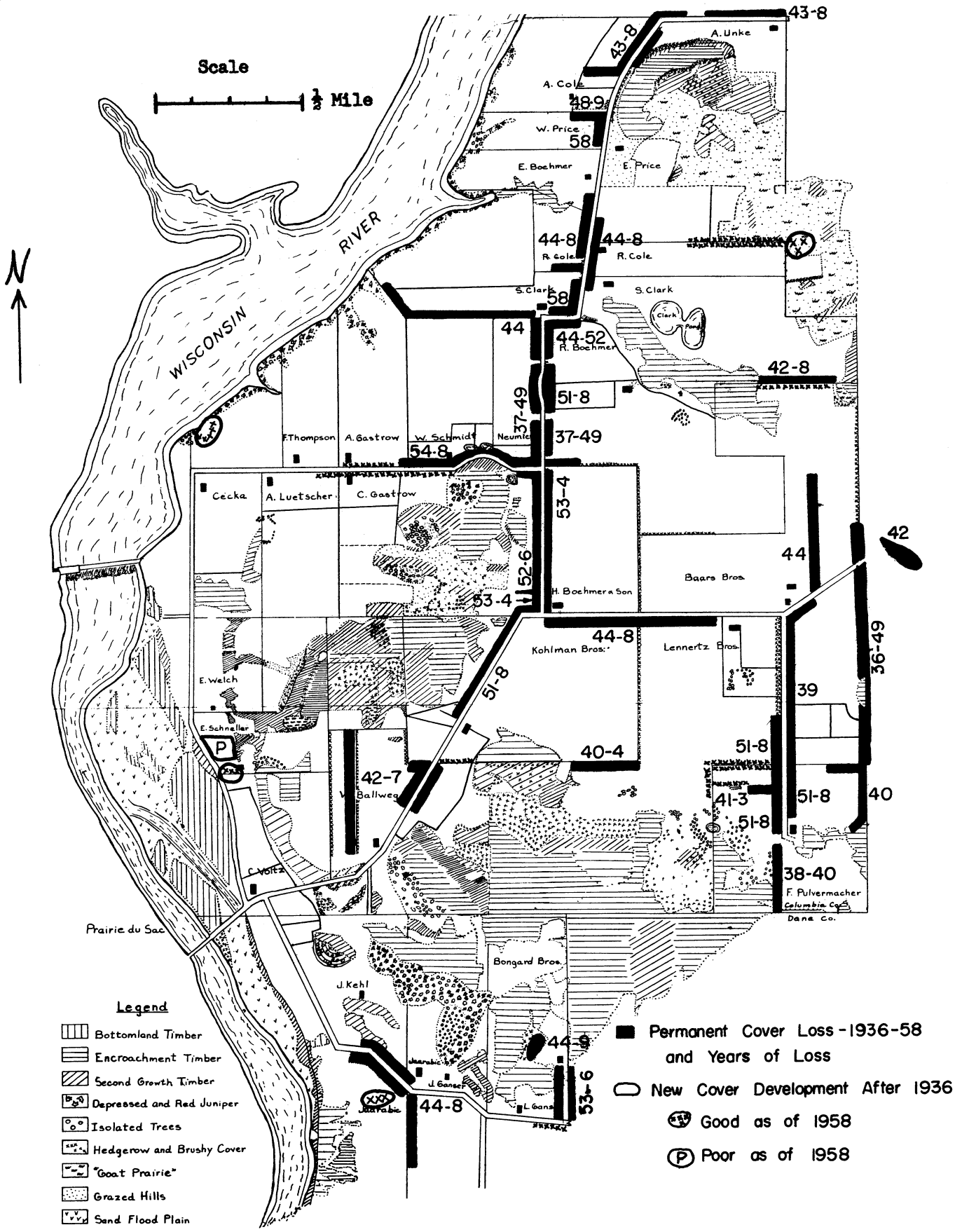
Figure 18. Roadside and fencerow cover changes on the Prairie du Sac area, 1936-58.
