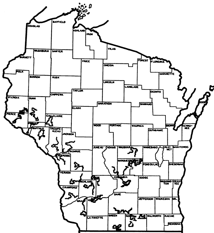
Figure 5. Location of quail whistling transects.
