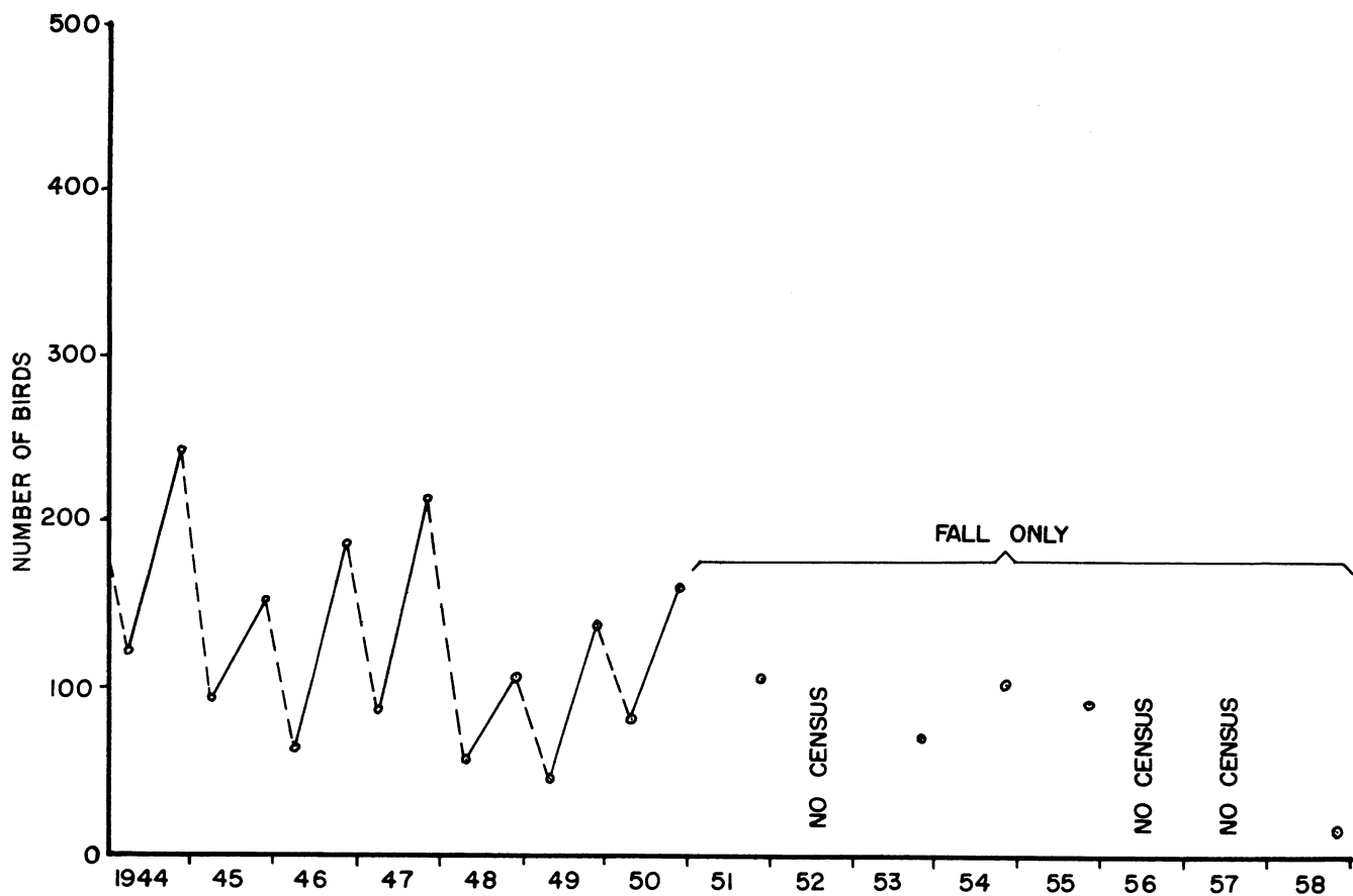
Figure 24. Fall and spring population censuses at the Prairie du Sac study area, 1929-58.
