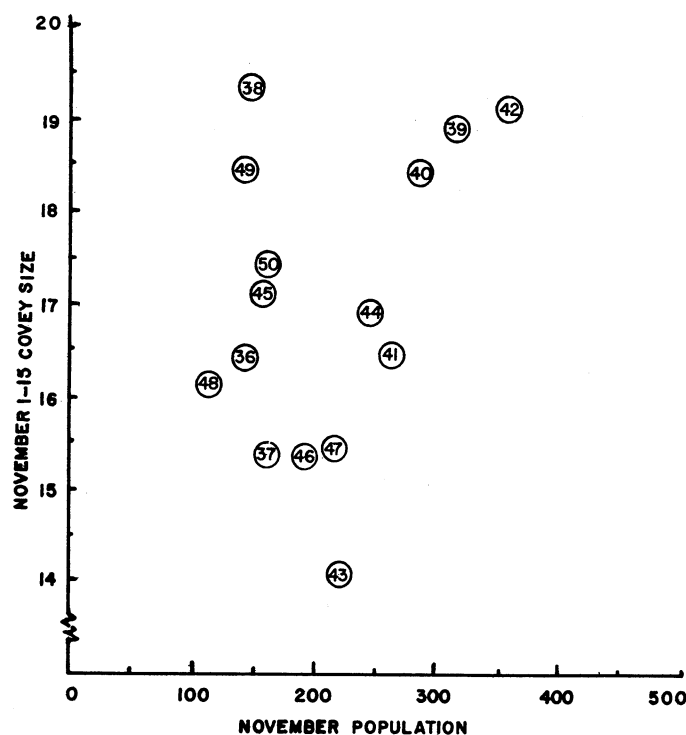
Figure 11. The relationship between covey size and fall population on the Prairie du Sac study area, 1936-50.
