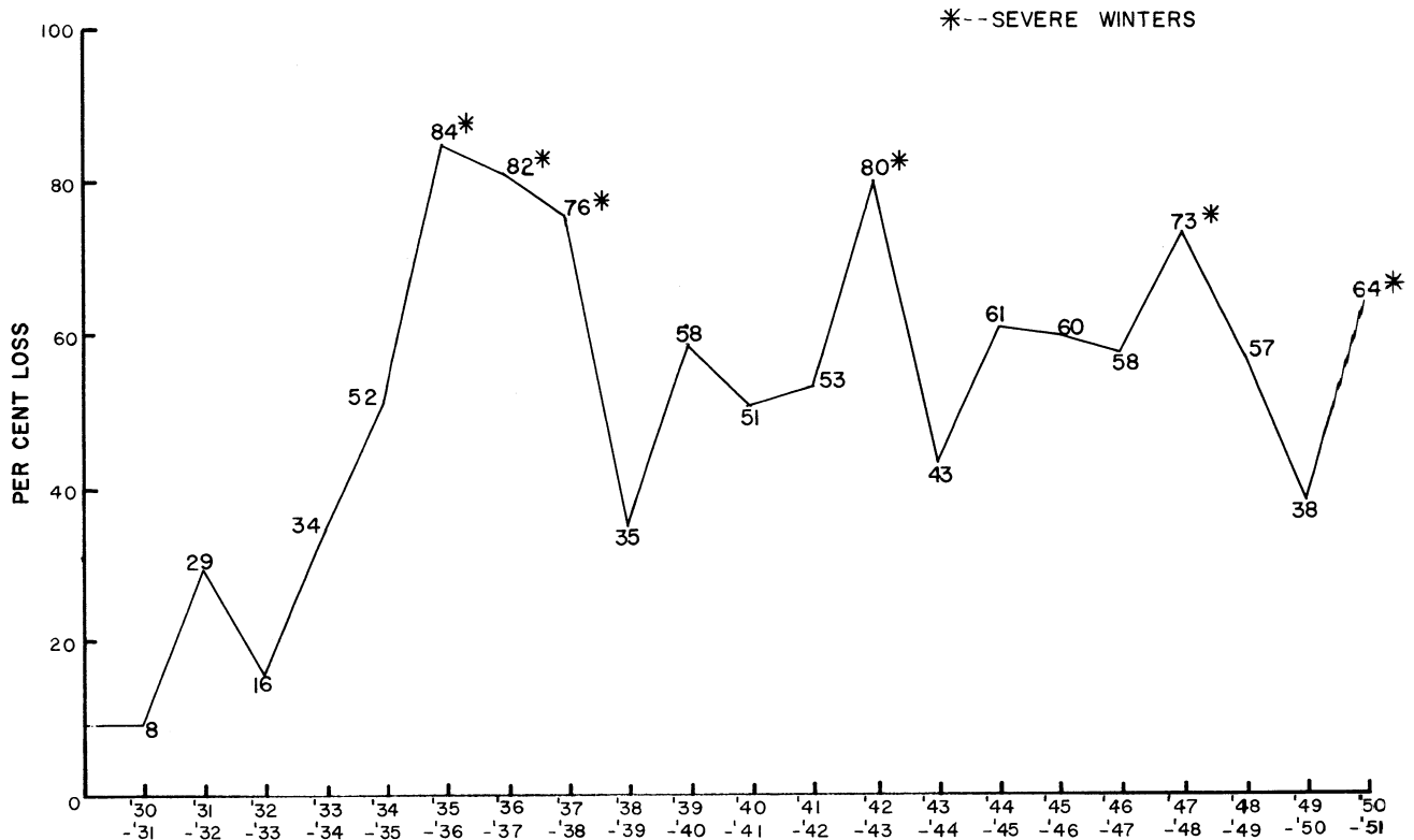
Figure 20. Annual winter loss (%) at Prairie du Sac showing the effects of severe winters, 1929-51.
