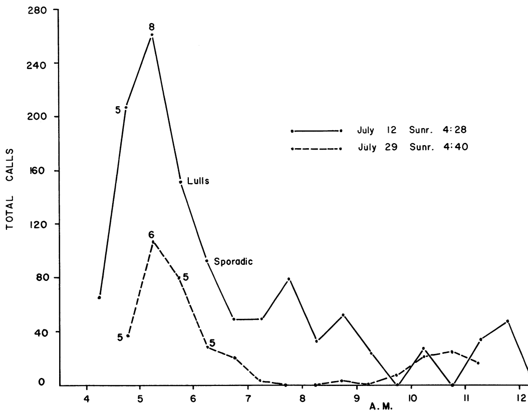
Figure 27. Daily pattern of whistling activity, morning hours, C.S.T., (1948). (5, 8, etc. are number of individual birds calling where known. Total calls per half-hour interval).
