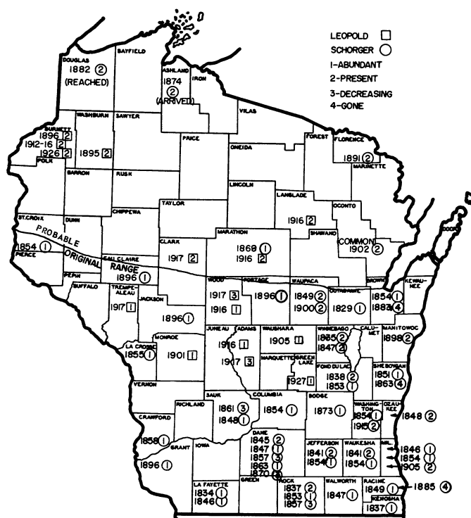
Figure 3. Wisconsin quail distribution and status based on early reports, 1834-1927.
