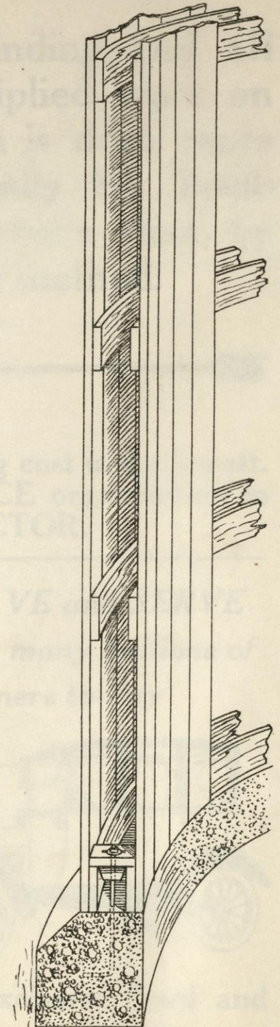
Showing the continuous Air Space Between the Walls
