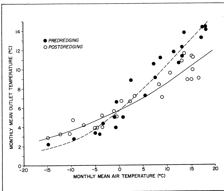
FIGURE 7. Monthly mean outlet temperatures and air temperatures at Sunshine Springs before (1968-69) and after (1970-72) dredging. Lines were fitted by curvilinear regression.
