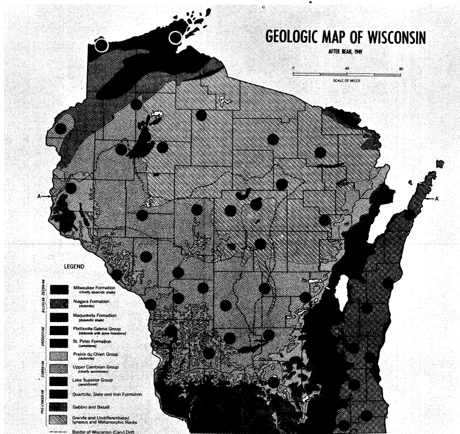
FIGURE 2. Location of groundwater supplies sampled in respect to geologic formations.
