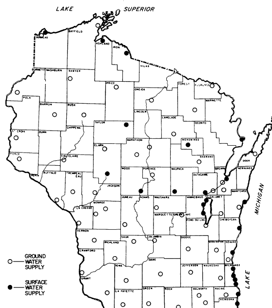
FIGURE 1. Sampling locations for trace element survey.
