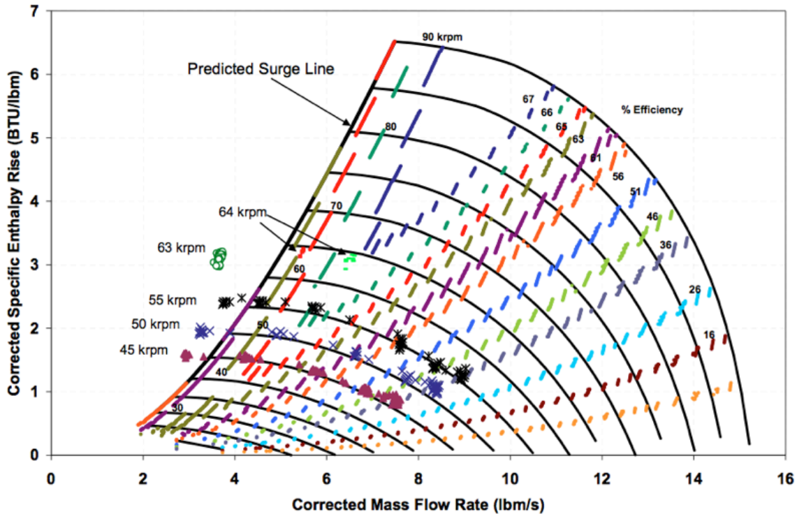
Figure 3.1. Performance map for the main compressor in the Sandia National Laboratory supercritical \text{CO}_2 test loop, taken from Wright et al. (2010). Note: the y-axis label should be “Corrected Specific Ideal Enthalpy Rise (BTU/lbm)”.
