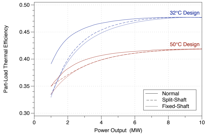
Figure 6.18. Part-load thermal efficiency of the three shaft configurations for the 32°C and 50°C designs.
