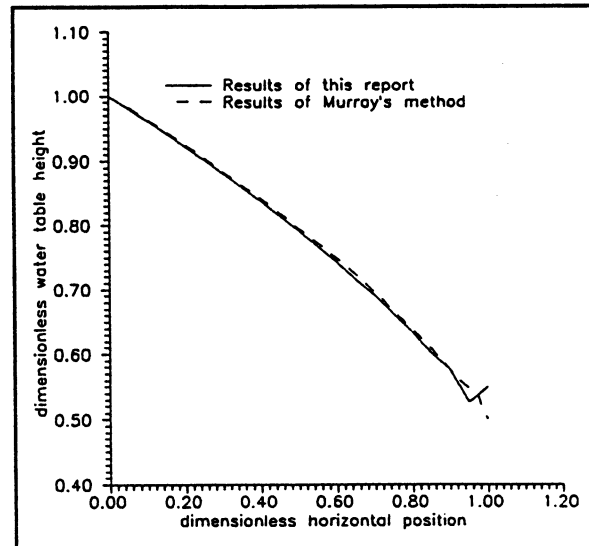
Figure 10. Comparison of phreatic surface water table from the method in this report and Murray's method when h_w/h_0 = 0.50 .
