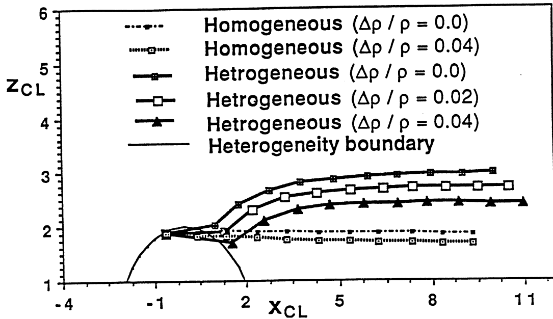
Figure 4. Effects of source buoyancy \Delta\rho/\rho on plume trajectory for initial slug case using variable buoyant plume density along the trajectory for (\zeta_o = 2.0, \epsilon = 10, x_i, y_i, z_i = 0.75, -0.25, 2.0) .
