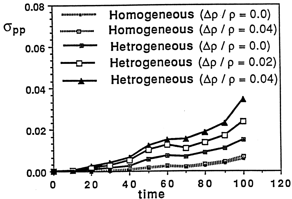
Figure 5. Effects of source buoyancy \Delta\rho/\rho on plume spreading for initial slug case using variable buoyant plume density along the trajectory for (\zeta_o = 2.0, \epsilon = 10, x_i, y_i, z_i = 0.75, -0.25, 2.0) .
