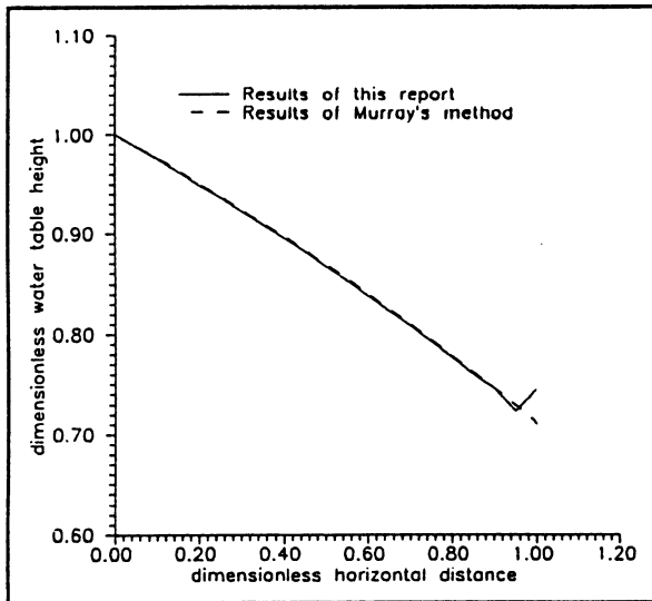
Figure 9. Comparison of phreatic surface water table from the method in this report and Murray's method when h_w/h_0 = 0.71 .
