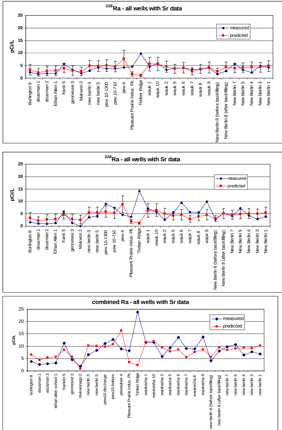
Figure 11: Match between predicted and measured radium levels in all wells with strontium data. The six rightmost New Berlin wells were used to establish the \text{Ra}^{2+}/\text{Sr}^{2+} ratio for use in Equation 1. Significance of error bars discussed in the text.
