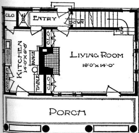
FIRST FLOOR PLAN OF COTTAGE.
