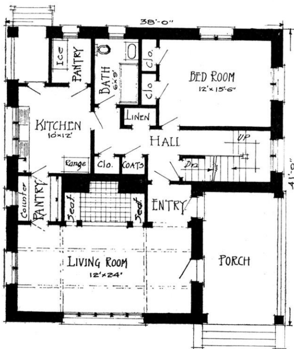
FIRST FLOOR PLAN OF CRAFTSMAN HOUSE NO. 220.
