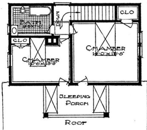
SECOND FLOOR PLAN OF COTTAGE.
