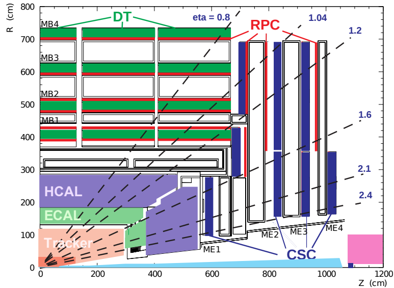
Figure 3.9: An rz cross section of the CMS muon system, demonstrating the \eta coverage and overlap of all constituent subsystems. [46]
