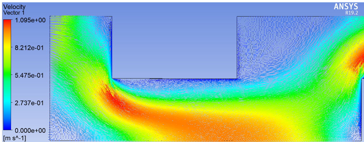
Figure 37: H_{\text{gap}} = 0.525 \text{ mm} , T_{\text{in}} = 300 \text{ K} , P = 2.6 \text{ MPa} , \dot{m} = 7.5 \text{ g/s} , resulting in Re = 145 .
