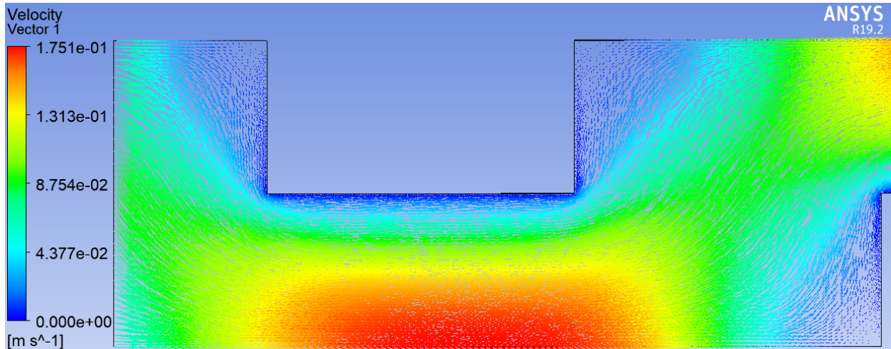
Figure 36: H_{\text{gap}} = 0.05 \text{ mm} , T_{\text{in}} = 300 \text{ K} , P = 2.6 \text{ MPa} , \dot{m} = 6 \text{ g/s} , resulting in Re = 2.4 , the lowest Reynolds number condition for the heat exchanger.
