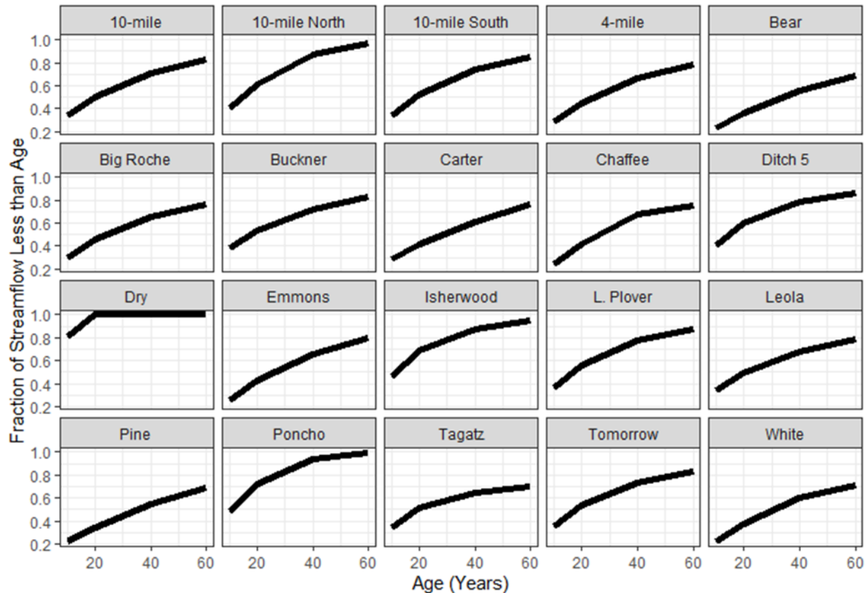
Figure 8. Streamflow age distribution for 20 sites monitored on the WCSP based on groundwater flow modeling.
