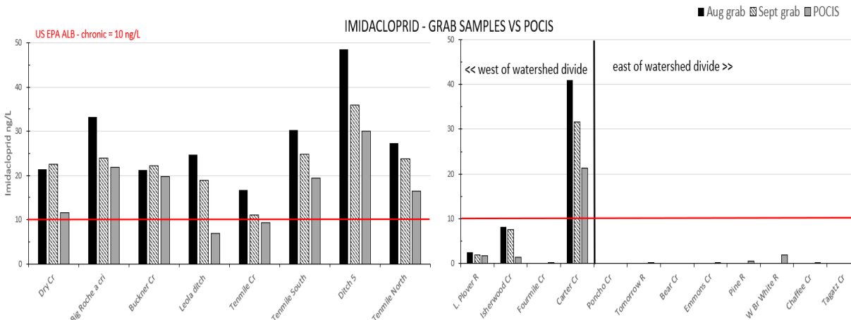
Figure 6. Traditional grab sample analysis and POCIS-derived concentrations of neonicotinoid insecticides.
