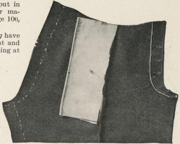
Fig. 318. Inside View of Pocket with Buttonhole Fly
