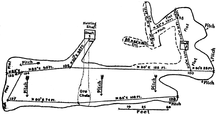
FIG. 6.—Map of the Enterprise mine. Rock walls of workings shown by full lines; filled walls of working by broken lines. Figures near crosses indicate approximate distances, in feet, from surface of the ground at top of hoisting shaft.
