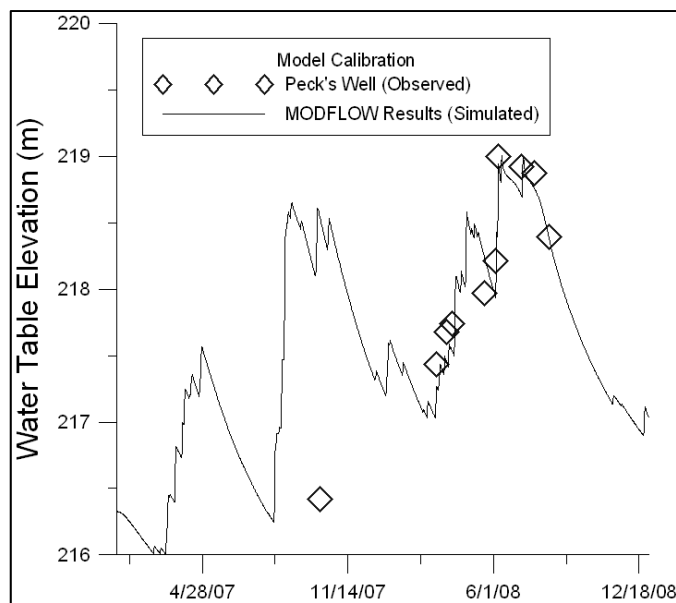
Figure 12. Observed and simulated water table elevation, 2007 – 2008. See Figure 1 for location of Peck's Well.
