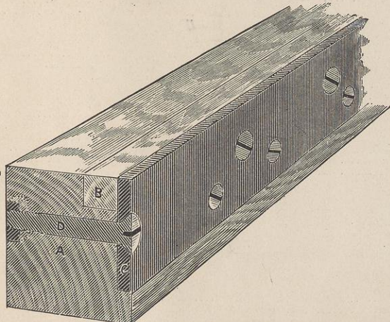
HAMILTON'S CUTTING STICK. For Paper Cutter.
