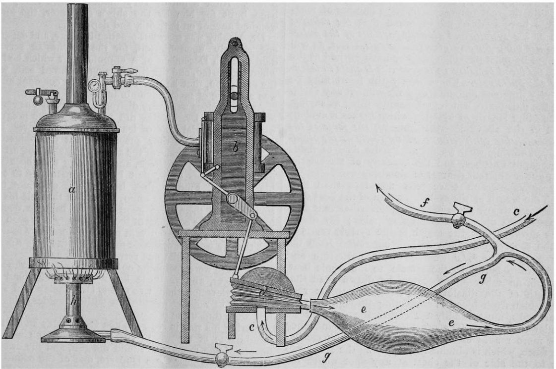
Automatically Working-engine, when supplied with coal-gas.
