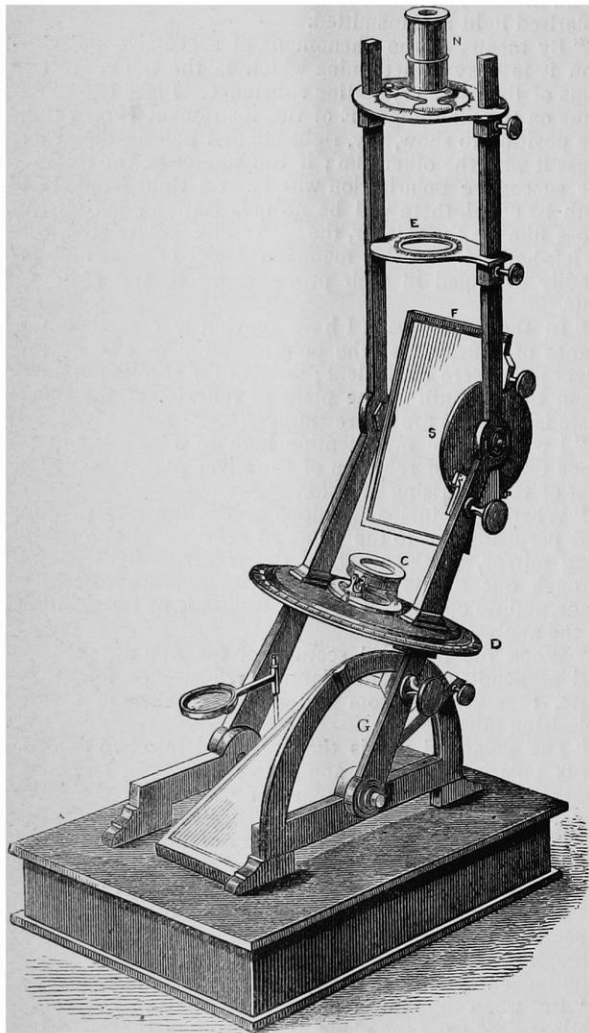
FIG. 15.—Wheatstone's modification of Norremberg's Polariscopes.
