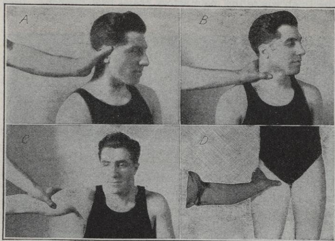
FIGURE 83.—Pressure points.
