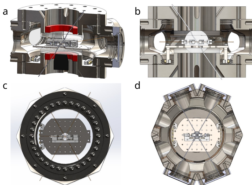
Figure E.7: The cavity node vacuum chamber and MInt Chip mounting system. The red sections in (a) represent quadrupole coils and the black object at the bottom represents a 0.4 NA custom objective, both of which are in the bore of a custom recessed objective.
