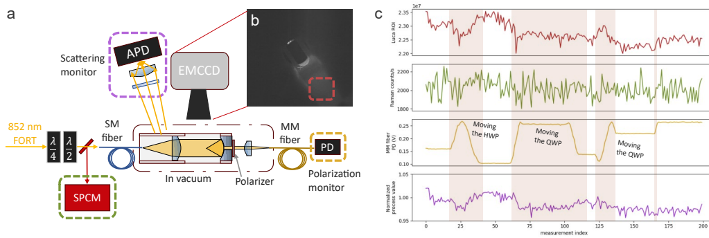
Figure 4.6: The feedback scheme for FORT dc intensity stabilization, shown schematically in (a). The inset (b) shows scattering from the FORT light on the Macor mirror tube in the chamber as viewed with an EMCCD. (c) Analysis of the extent to which the scattering monitored with the APD, which is used for dc stabilization of the FORT power, is dependent on polarization. The color of the data corresponds to the detectors outlined in the same color in (a).
