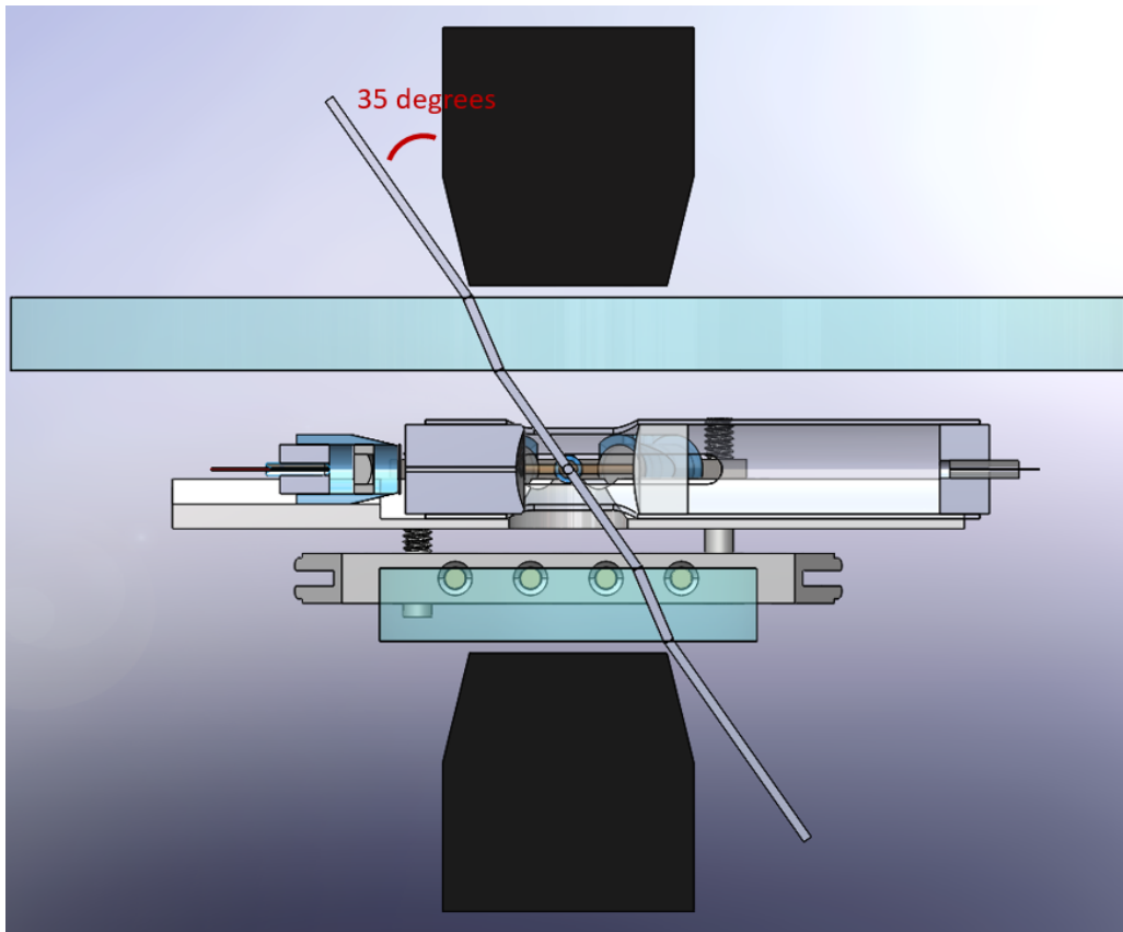
Figure 4.1: Cross section of the network node science chamber, with the steel chamber hidden, with two 0.4 NA JenOptik objectives represented in black. The cylindrical solids representing the MOT beam have radius equal to the 1/e^2 intensity waist w_0 , and there is \sim 2w_0 from the beam axis to the objectives at closest approach.
