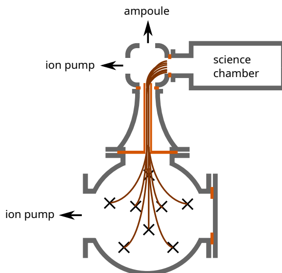
Figure 3.4: A cross-section illustration of the vacuum chamber design 1 showing the copper pinch off tube used as a differential pumping tube between the upper and lower vacuum chamber regions. The 8 fibers coming through the drilled Teflon plugged SwageLock feedthroughs (each feedthrough marked as a black X) go up through the copper tube and into the science region.
