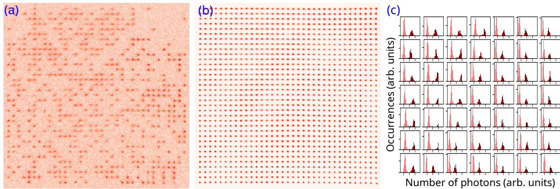
Figure 6.4: Single atom loading in a 1225-site array of dark traps formed with a broadband, spatially multimode laser. See section 6.3. (a) Single fluorescence image, showing stochastic loading of the trap array. The spacing between trap sites is about 3 \mu\text{m} . (b) Averaged fluorescence image processed with independent component analysis. (see Sec. 6.7.3). (c) Histograms of photocounts from regions of interests defined for the central 49 sites in (a), (b), showing the well-separated background (pink) and single atom (dark red) distributions.
