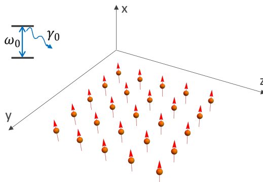
Figure H.2: A 2D grid of two-level atoms, or equivalently, classical electric dipoles.
