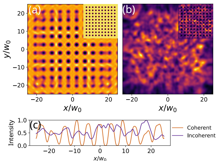
Figure 6.9: Comparison of simulated Talbot plane trap formation for a 10 by 10 dark aG array formed with (a) spatially coherent monochromatic light and (b) spectrally and spatially incoherent field. For the incoherent light, 21 frequency components spanning \Delta\lambda_{\text{FWHM}} = 3 \text{ nm} , each with 200 Hermite-Gaussian modes with random phases. The insets show the the focal plane intensity. The plot axes are scaled to the best fit Gaussian waist, w_0 = 0.943a(f_2/f_1) . (c) Line profile comparison of a row of traps from (a) and (b), showing the washed out Talbot interference for the multimode light. For both simulations, \lambda_0 = 825 \text{ nm} , d = 430 \mu\text{m} , and a = 100 \mu\text{m} , and a magnification of 1/100.
