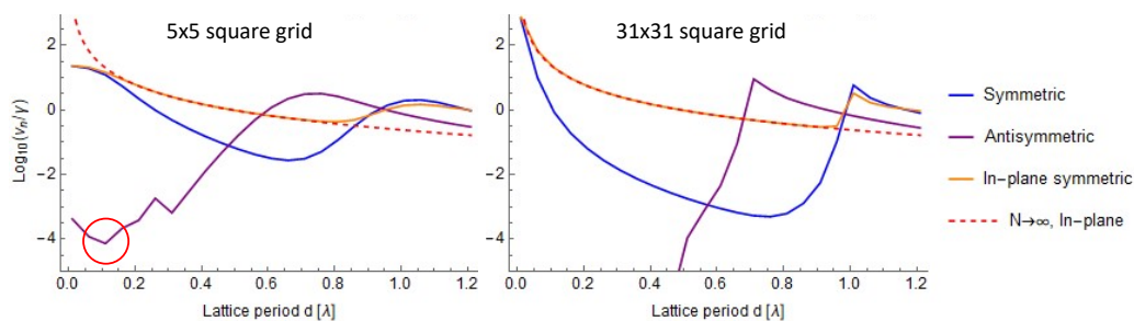
Figure H.4: Linewidths for various polarization orientations of atom arrays of two sizes. For the 31x31 array, the author has reproduced with his own code the results from Fig. (2) of [115] as a sanity check, and the obvious mimicry of plot styling is intentional for ease of comparison.
