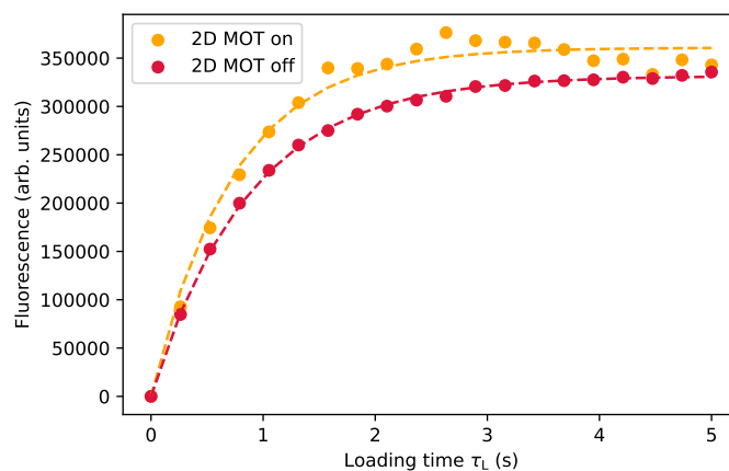
Figure 6.13: Loading curves for the Cs 3D MOT, with and without the 2D MOT on. In the latter case the 3D MOT is loaded directly from background. The fits to Eq. 6.21, where fluorescence is used as a proxy for N_s , give N_s, \tau_L = (360821.457, 0.727) and (331722.200, 0.872) . Fitting a line to these pairs gives \alpha/\beta = 5.076 \times 10^5 and \gamma_b = 0.397 \text{ s}^{-1} from which the pressures given in the text are obtained using Eq. 6.24.
