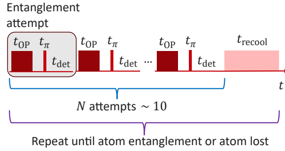
Figure 2.3: The remote entanglement generation loop.
