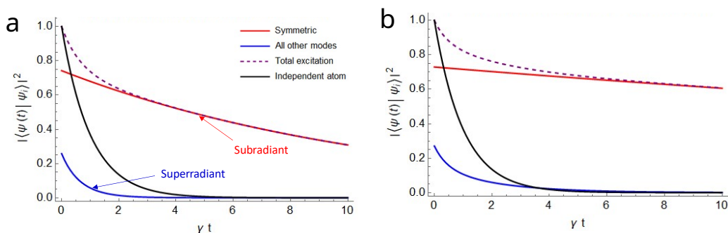
Figure H.5: Eigenmode composition of the excitation in the array versus time for an initial symmetric (a) and anti-symmetric excitation (b) of the 9 central atoms.
