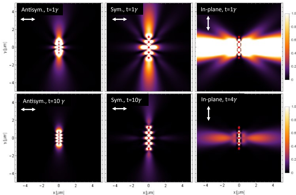
Figure H.6: Emission intensity patterns at different times for different polarization arrangements, where the central nine atoms share a single excitation at t = 0 , i.e., |c_i(t = 0)| = 1/3 in all cases. The inset double arrow denotes the polarization direction.
