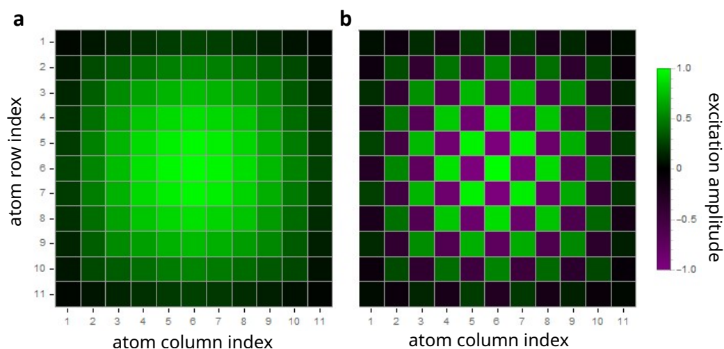
Figure H.3: Symmetric (a) and anti-symmetric (b) modes of an 11x11 square grid of atoms with out-of-plane polarization, found by sorting the eigenmodes by maximum overlap with the state of interest.
