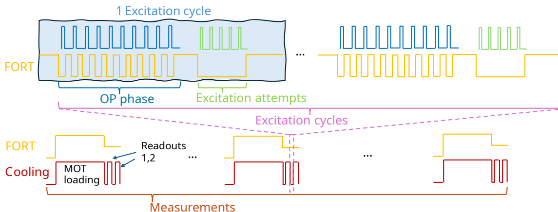
Figure 5.1: The experiment sequence loop for generating single photons, involving multiple sequences of chopped optical pumping (blue) and excitation attempts (green) per atom loaded. The nomenclature shown is used for consistency with what is used in the lab.
