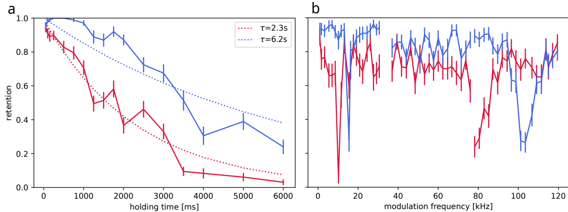
Figure 6.6: (a) Coherent trap lifetimes and (b) vibrational frequencies. The blue (red) curves in each corresponds to data from the same trap site in the array, and the error bars denote \pm 1 standard deviation for the measurements. The values reported in the text come from the red. Discrepancies between the frequencies and lifetimes are attributed to the difference in trap depth across the array, as a Gaussian intensity profile was used to illuminate a subset of only \sim 25 apertures on the array mask.
