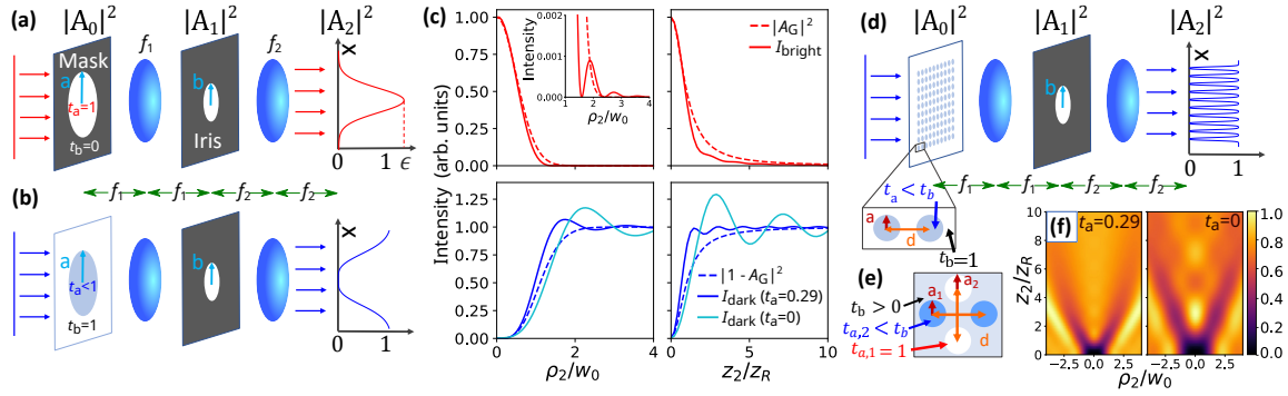
Figure 6.1: Working principle for creating approximately Gaussian (aG) field profiles using a 4f filtering scheme. (a) The design for producing a bright trap from an approximately Gaussian beam. An input plane wave is apertured by an opaque mask with a transmitting hole of radius a to create a top-hat profile. A spatial filter or iris of radius b in the Fourier plane transmits only the central lobe of the Airy disk. After transforming through lens f_2 , the output field, A_2 , is an approximately Gaussian (aG) beam. (b) Dark traps can be produced with a mask which is fully transmitting with a partially transmitting aperture, for which the output is the aG field subtracted from a plane wave. (c) Intensity profiles of bright (red) and dark (blue) traps based on aG beams (solid lines) compared to their Gaussian (dashed lines) counterparts plotted in terms of the Gaussian waist w_0 and Rayleigh range z_R = \pi w_0^2/\lambda for the Gaussian bright trap. The bright traps are normalized to their respective peak focal plane intensities and the dark traps are normalized to the asymptotic intensity at large \rho_2, z_2 . The inset shows a zoomed in view of the higher order deviation between the aG and Gaussian beam. The axial ( \rho_2 = 0 ) and radial ( z_2 = 0 ) profiles for the bright and dark aG trap are computed numerically using Fresnel diffraction theory. The pairs of dark and light solid blue curves have t_a = 0.287, t_a = 0 , respectively. For all aG beam curves, a = 100 \mu\text{m} and b = f_1 x_1^{(1)}/ak , except for the light blue ( t_a = 0 ) curve, which has b = f_1 x_1^{(0)}/ak . The other simulation parameters are \lambda = 825 \text{ nm} , and w_0 = 0.974(f_2/f_1)a and w_0 = 0.943(f_2/f_1)a for the bright and dark Gaussian beams, respectively. (d) Extension of the 4f filtering scheme to produce a 2D grid of dark traps, using a mask with a grid of apertures with spatial period d . (e) A dual grid of bright and dark traps with a single wavelength can be made with a mask which has finite background transmission t_b populated a grid of fully transmitting ( t_{a,1} = 1 ) apertures and a dual grid of apertures with transmission t_{a,2} < t_b . (f) Dark trap profiles in the \rho z plane corresponding to the blue and light blue solid curves in (c), normalized to their respective peak intensities.
