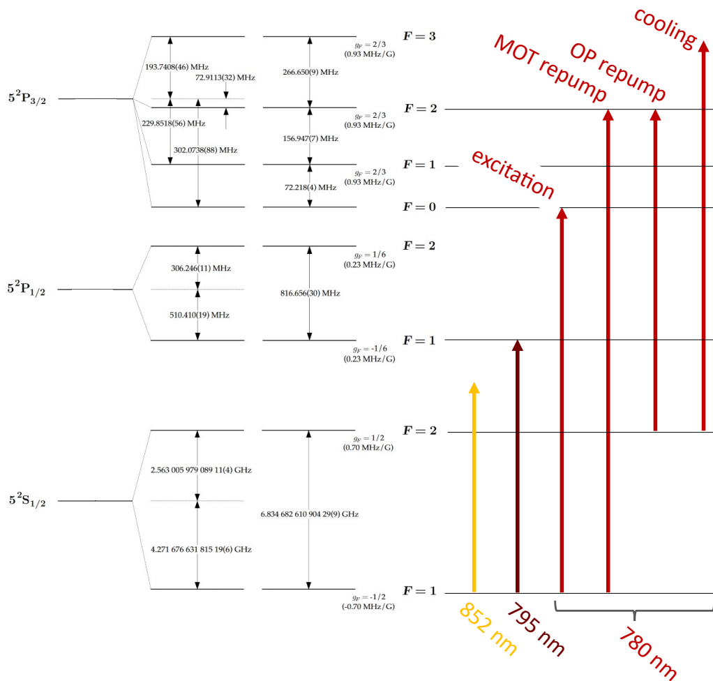
Figure 3.14: The different laser frequencies used in the quantum network experiment and their purposes, with ^{87}\text{Rb} energy levels adapted from [54].
