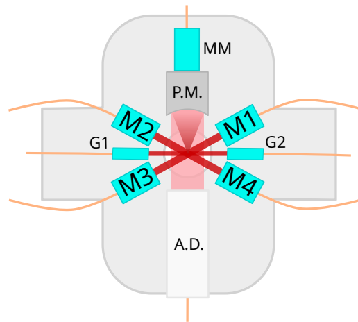
Figure 3.2: A simplified illustration of the layout of optical modules on the Macor bridge for the first version of the quantum network node. The modules M1-M4 (MOT 1 - MOT 4 in the text) produce the four MOT arms in a plane parallel to the bridge, G1 and G2 (GRIN 1 and GRIN 2 in the text) produce beams for optical pumping and excitation for Bell state preparation, P.M. is the parabolic mirror, and A.D. houses an achromatic doublet. In reality, A.D. and P.M. are a single optical module, but are shown separately here for clarity. MM couples light which passes through a central hole in the parabolic mirror and then a polarizer into a multimode fiber. Each module is interfaced with a polyamide coated optical fiber (orange lines), which allows coupling light from outside the vacuum system. See Sec. 3.2 for more details on the optical modules.
