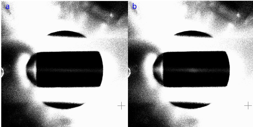
Figure 4.2: Alignment of the MOT6 beam, containing only cooling light, to an on-chip beam containing only MOT repump light. When the beams are overlapped and the cooling laser is locked as in (b) there is a clear enhancement of the fluorescence in the region of overlap, compared with the case in which the cooling laser is unlocked, shown in (a).
