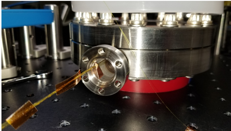
Figure 3.11: The optical fibers passing through the neck of the chamber were strain relieved by gluing a piece of the copper sheet to the chamber neck and gluing the fibers in turn to the copper. Note also the pieces of Kapton which can be seen securing the fiber bundle which is emerging from the chamber neck.
