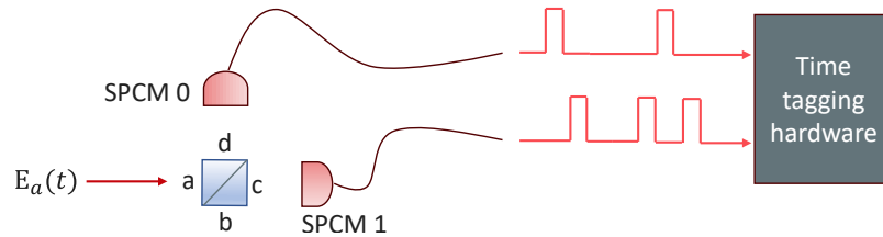
Figure 5.3: The optical setup for measuring g^{(2)} , where a vacuum state at port b is implied. The time tagging hardware is our Sinara hardware, where the TTL signals from the SPCMs are read in with DIO channels.
