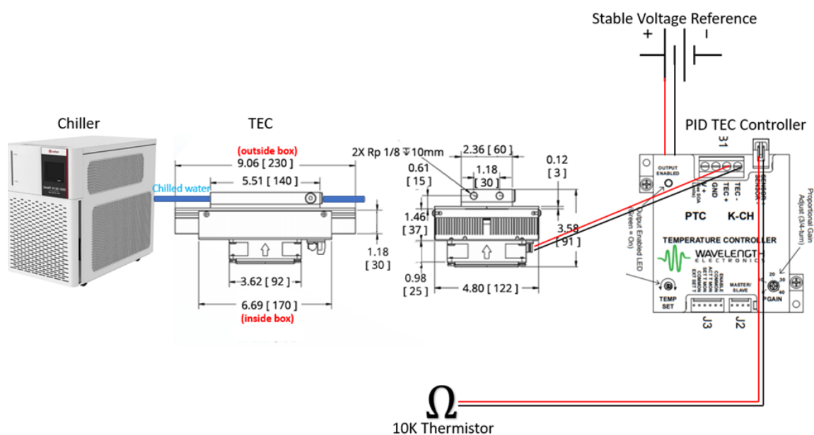
Figure C.1: Chiller, TEC, and TEC controller connections. Courtesy Arian Noori.
