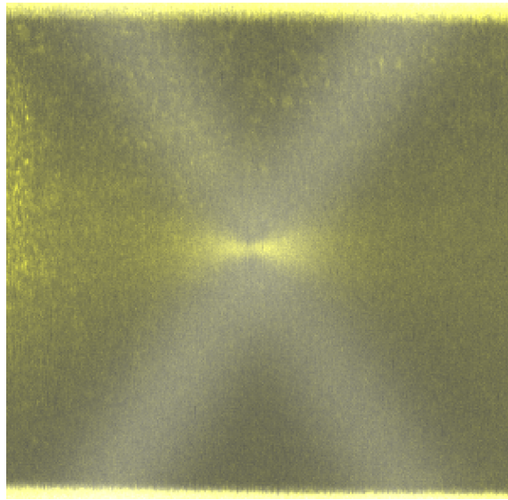
Figure 4.5: False-color image of the optical path of the FORT (yellow) and the on-chip MOT beams (grey) imaged with fluorescent emission from thermal Rb atoms in the chamber. The image is a combination of two separate images of the MOT beams and FORT path, both with 780 nm light, so that their pixel values could be scaled, clipped, and colored independently for optimal visualization.
