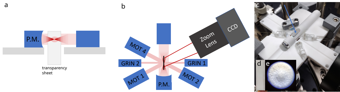
Figure 3.9: Schematic of the setup to image the optical chip beams as projected on a transparent scattering sheet made from an acetone-rinsed transparency sheet. (a) Cross-section of the optical chip from the side showing the transparency sheet in the path of the beam incident on and reflected by the mirror, and the projection of a MOT beam (light red oval). (b) View of the optical chip and transparency sheet from the top, showing the imaging path. (c) A photo of the optical chip showing the transparency sheet. Inset (d) shows the transparency sheet which appears matte white after the acetone rinse, and inset (e) shows its surface under an inexpensive microscope, captured with the author's phone's camera. The apparent bulge is due to optical aberration.
