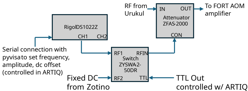
Figure 4.8: Setup for switching between static and modulated trap for the trap frequency measurement. RF to the FORT AOM is controlled with a voltage controlled attenuator (VCA). The VCA is controlled with a DC voltage for atom loading and readout or modulated with DC + AC from a Rigol function generator between readouts, as determined by a switch.
