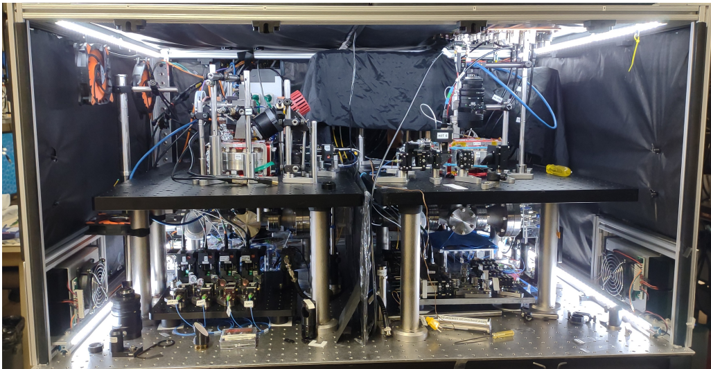
Figure 3.1: The two node quantum network apparatus in the lab, as of 2024.11.14. The left-side node is the one discussed in detail in this thesis. The two nodes are housed in a temperature-stabilized box (Appendix C), and the Bell state measurement optics live under the black sheet which can be seen in the back right.
