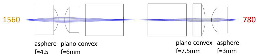
Figure E.3: Mode matching lenses for coupling a 1560 nm beam from a SM fiber into the cavity, and a cavity mode at 780 nm out of the cavity and into an SM fiber. The lenses are, from left to right, Edmund 83-580 , Edmund 67-447 , Edmund 89-014 , and Thorlabs 355660-B . Hyperlinks to products are available online.
