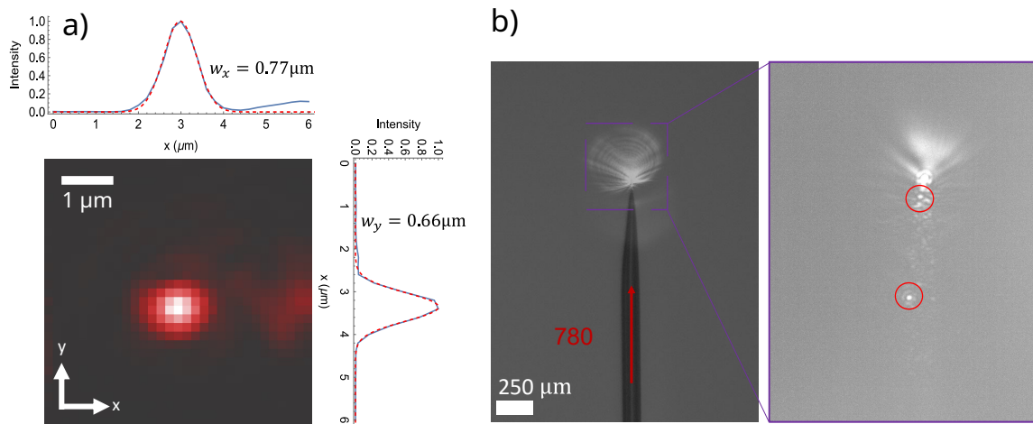
Figure 3.6: (a) The mirror focal intensity pattern as measured by coupling light from the mirror into a tapered fiber tip with a raster scan. Gaussian fits are shown for slices in x and y , where the fiber tip pointed along -y . The step size of the scan was 200 nm in each direction. The apparent aberrations on the beam are due to coupling into defects in the fiber tip, shown in (b). By coupling light into the non-tip end of the fiber, we can see that the emission, and hence collection, mode shape is not truly point like. The left and right images show the fiber with lower and higher exposure and zoom, respectively, to make clear the structure of the tip mode (left) and the weaker defect modes (right).
