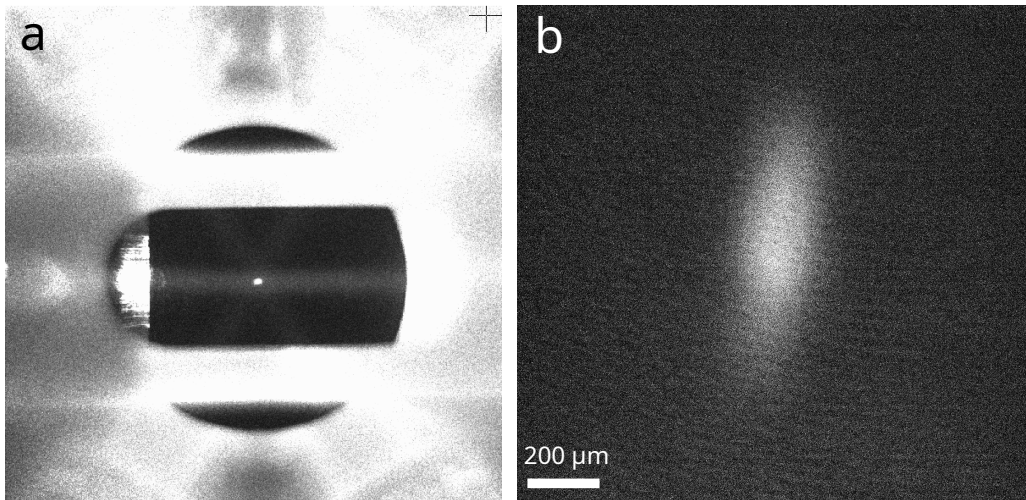
Figure 4.3: (a) A bright MOT captured with Andor Luca, and (b) a more typical MOT as imaged through a custom 0.4 NA objective onto a CS165MU ThorCam.
