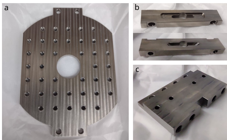
Figure E.6: (a) The titanium MInt Chip substrate and (b,c) cavity mounting hardware.
