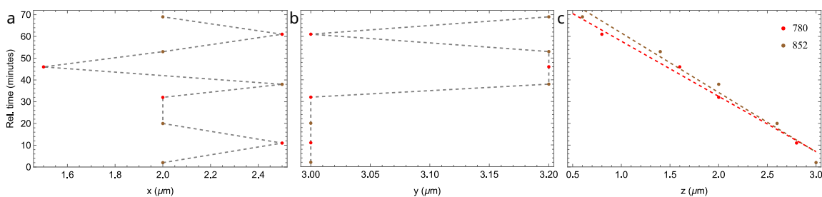
Figure 3.8: Tapered fiber scan measurement of chromatic shift between 852 and 780 nm light focused by the parabolic mirror. (a), (b), and (c) show the coordinate of the brightest pixel for a given 3D scan at either 780 (red points) or 852 (brown points), at x, y , and z , respectively. In the lab frame, gravity points along -\hat{z} , the fiber tip points along \hat{y} , and the detected beam propagates along \hat{x} . In each 3D scan, the step size is 200 nm in y and z (i.e. in the transverse planes), and 500 nm in the axial direction. The dashed lines in (a) and (b) are guides to eye, whereas the dashed lines in (c) are linear fits to the data for each wavelength.
