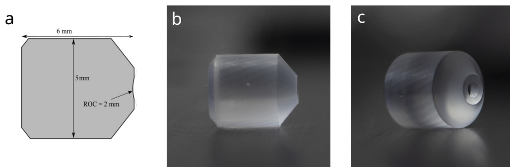
Figure E.1: The fused silica cavity mirror substrate design and photos of the final product from Optics Technology in Rochester, NY. The chamfered edges allow clearance for \sim 1 mm diameter MOT beams to be sent through the cavity. Design image and photos courtesy of Akbar Safari.
