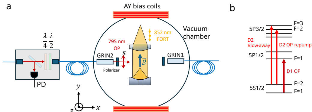
Figure 4.12: (a) The relevant components of the network node involved in optical pumping of the atoms and (b) the relevant energy levels, where only the hyperfine levels involved are labeled. PD is a TTI detector for monitoring pulse timing and power. Microwaves (not shown) for driving transitions between F = 1 and F = 2 states in the hyperfine ground manifold are polarized along y and propagate along -z . The OP repump (not shown) is sent through the same paths as the MOT beams (either 1-6 or just 5 and 6) and blow-away light is sent through the free space MOT 6 path. Note that although the D1 light is shown entering through GRIN2, we have more recently used GRIN1, for no particular reason, and may in the future alternate between the two during the optical pumping phase.
