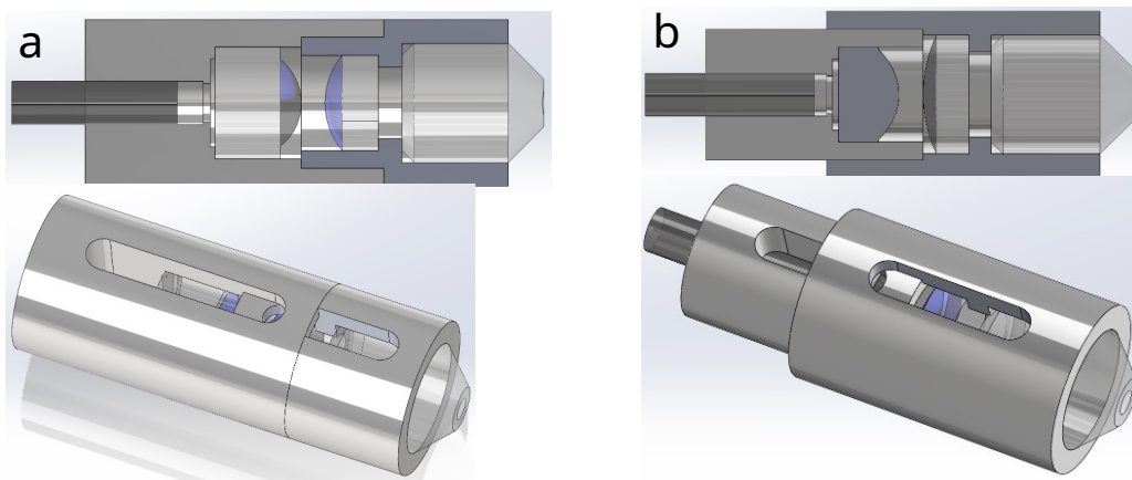
Figure E.4: Solidworks models of the housings designed to mount the fiber and cavity mode matching optics to the cavity mirrors for both the 780 nm photon collection side (b) and the 1560 nm locking side (a). The housings are designed to be Macor and are vented for use in vacuum. Note: the models shown were modified after the above images were made to include a chamfer on the cavity mirror end of each housing to match the cavity mirror's own chamfer, in order to not clip MOT beams. This update can be seen in Fig. E.5.
