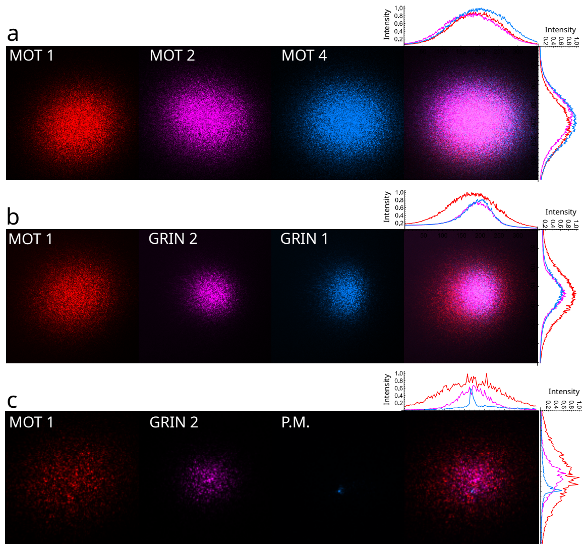
Figure 3.10: Optical chip beam projections on an acetone-rinsed transparency sheet. A setup of the imaging schematic is given in Fig. 3.9. The three panels (a)-(c) show different combinations of beam images, where the right-most image in each row is a combined image from the three individual beam images. The curves on the top and right sides are the sums of the rows and columns, respectively, for the individual beams. The "P.M." image in (c) shows the focus of the parabolic mirror.
