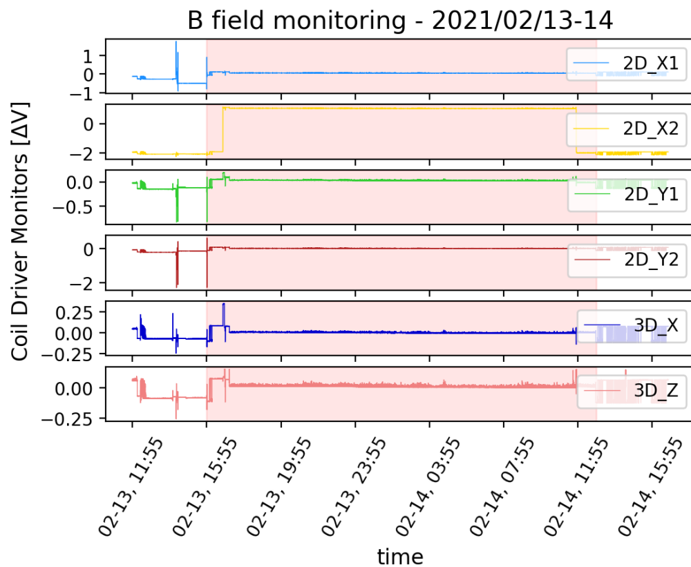
Figure A.2: Coil driver current monitor outputs, for selected 2D and 3D MOT coils measured with an NI DAQ analog input card and logged using the GOOD Logger. The shaded red region is where experiments are not being run, which shows that abrupt changes occur in the coil values came about without influence by the experimenters.
