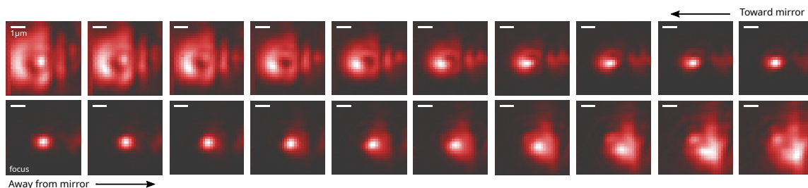
Figure 3.7: Transverse slices of the dipole trap beam taken at several axial positions about the focus. Each pixel is 200 nm and the longitudinal position varies by 0.5 \mu\text{m} between each slice. Note that each slice has been individually normalized for clarity. The scale bars indicate 1 \mu\text{m} .
