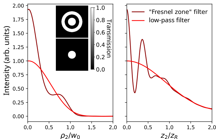
Figure 6.8: Comparison between an aG beam produced with a low-pass Fourier filter (see main text) and a modified version using a "Fresnel zone" Fourier filter. The horizontal axes are scaled to the best fit Gaussian waist w_0 and corresponding Rayleigh range z_R = \pi w_0^2/\lambda for the aG beam. The two Fourier filter variants are shown in the inset, and the radii of the transmitting rings and central aperture are given in the text.
