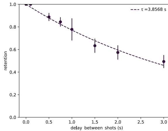
Figure 4.11: Single atom lifetime in the FORT. The dashed line is a fit to a decaying exponential with decay constant \tau .
