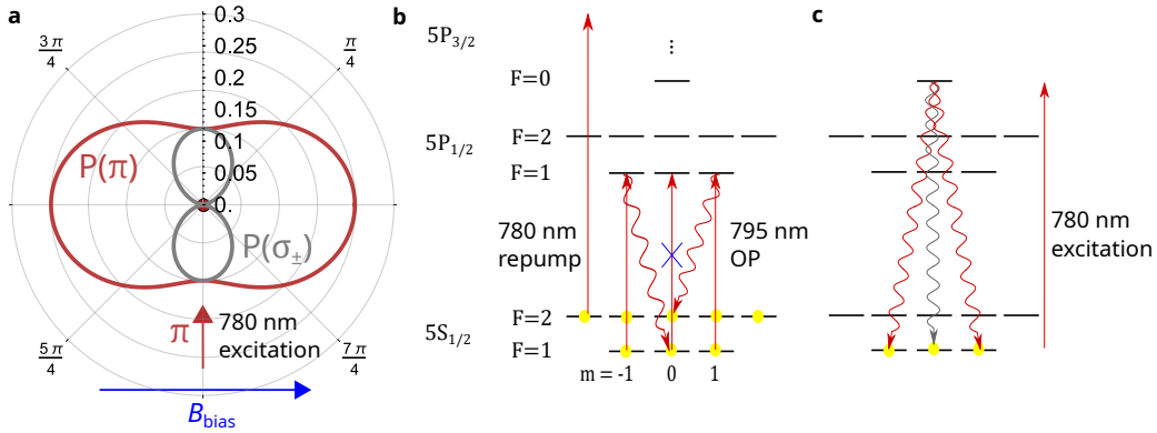
Figure 2.2: The atom-photon entanglement generation protocol. (a) The dipole emission pattern of the atom, oriented with the quantization axis defined by a magnetic field B_{\text{bias}} aligned to the optical axis of the photon collection optics. (b) The communication atom at each node is optically pumped into |5S_{1/2}, F = 1, m_F = 0\rangle , after which (c) the atom is excited with a \pi pulse to |5P_{1/2}, F = 0, m_F = 0\rangle , resulting in the creation of an atom-photon entangled state.
