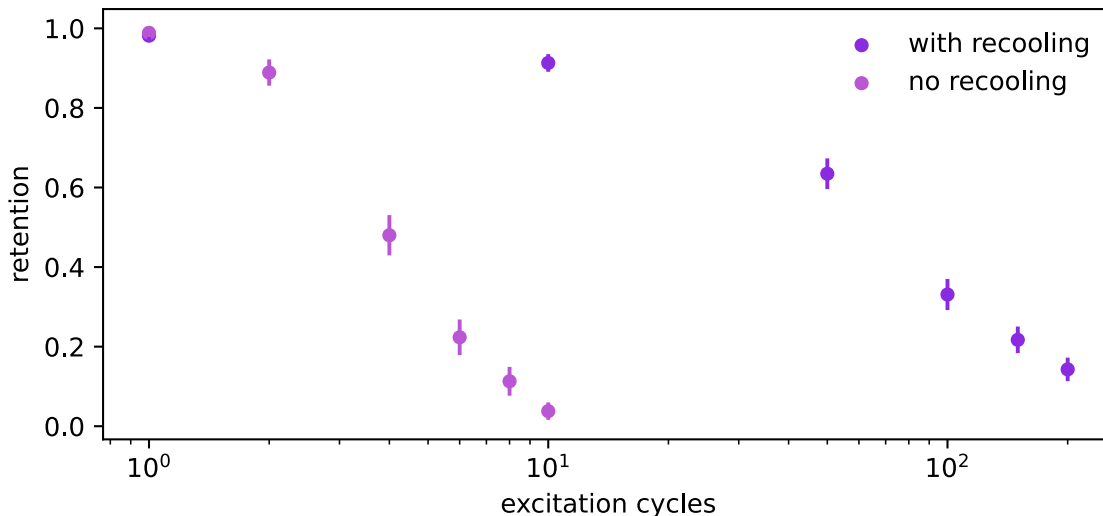
Figure 5.2: The probability an atom is retained following some number of excitation cycles with (a) and without (b) recoiling. For the data with recoiling, a 5 ms recoiling stage, consisting of turning on the MOT beams and using the readout shim coil settings, was appended to the end of each excitation cycle.
