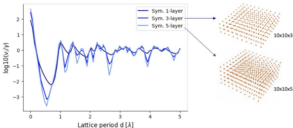
Figure H.9: The collective decay rate of the symmetric state for a 1-, 3- and 5-layer atomic volume with 10 \times 10 atoms in the layers.
