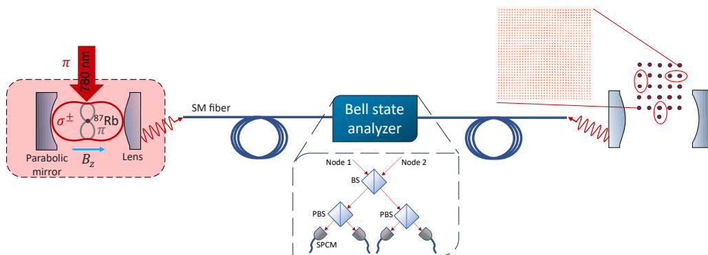
Figure 2.1: A rudimentary network of quantum registers as envisioned in this thesis. The red ellipses on the right-hand node represent Rydberg gates between the encircled qubits. The atomic array data inset is from Ch. 6.
