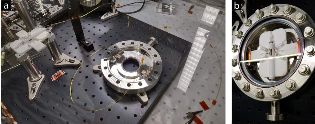
Figure 3.3: The custom two piece 6" flange-like vacuum chamber for one of the quantum network nodes. (a) The brain and spinal cord of the quantum node being strung through its head (optical chip, fibers, and bottom of the chamber, respectively). Note the Kimball Physics Groove Grabbers and copper shims used for mounting the so-called optical chip. (b) The optical chip in the chamber with the top window attached.
