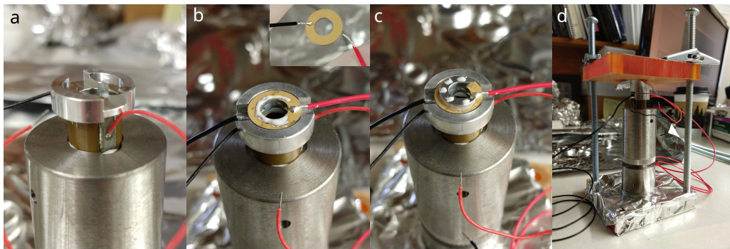
Figure G.1: Assembly stages of the two piezo stack for the filter cavity. (a) Fast piezo holder glued atop slow piezo, which is glued to the invar cavity spacer. (b) Fast piezo with soldered connections glued into its holder, with glue applied for the next spacer. (c) Spacer applied to fast piezo, which gives clearance for the positive electrode. (d) The assembly is glued using a makeshift clamp made with acrylic panels, which keep the components sufficiently parallel while the glue cures.
