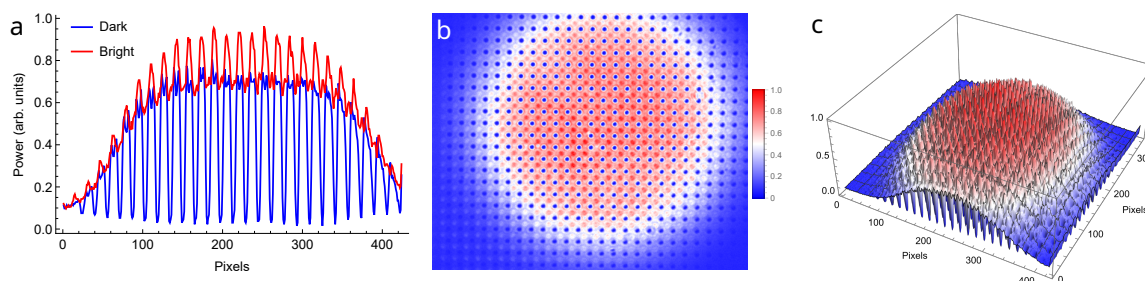
Figure 6.12: An intensity pattern formed by 808 nm incoherent light incident using a prototypical amplitude mask for creating bright and dark traps. The data is shown three ways, increasing in representation dimensionality from (a) to (c). (a) shows a single pixel row slice of dark traps and one of bright traps, where it can be seen that the depth of both trap kinds are with respect to approximately the same background intensity. The image was taken with the same optical setup used for producing the single-species traps described earlier. The amplitude mask was fabricated by Chengyu Fang of the Kats group in the UW-Madison ECE department.
