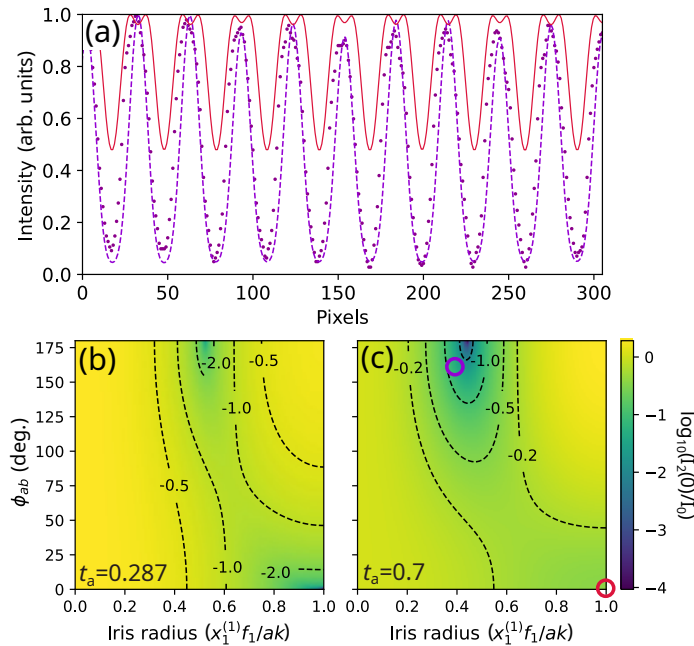
Figure 6.7: Numerical analysis of dark aG trap profile dependence on relative mask phase \phi_{ab} and Fourier filter (iris) radius. The iris radii here are given as dimensionless by dividing by the value used in the derivation in the main text, b = x_1^{(1)} f_1 / ak . (a) Trap profile data (purple points) from Fig. 6.3a compared to two Fresnel diffraction calculations: one with parameters which give a similar profile (purple dashes), and one with parameters corresponding to the expected trap given the specified parameters of the mask used (red line). Both parameter sets use f_1 = 500\text{mm}, f_2 = 50\text{mm}, \lambda = 805\text{nm} , with the former using (\phi_{ab}, \text{iris radius}) = (160^\circ, 0.4) , and (0^\circ, 1) for the latter. (b) and (c) show the dark trap center intensity (log scale) versus \phi_{ab} and iris radius. The choices of \phi_{ab} and iris radius used to generate the numerical curves in (a) are marked with rings of the same color in (c).
