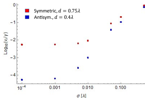
Figure H.7: The collective decay rate for an 11-by-11 array versus the standard deviation of an atom's position in the plane of array, given by a Monte Carlo simulation.
