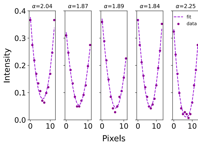
Figure 6.10: A row of adjacent trap site profiles from the data shown in Fig. 2, where each site has been fit to a form a\rho^\alpha + b . The data was clipped above the 1/e intensity to ensure fitting to the lower order portions of the traps. It is clear that the experimentally observed radial profiles are nearly quadratic, rather than the quartic profiles expected for t_a = 0.287t_b with zero relative mask phase.
