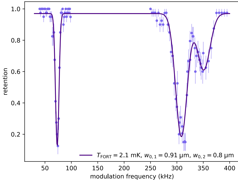
Figure 4.9: Vibrational spectroscopy of trapped atoms in the network experiment. The non-degenerate transverse resonances at high frequencies result from slightly different transverse waists in x and y . The two axial resonances at low frequency are not resolved, showing up as a single resonance. The error bars are 1/\sqrt{N} , with N the number of atoms loaded per data point. The solid line is a fit to a sum of three Gaussians.
