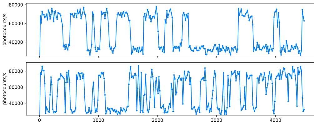
Figure 4.7: Photon count rate as atoms enter and leave the FORT with the MOT loaded continuously. The top subplot shows clearly the bimodal nature of the signal, indicating that we load either zero or one atom. The lower subplot shows atoms coming and going more frequently, corresponding to a higher atom loading rate. Note that although the vertical axis is given as counts per s, the data collected in the lab is counts, which is then divided by the exposure time for the SPCM here.
