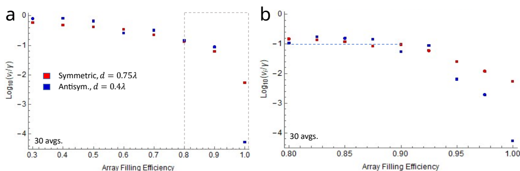
Figure H.8: The collective decay rate for an 11-by-11 array vs array filling fraction, given by a Monte Carlo simulation. (b) shows simulation results zoomed for more values of filling fraction over the range demarcated by the dashed box in (a). The dashed horizontal line in (b) is simply a guide to the eye.
