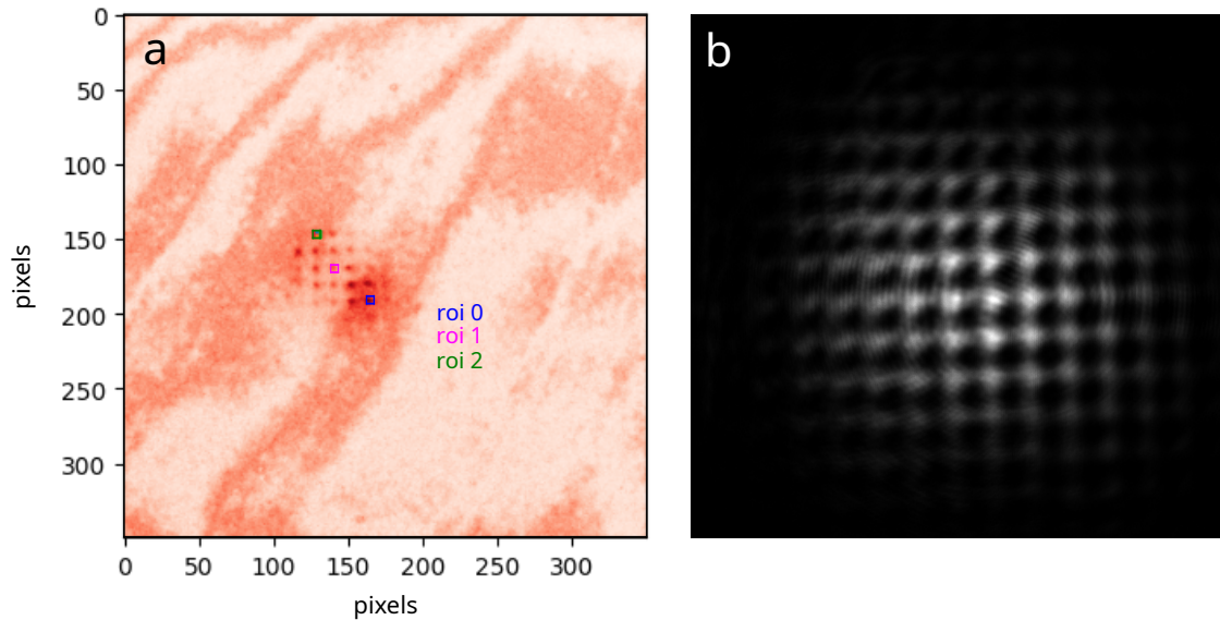
Figure 6.5: (a) Averaged image of trapped single cesium atoms in the coherent trap array and (b) an image of the corresponding trap intensity pattern in the intermediate imaging plane. The colored rectangles in (a) show the regions of interest (ROIs) used in experiments, where ROIs 0 and 1 are the sites used for the reported trap frequency and lifetime measurements. Fringes in (b) are from the camera sensor, and the wavy pattern in (a) is due to varying gain across the sensor array on the Hamamatsu camera used, attributed to the camera’s age.
