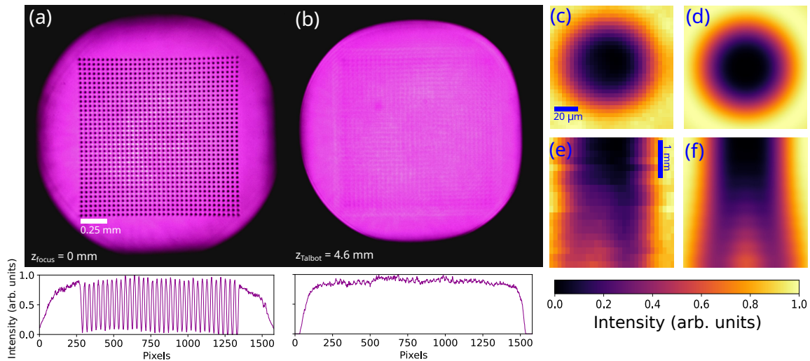
Figure 6.3: Dark trap intensity profile with broadband, spatially multimode light. (a) The focal plane of traps imaged onto a CCD, formed with a 4f filtering system with a magnification of 1/10 , giving an array period of 43 \mu\text{m} in the imaging plane. For the \lambda = 805 \text{ nm} light used, (b) the Talbot plane is located at z = 4.6 \text{ mm} , where the re-imaged traps have been strongly suppressed. (c) and (e) show a single trap site with 808 \text{ nm} multimode light projected on the focal plane and along the propagation plane intersecting \rho = 0 . For qualitative comparison, (d) and (f) show numerical simulations of the trap using coherent single mode light
