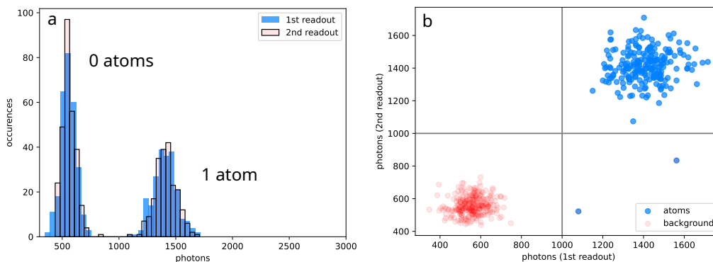
Figure 4.10: Single atom readout data for the two experiment readouts or “shots”. The same data is shown (a) as a histogram for each readout and (b) as a scatter plot, for a 14 ms exposure time and 3 ms holding time between shots. There is a clear absence of multi-atom loading events in (a), whereas the single atom loading fraction is 44% (b) shows that the fraction of atoms detected during the first shot which are also detected in the second, i.e. the retention fraction, is 99%.
