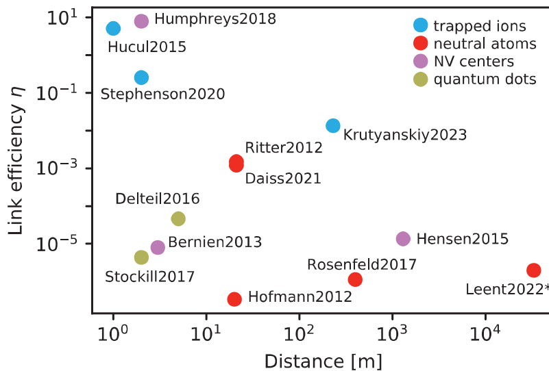
Figure 2.4: Link efficiency for rudimentary quantum networks vs the node separation across different platforms, reproduced from [32]
