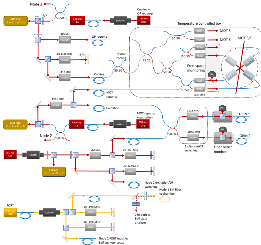
Figure 3.15: Schematic of the laser systems for the quantum network experiment. Each laser head supplies both nodes, but only the common paths and those for one node (arbitrarily chosen to represent Node 1). The Node 2 setups are mostly duplicates of those for Node 1 except for some minor component-level differences.
