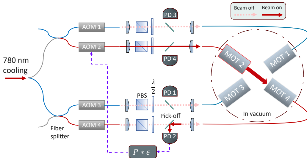
Figure 4.4: Schematic of the DC power stabilization for the on-chip MOT beams.
