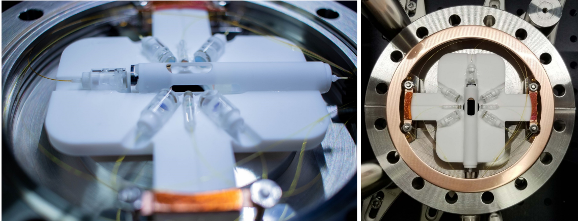
Figure 3.12: The finished optical chip in the science chamber, with the top of the chamber removed. In the right photo, note that the copper gasket has been cut to make clearance for the nuts which secure the bridge. Photo credit: Akbar Safari.
