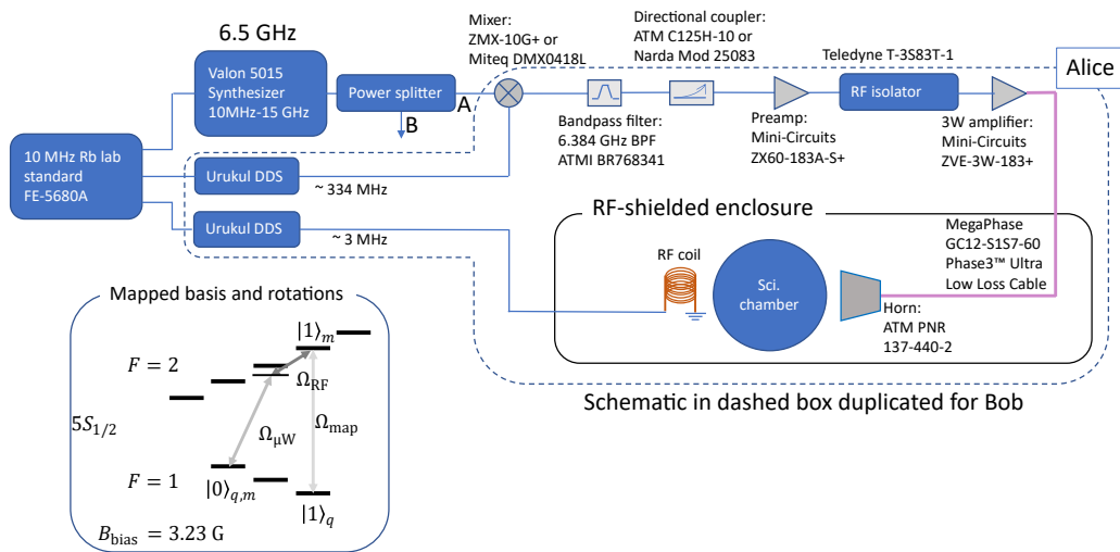
Figure 4.14: The microwave system used in the quantum network experiment and a (not yet implemented) RF line and coil planned to be used for two-photon rotations in the computational basis used for atom state tomography, as shown in the inset level diagram.
