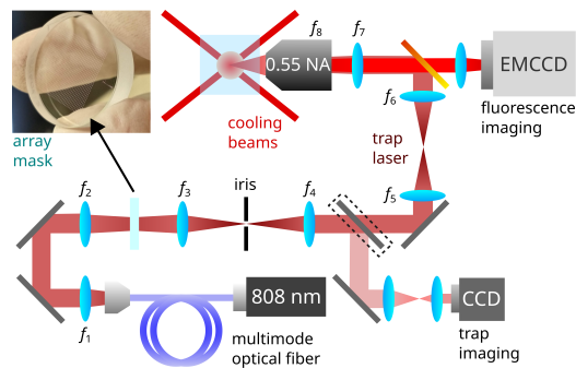
Figure 6.2: Schematic of the experimental apparatus for trapping laser-cooled cesium atoms in a dark trap array made with a broadband, spatially multimode 808 nm laser. Atoms are loaded into a magneto-optical trap (MOT), then transferred into a blue-detuned dark trap array which overlaps the MOT. The trap array pattern is formed using a passive optical mask and 4f filtering scheme, and the trap is imaged onto the atoms using a 0.55 NA custom objective. The dashed outline denotes a removable mirror which is used for imaging the trap at low power onto a CCD camera. An EMCCD camera captures 852 nm fluorescence from the atoms, which is collected through the same objective lens used for focusing the trap light and picked off with a long-pass dichroic. The labeled lenses have focal lengths f_{1-8} = (4.5, 500, 250, 75, 200, 30, 150, 22.8) mm.
