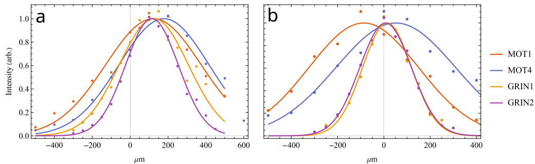
Figure 3.13: Fiber scans of MOT and GRIN beams with coordinates relative to the mirror focus location, taken after the air bake of the chip in the science chamber.
