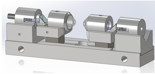
Figure E.5: Solidworks models of the assembled cavity with optional mirrors inserted between the fiber coupling and mode-matching optics housings on each side, to allow for free-space cavity coupling. The cavity length can be modulated using piezo-electric elements (dark gray). Note that the V-grooves on the left have small dimples to mark that they are 100\ \mu\text{m} shorter vertically, to allow for shimming to the correct height.
