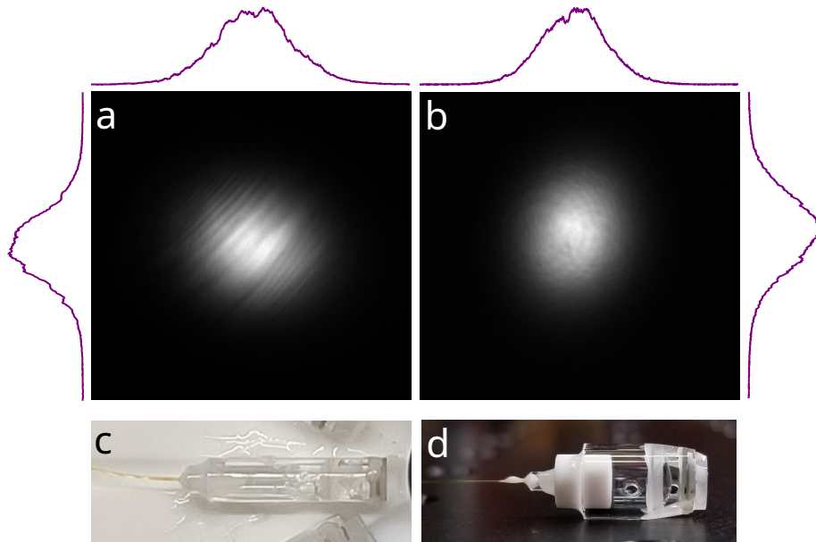
Figure 3.5: Photos of assembled optical modules and their resulting beam profiles. The beam profiles shown are from (a) GRIN 2 and (b) MOT 1. The purple curves are cross sections of the beams. A typical MOT and GRIN tube are shown in (c) and (d) respectively. Although the quality of the beam produced by the GRIN lens is much worse than that produced by a standard glass lens of uniform refractive index, because the atom will be confined to an area of order 1\mu\text{m}^2 , this aberrated beam profile is expected to be inconsequential.
