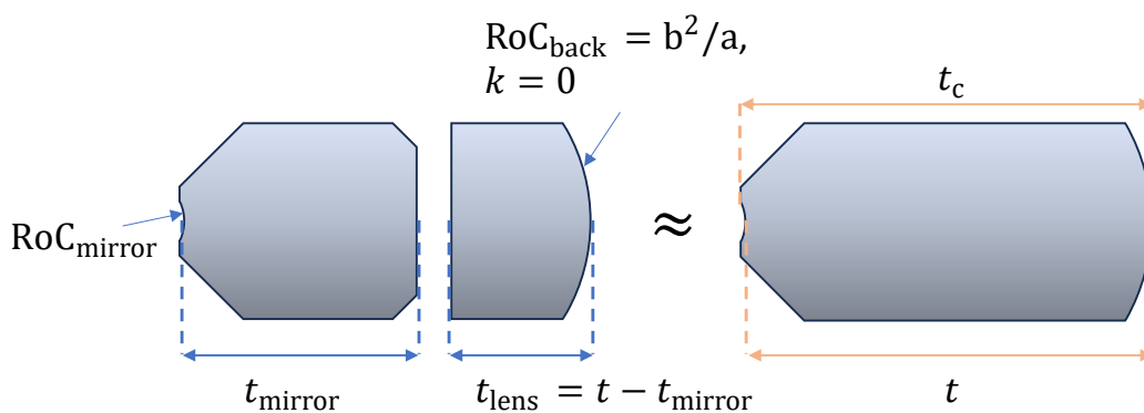
Figure E.2: A cavity mirror with an elliptical back surface (right) for transforming a spherical wave in the cavity to a plane wave outside the cavity can be approximated by a mirror with a flat back plus a plano-convex spherical lens (left). The spherical surface of the lens should have the same curvature constant as the elliptical surface. See text for details.
