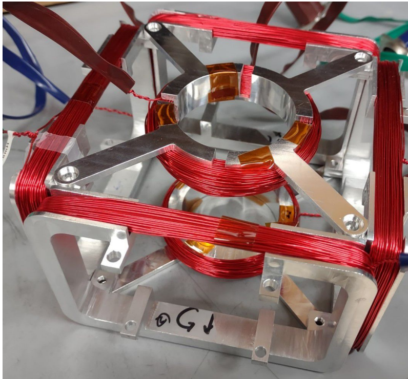
Figure 3.16: The coil assembly used for the first node in the quantum network experiment. A second version with minor modifications was made to give slightly deeper channels for the coils and notches to help start the winding. The circular coils can be driven in either an anti-Helmholtz or Helmholtz configuration to form a quadrupole field for the MOT or shim fields, respectively.
