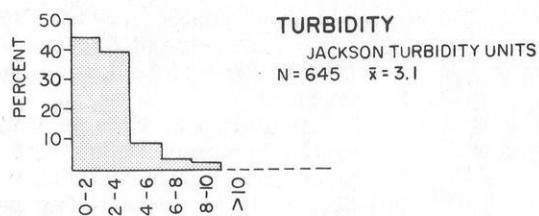
FIGURE 5. Selected limnological characteristics of Wisconsin lakes within the random data set. (More detailed data may be found in Figure 24.)
