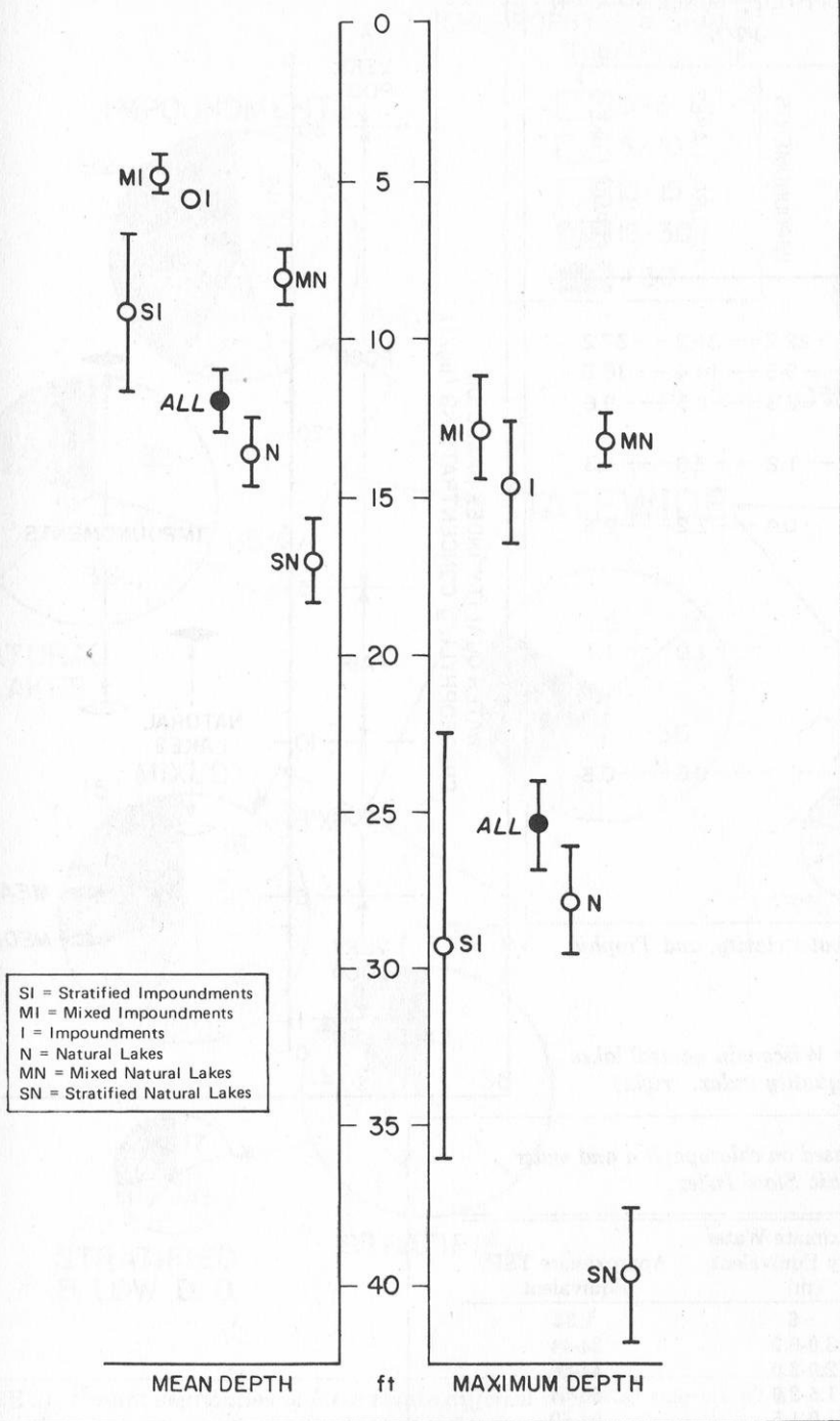
FIGURE 28. Comparisons of mean and maximum depths (means \pm 95% C.I.) for different types of lakes (random data set).
