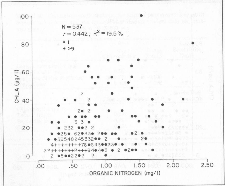
FIGURE 72. Relationship of chlorophyll a to summer organic nitrogen levels (natural lakes, random data set).
