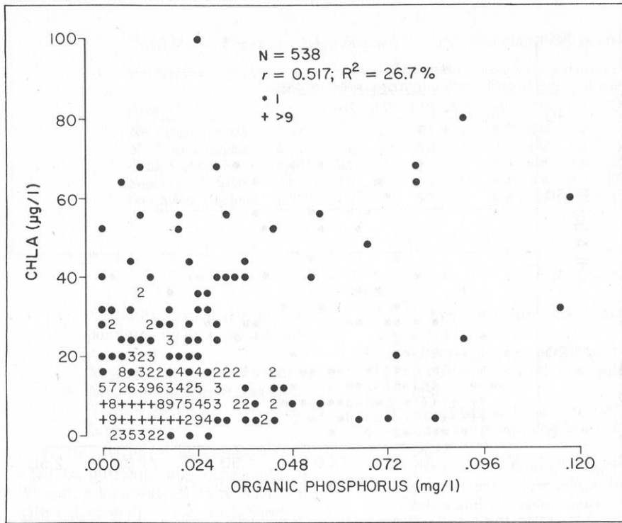
FIGURE 74. Relationship of chlorophyll a to organic phosphorus (natural lakes, random data set).
