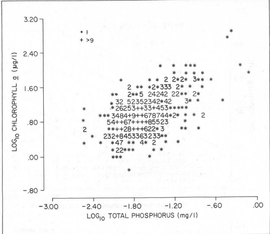
FIGURE 46. Relationship of Log-transformed chlorophyll a and total phosphorus data for 641 randomly sampled Wisconsin lakes.
