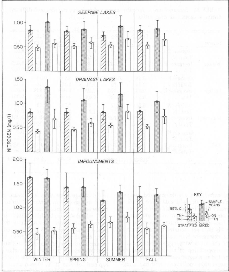
FIGURE 66. Seasonal means of total and organic nitrogen for different lake types.
