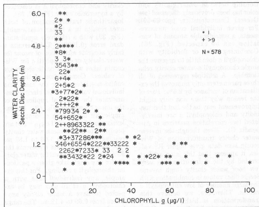
FIGURE 38. Relationship between water clarity and chlorophyll a concentrations (random data set).
