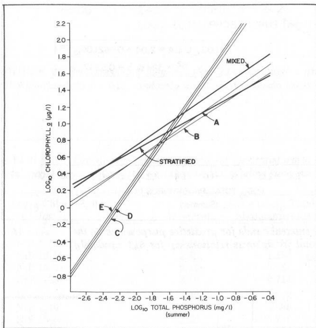
FIGURE 50. Relationship between chlorophyll a and total phosphorus for lakes with total phosphorus levels less or greater than 10 µg/l. (top left)
