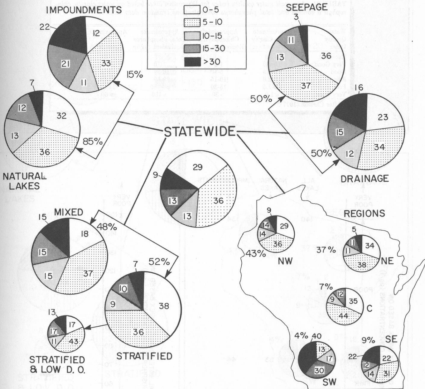
FIGURE 31. Percent distribution of lakes within different ranges of chlorophyll a concentrations separated on the basis of lake type and region.
