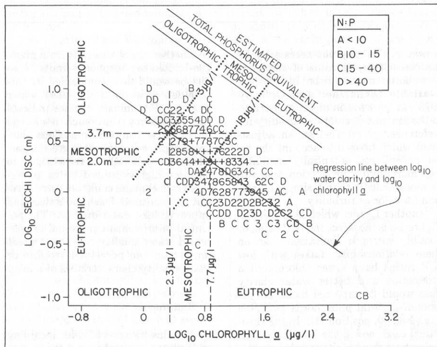
FIGURE 61. Trophic classification of 578 Wisconsin lakes based on water clarity, chlorophyll a, or total phosphorus concentrations (from data in Table 27 and linear regressions provided in Tables 23 and 25, representing all random data).
