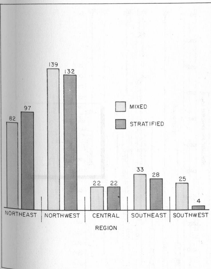
FIGURE 22. Distribution of mixed and stratified lakes by region (random data set).
