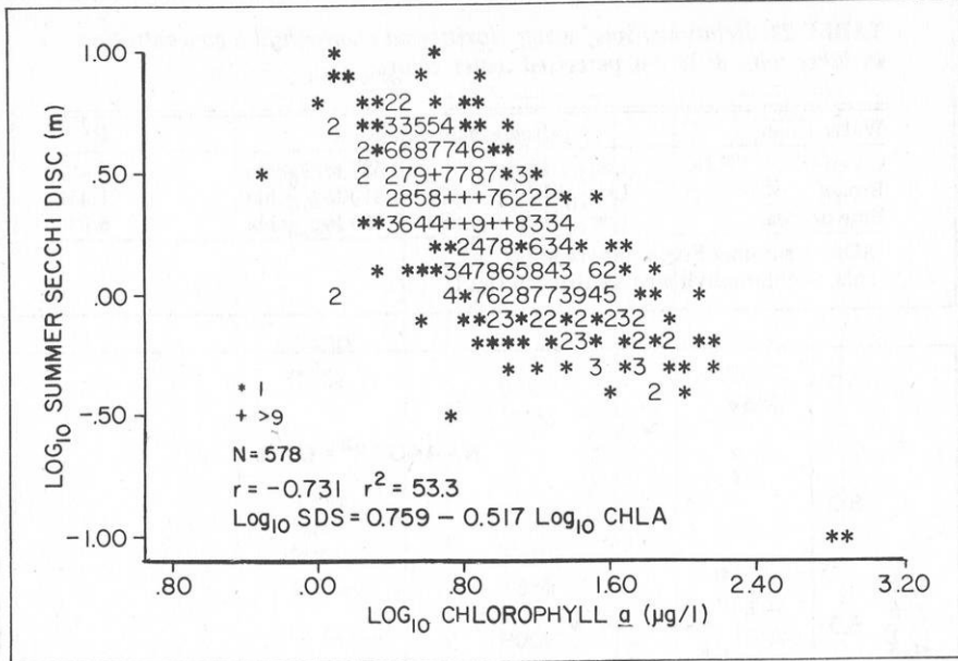
FIGURE 39. Water clarity and chlorophyll a relationship in Wisconsin lakes (Log-Log transformation).
