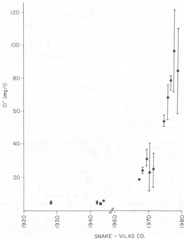
92 FIGURE 81. Historical trends in chloride concentrations in selected Wisconsin lakes.
