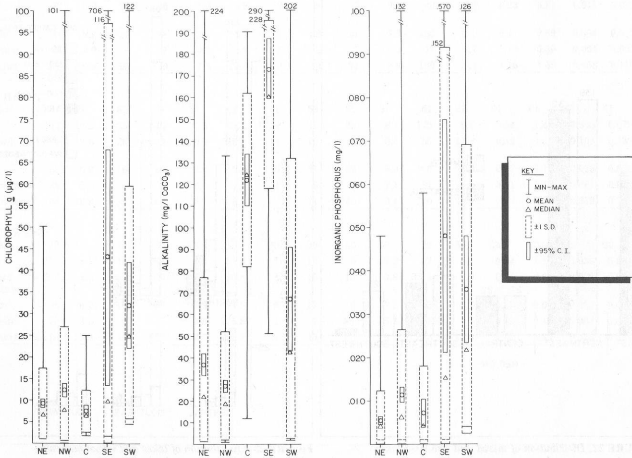
FIGURE 24. Characteristics of Wisconsin lakes by region (random data set).
