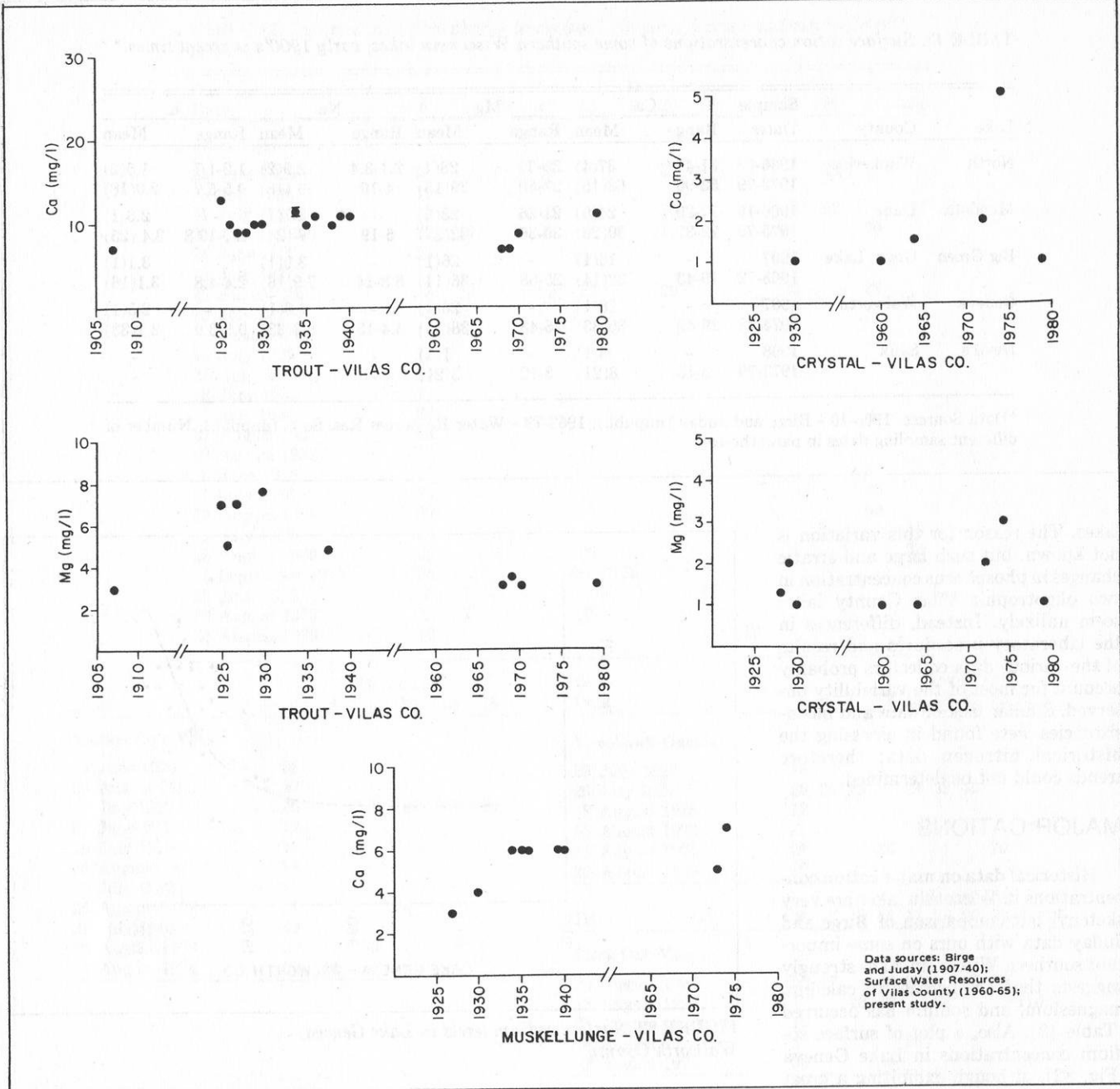
FIGURE 83. Surface calcium and magnesium concentrations in some Vilas County lakes.
