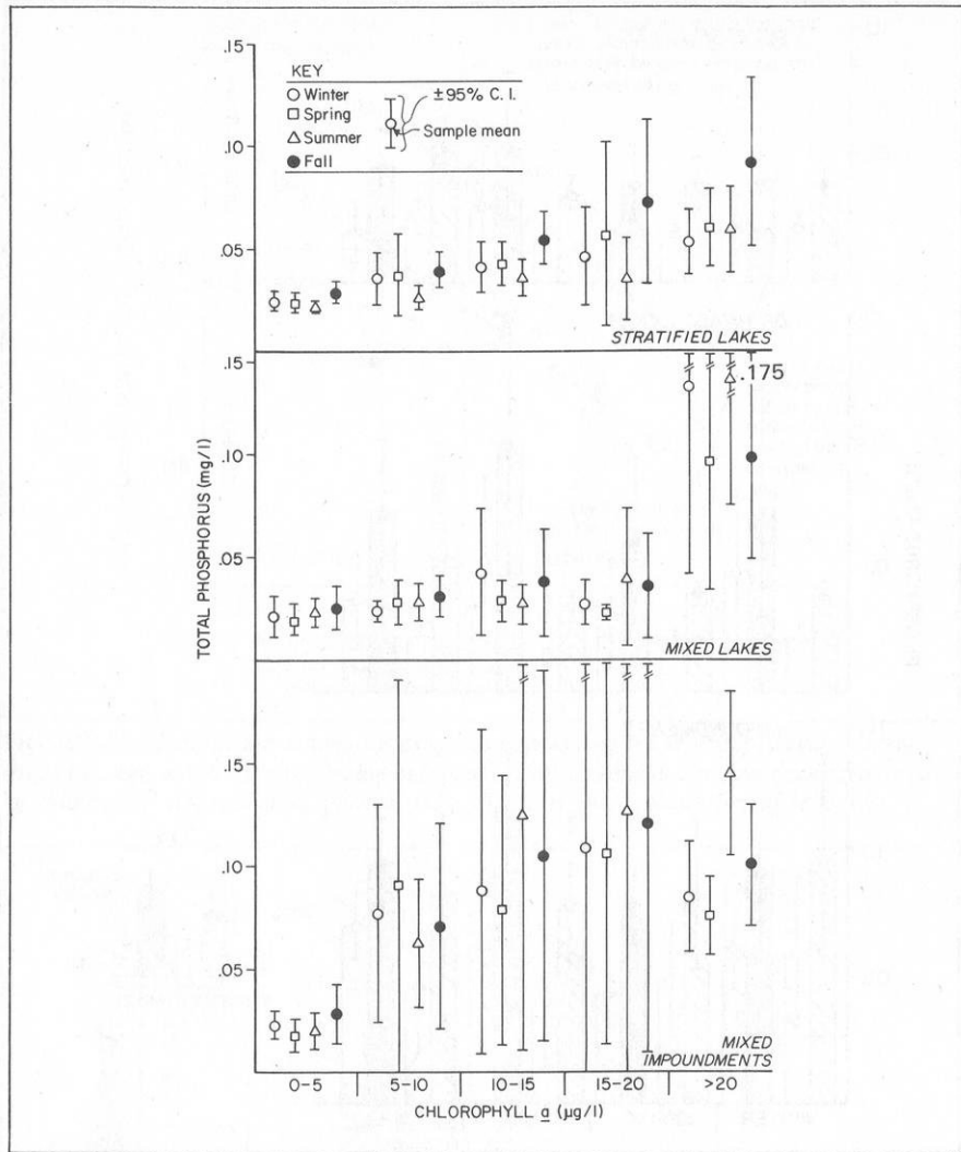
FIGURE 64. Seasonal changes in total phosphorus as related to lake type and chlorophyll a concentrations (quarterly data set).
