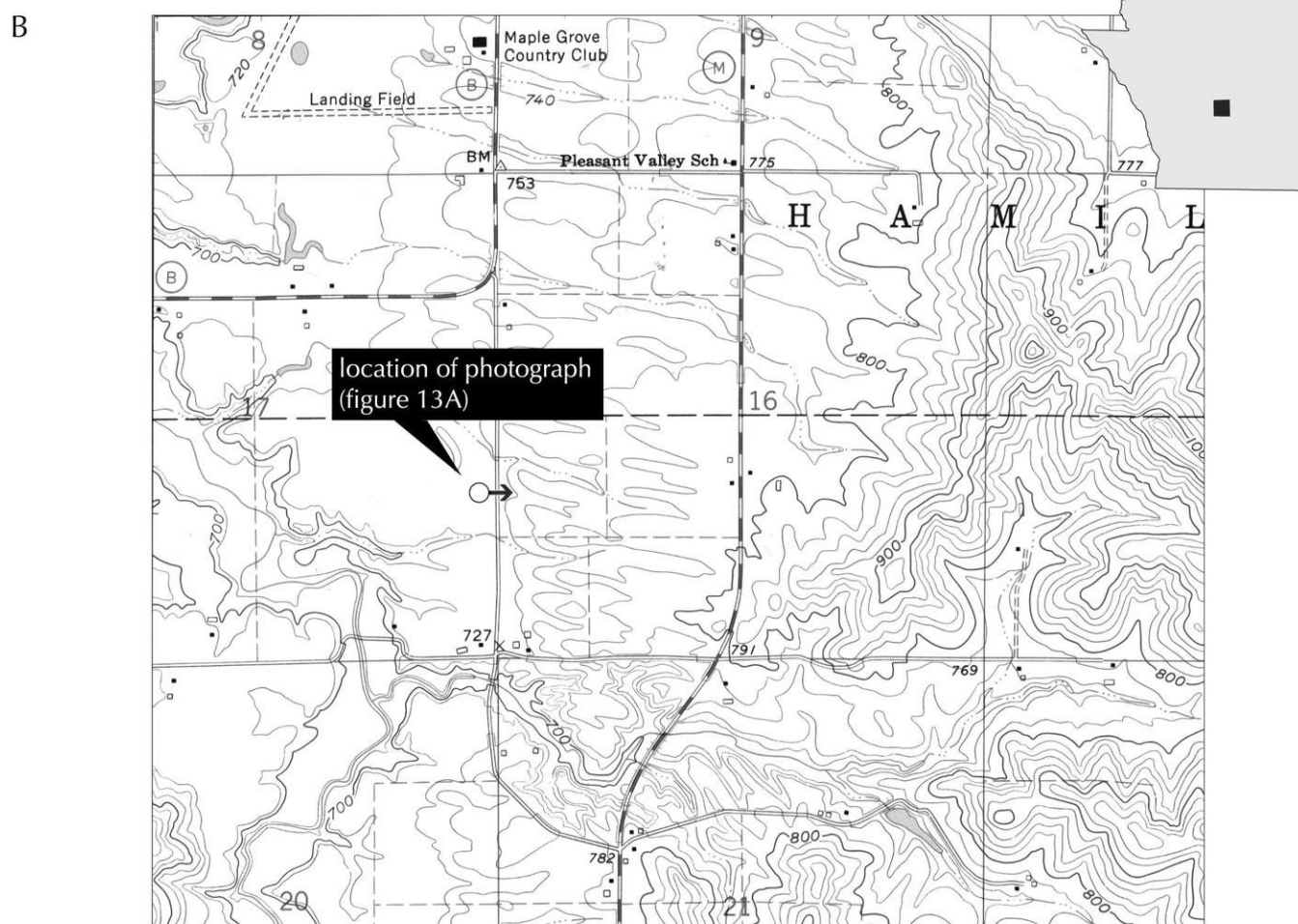
Figure 13. Panoramic view (A) and topographic expression (B) of paha landscape near West Salem east of County Highway B (SW \frac{1}{4} NW \frac{1}{4} SW \frac{1}{4} sec. 16, T16N, R6W) and is about 2 miles wide (U.S. Geological Survey, West Salem and St. Joseph, Wisconsin, quadrangles, 7.5-minute series, topographic, 1993 and 1974; contour interval is 20 ft).
