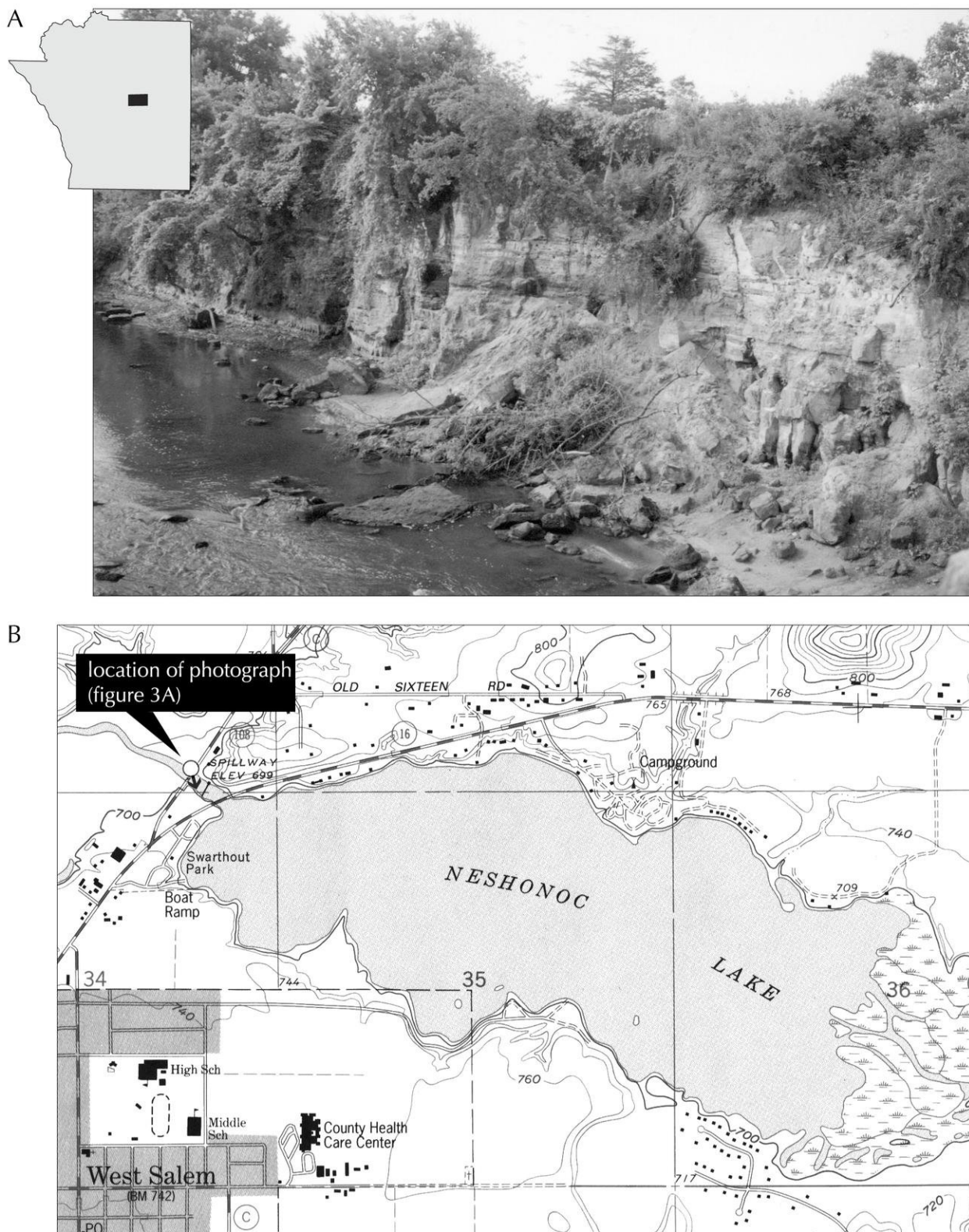
Figure 3. A. Exposure of Eau Claire Formation at Neshonoc Lake outlet near West Salem, taken from County Highway C looking southeast. B. Topographic map showing Neshonoc Lake and surrounding features. Area shown is 3 miles wide; contour interval is 20 ft. (U.S. Geological Survey, West Salem, Wisconsin, quadrangle; 7.5-minute series, topographic, 1993; contour interval is 20 ft).
