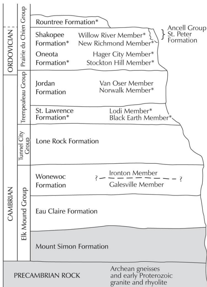
Figure 2. Lithostratigraphic units in La Crosse County. Asterisks indicate units recognized in the county, but not shown separately on plate 1; shading indicates units discussed in text, but not exposed at land surface.
