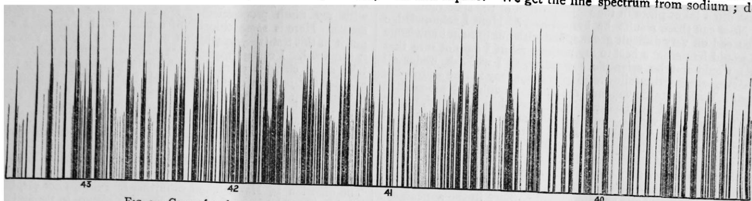
FIG. 3.—Copy of a photograph of the long and short lines of iron between wave-lengths 4,000 and 4,300.
