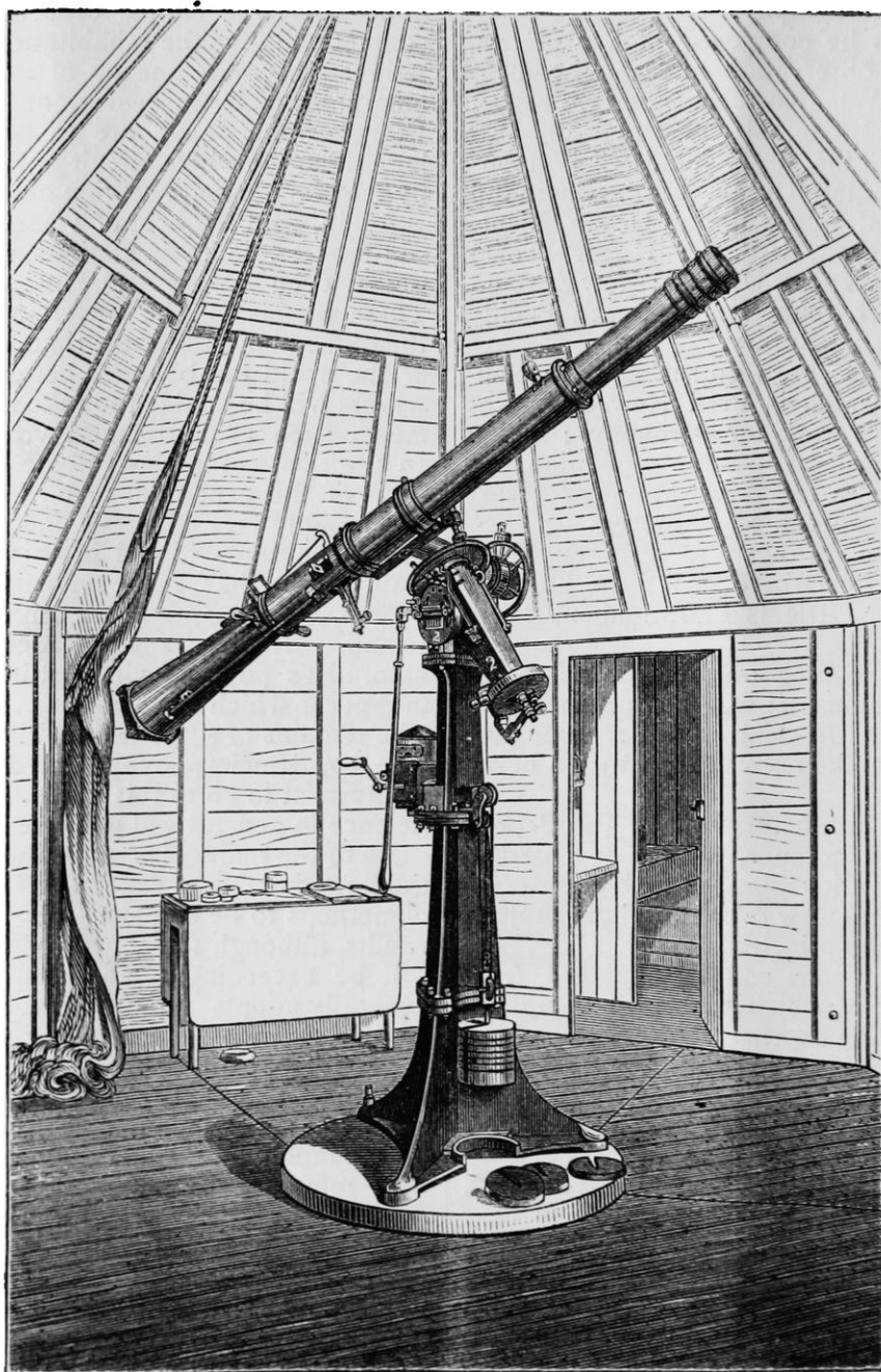
FIG. 19. — Photo-heliograph of the British Expeditions.
